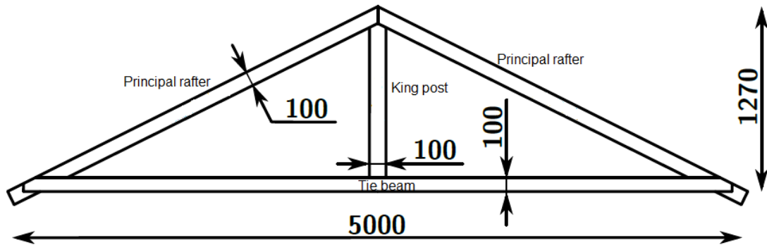
a) Roof king post truss dimensions
