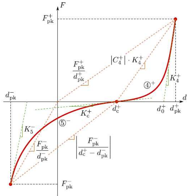
b) Definition of hysteresis loops
