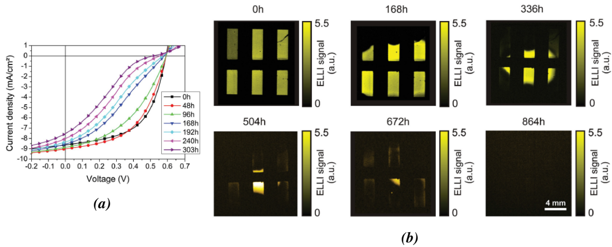
Figure 1.49: (a) J(V) curves of a glass-encapsulated inverted P3HT:PCBM 6-cells module along aging at 65 °C and 85% RH in the dark and (b) associated EL images of the same device. Reproduced from [216].
