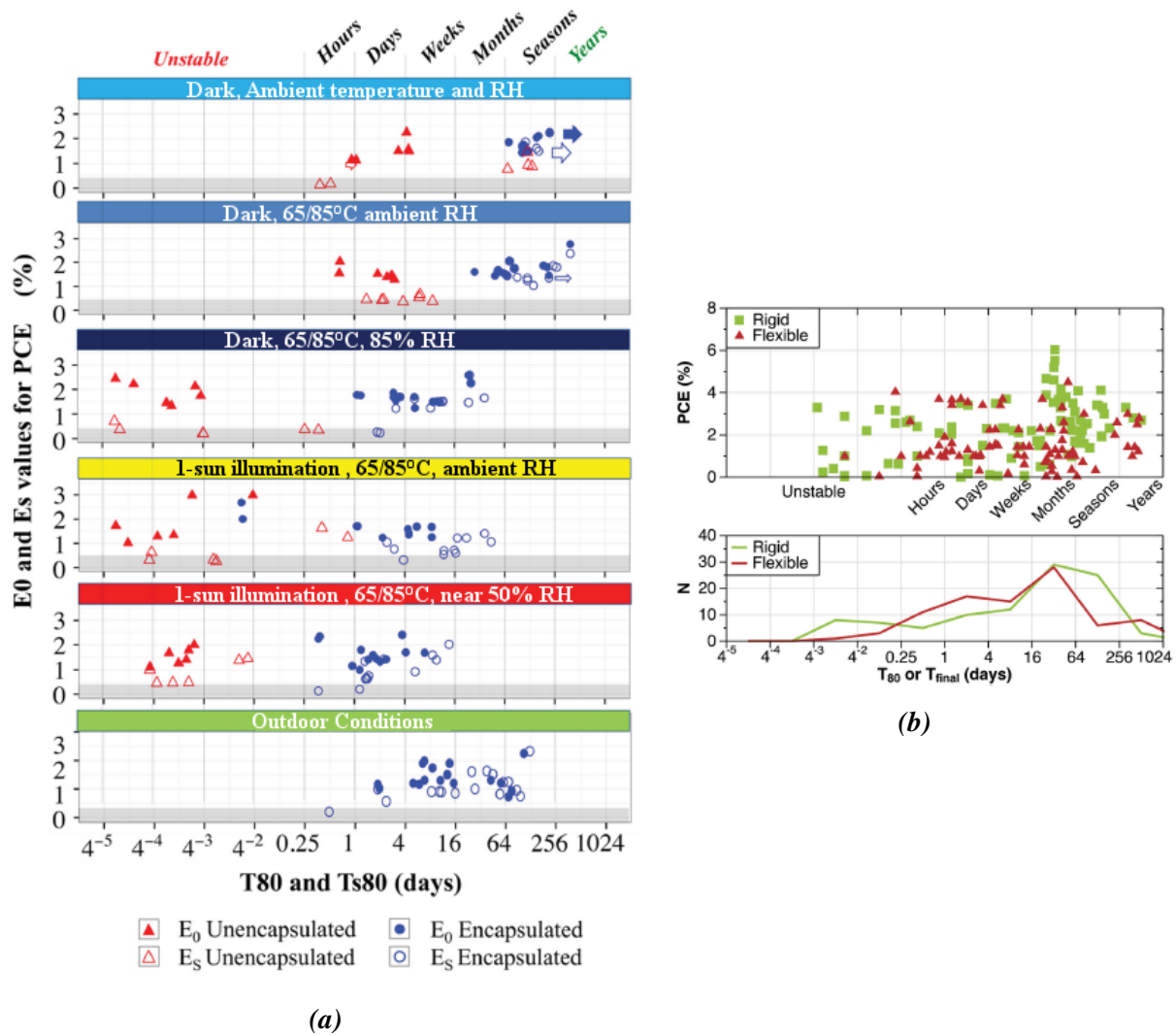
Figure 1.22: (a) E_0 and E_S , the initial efficiencies of the devices before and after burn-in, respectively, as a function of their T_{80} and T_{80} times, which represent the time at which 80% of the initial performances ( E_0 or E_S , respectively) remained. (b) PCE versus stability of devices according to the encapsulation type : rigid or flexible. All aging conditions were included in this analysis. Adapted from [66].
