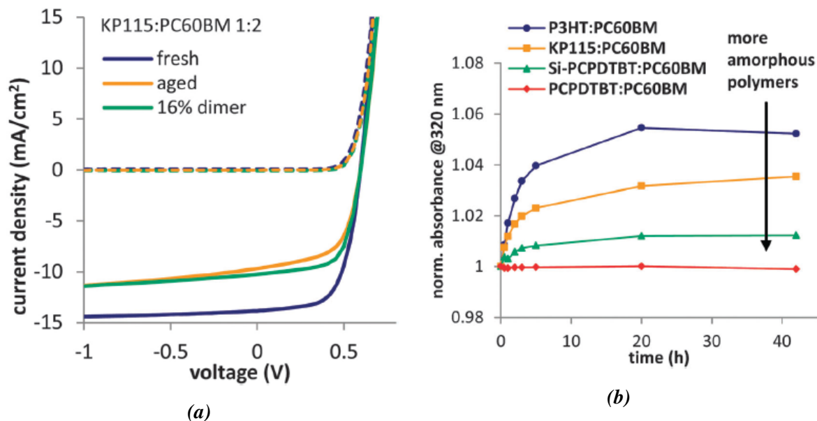
Figure 1.11: (a) Dark (dashed lines) and illuminated (plain lines) J(V) curves of fresh and aged (120 h under 1-sun illumination) inverted KP115:PC 60 BM devices along with a fresh device with a 16 % PC 60 BM dimers added to the active layer during cell production. (b) Normalized absorbance at 320 nm, representative of the PC 60 BM dimer concentration, for different donor polymers (with a 1:2 donor/acceptor ratio), plotted as a function of aging time under 1-sun illumination. Reproduced from [98].
