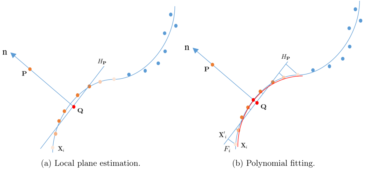
FIGURE 4.10: Surface denoising.
