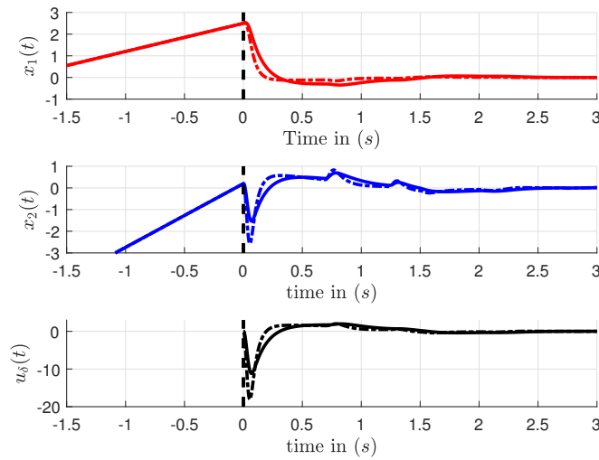
FIGURE 6.4 – Comparison of system states x_1 and x_2 and input u_\delta between two weighing cases.
