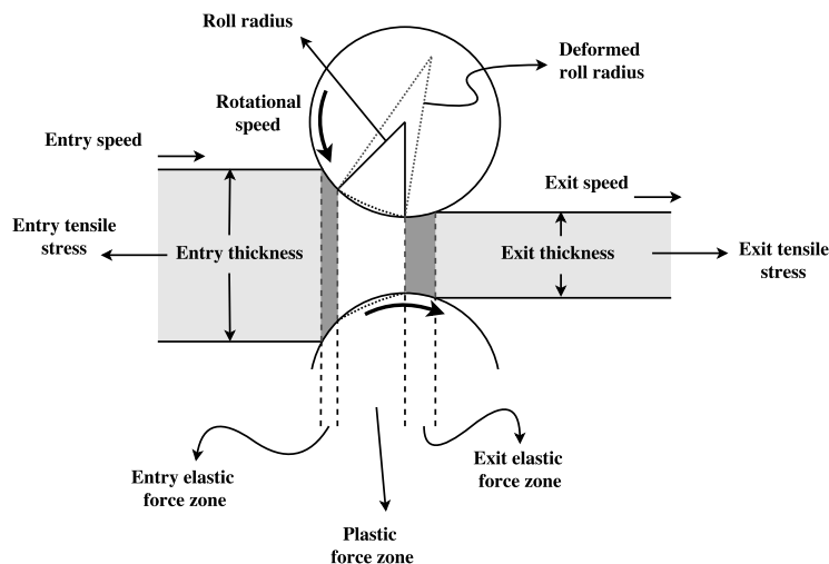
FIGURE 2.4 – Rolling deformation zone
