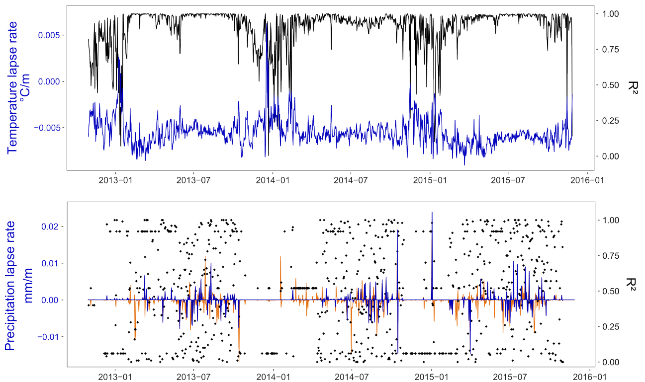
FIGURE III.6 – Daily temperature and precipitation lapse rates. Discarded precipitation lapse rates (with a R^2 < 0.75 ) are represented in orange.
