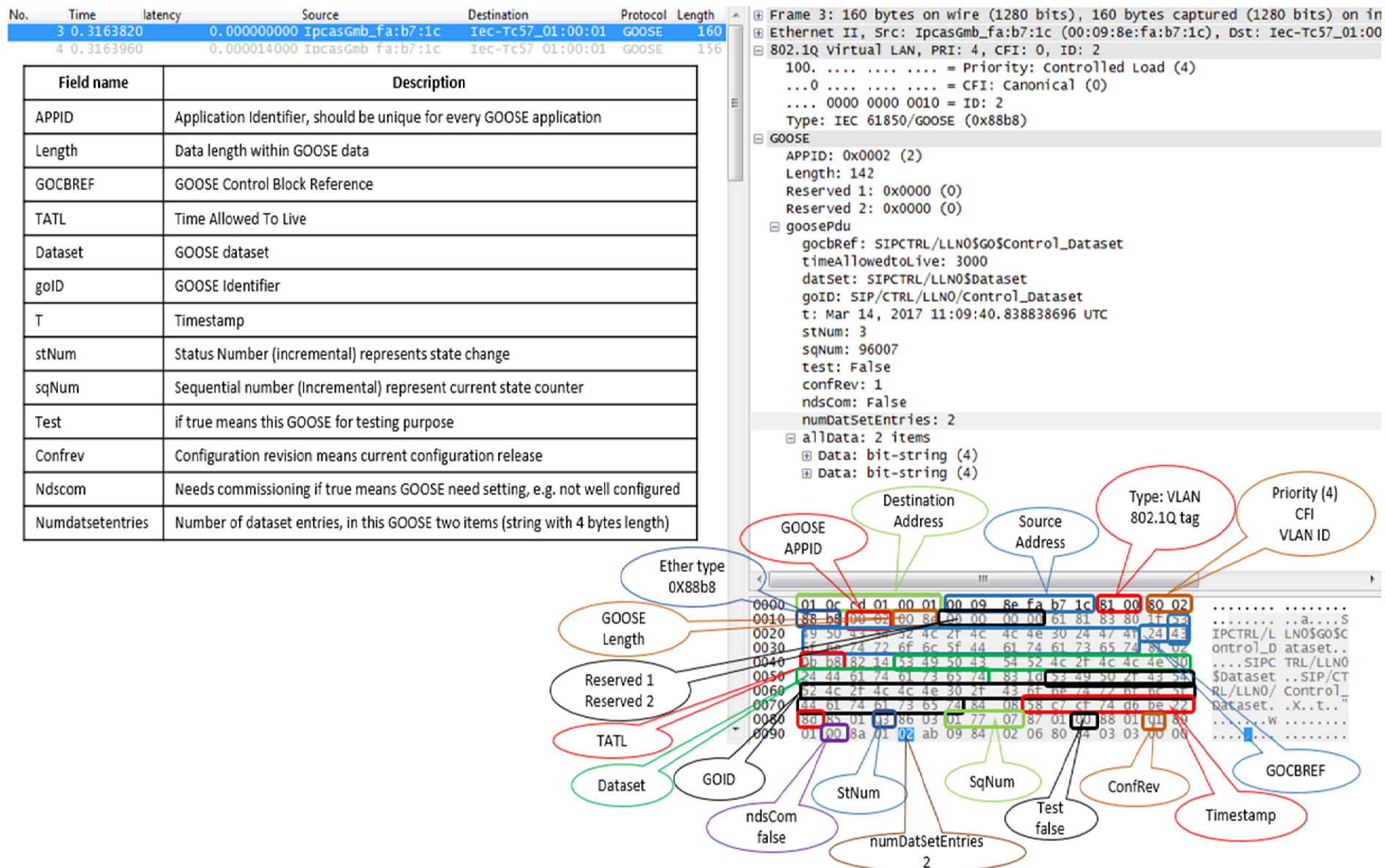
Figure A.3: GOOSE message embedded into an Ethernet frame with VLAN and priority
