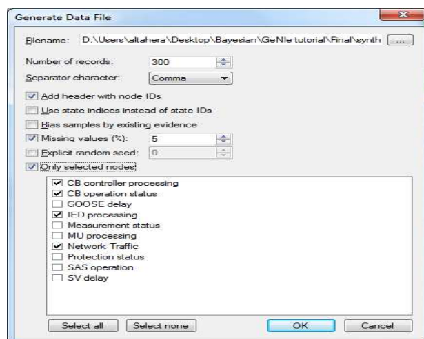
Figure 7.17: Generating a dataset with 5% missed values to evaluate the diagnosis performance of the BN model
