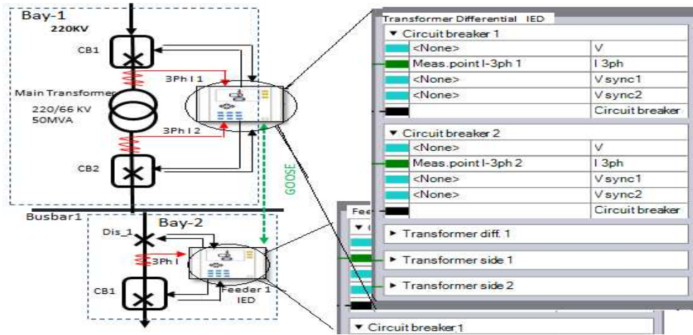
Figure 4.9: Configuring fundamental functionalities: at right side, green part represents current measurements, while black part represents circuit breaker positions
