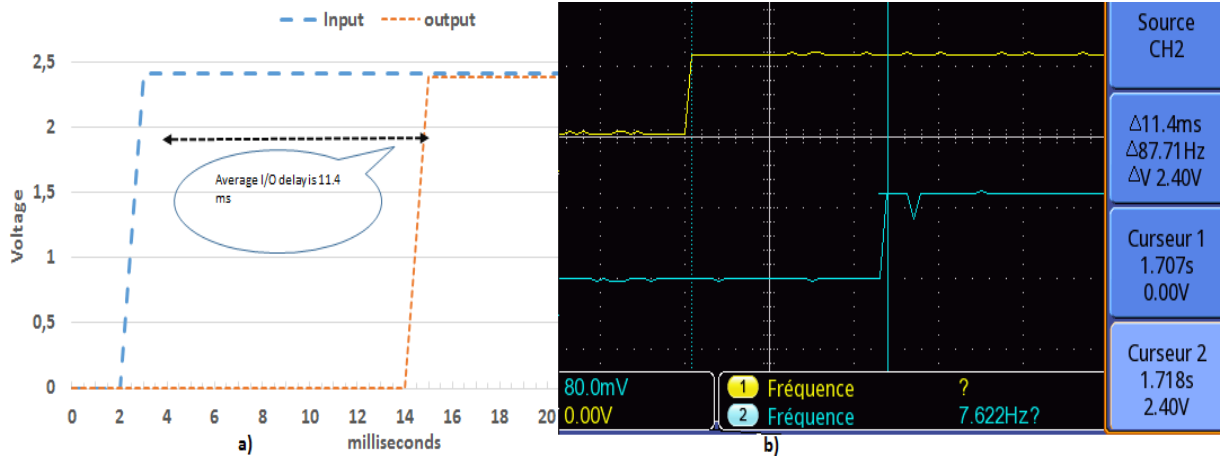
Figure 5.4: The Response time of the hardwired I/O a), Oscilloscope screenshot to measure I/O delay b)
