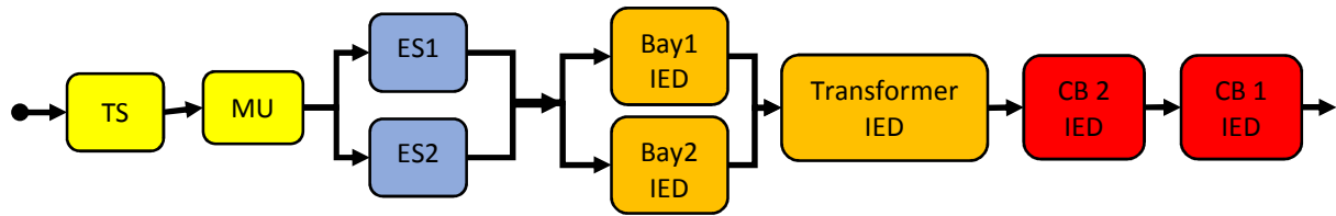
Figure 6.6: RBD diagram for the transformer bay system illustrating redundancy of Ethernet switch and Bay controller
