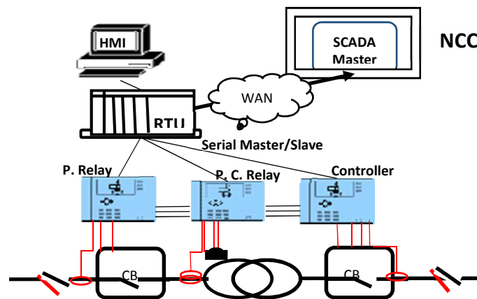
Figure 2.6 : Conventional cabling: inter-relay cabling and process hardwired connection
