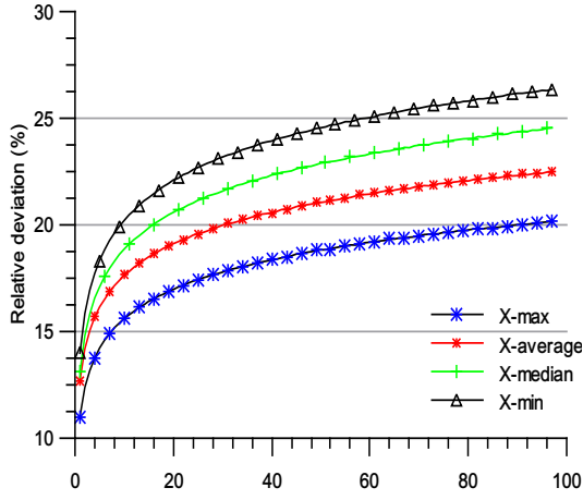
c. (m=7,n=200,d=2)
