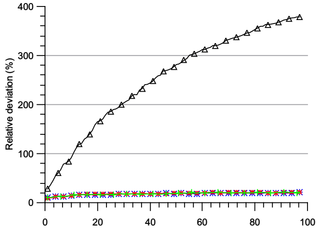
c. (m=3,n=200,d=3)
