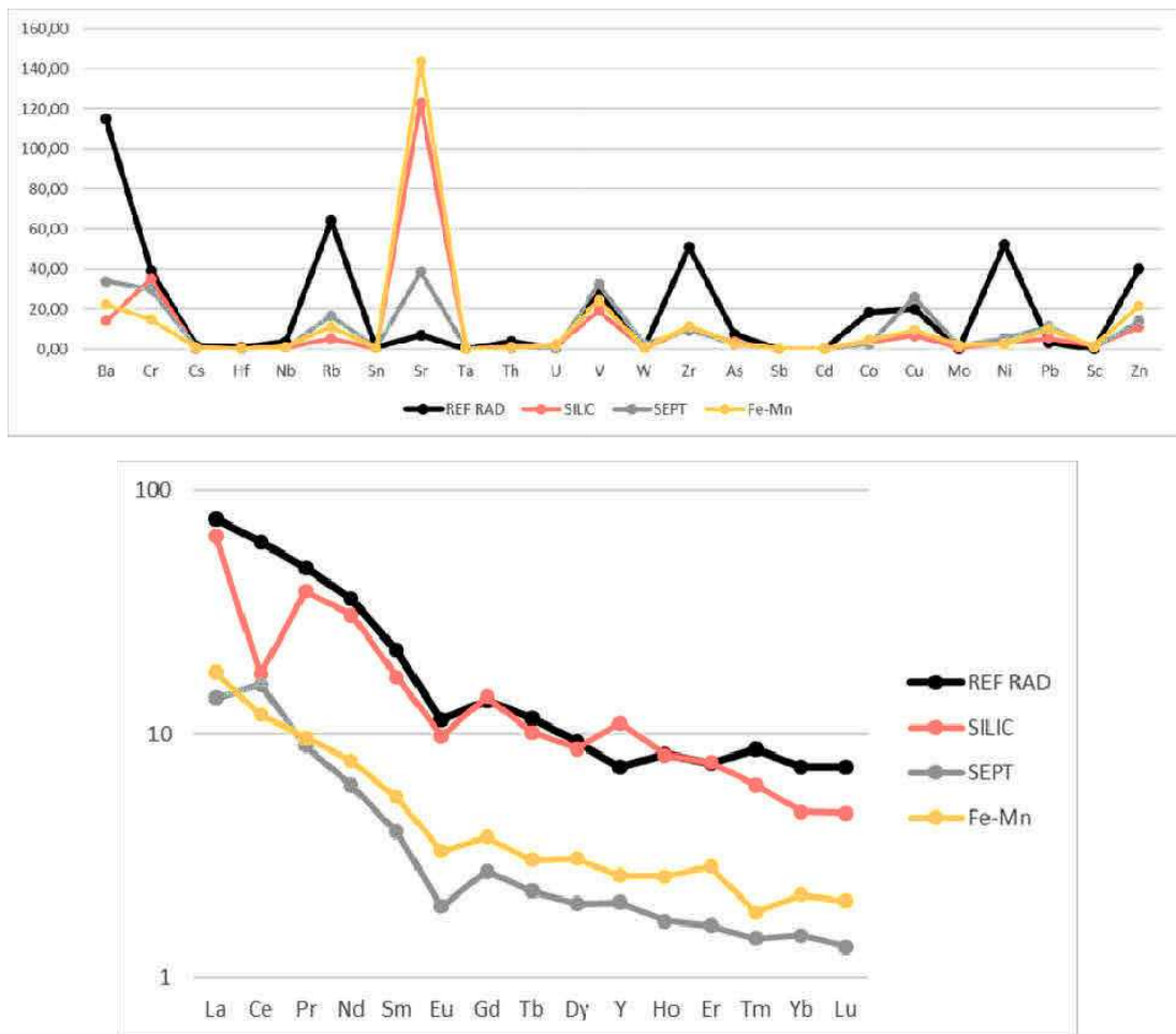
Fig. 9.4 - Trace elements content (in ppm) and chondrite-normalized REE patterns of
