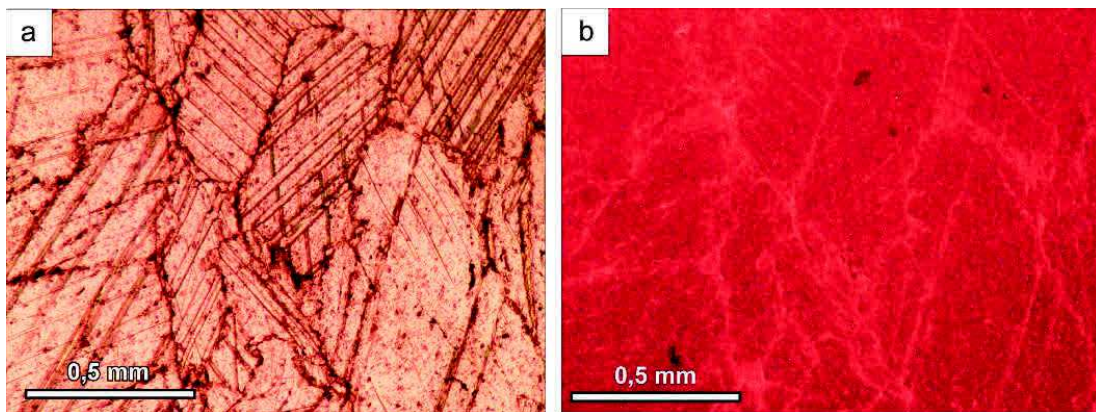
Fig. 13.11 - (a) TL and (b) CL images of dolomite marbles. Note the coarse grained textures and the sutured contact among the crystals.
