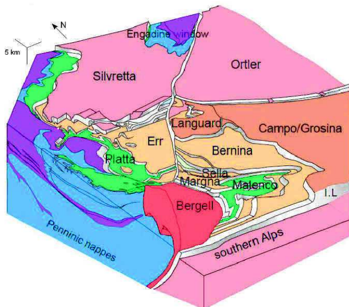
Fig. 3.2 - 3D block diagram of the present-day Alpine architecture of SE-Switzerland and N-Italy showing the Austroalpine and Penninic nappe stack (modified after Mohn et al., 2010; Froitzheim et al., 1994).
