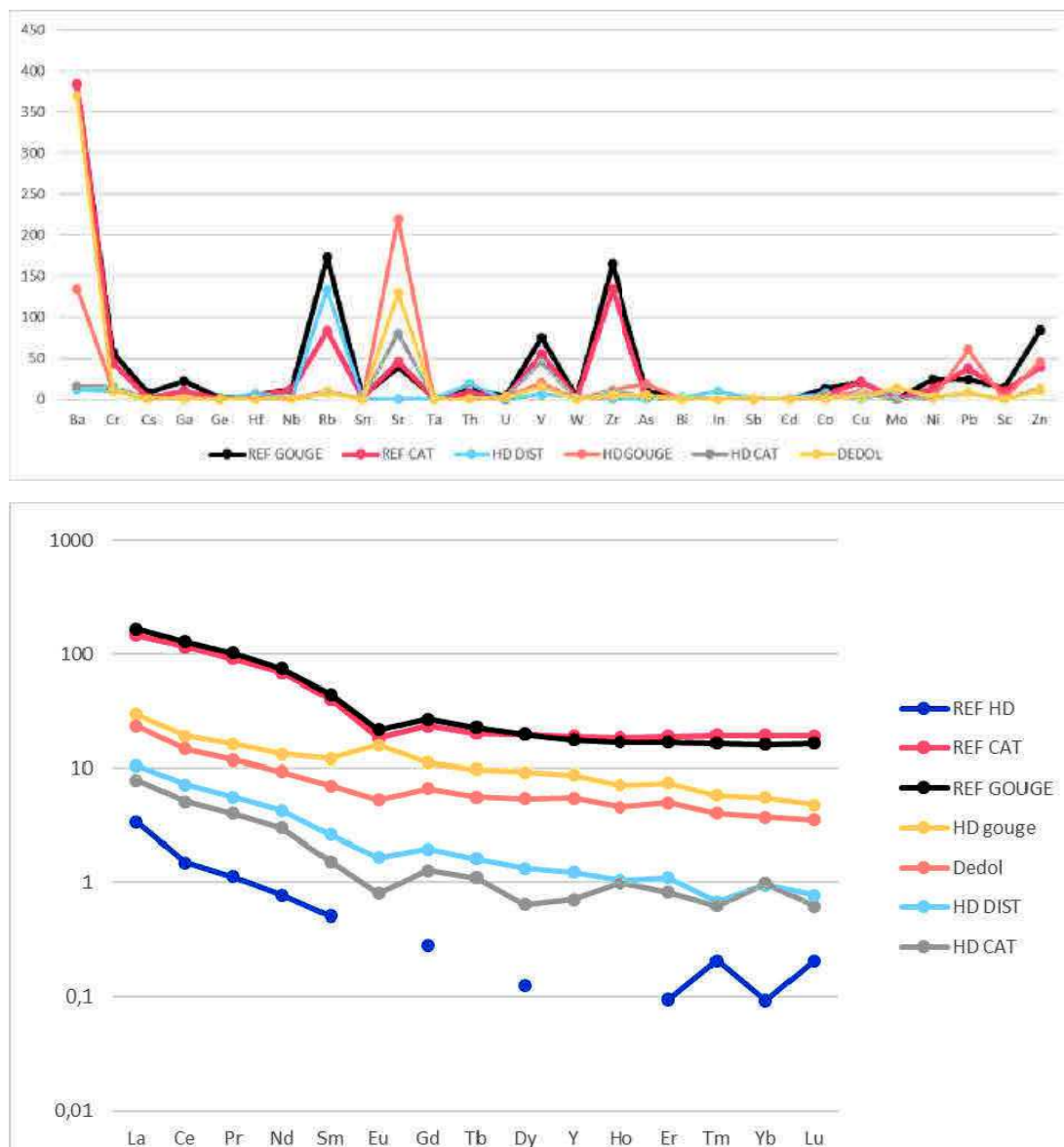
Fig. 9.2 - Trace elements content (in ppm) and chondrite-normalized REE patterns of Hauptdolomit Fm. in the Adriatic distal margin. REF GOUGE and CAT: reference samples of black gouge and cataclasite from Pinto et al. (2015); REF HD: reference samples of Hauptdolomit Fm. (courtesy of Prof. Fabrizio Berra); HD DIST: Hauptdolomit Fm. in the distal margin; HD GOUGE: clasts of Hauptdolomit Fm. within the black gouge; HD CAT: cataclasite made of Hauptdolomit Fm.; DEDOL: dedolomite.
