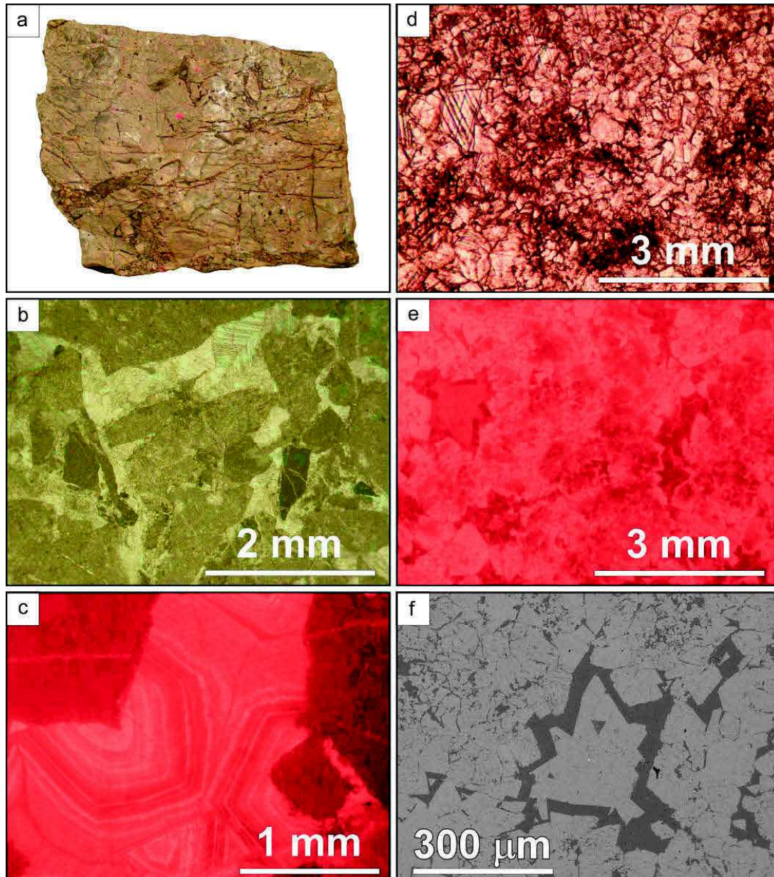
Fig. 4.3 - (a) Hand specimen of Hauptdolomit Fm. characterized by brecciated texture. (b) Transmitted light and (c) CL images of polymict rubble breccias cemented by coarse equant calcite spar, which shows oscillatory zoning. (d) TL, (e) CL and (f) SEM-BSE images of the former coarsely, crystalline, dull luminescent dolomite, dark grey in SEM-BSE, largely replaced by sparry calcite, which shows a moderate to bright yellow CL and is light grey in SEM-BSE.
