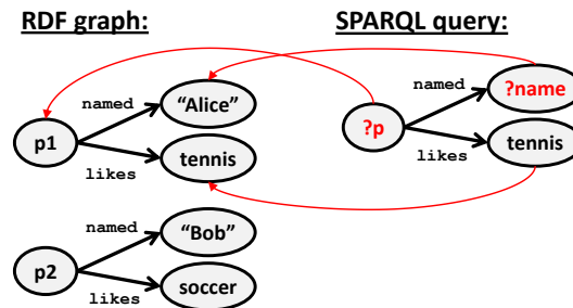
Figure 3.1: SPARQL query matching
