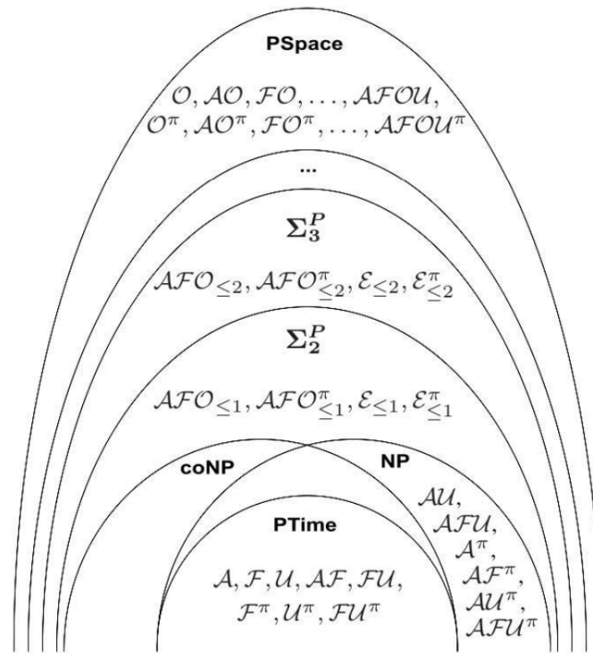
Figure 7.1: SPARQL query evaluation complexity summary
