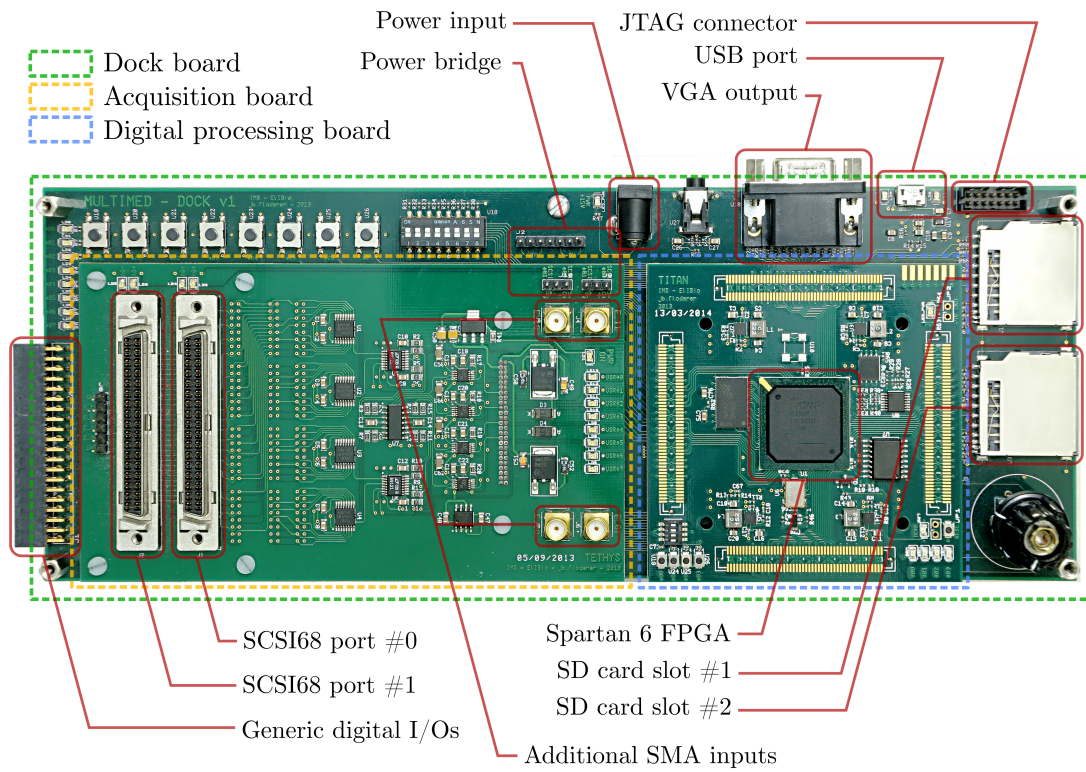
Figure 2.1 – The Multimed hardware and its key components.
