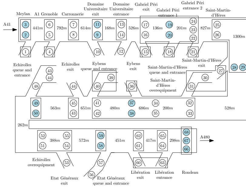
Figure 7.2: Detailed distribution of sensors within the Rocade Sud in the direction east-west. The positions of the 68 fixed sensor points are shown in the stylized map [LCK16].
