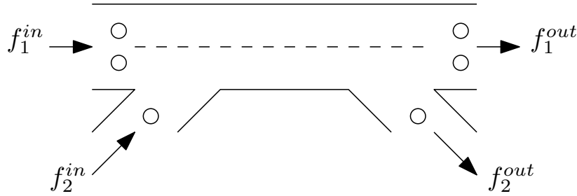
Figure 7.12: Single cell flow conservation. Averaged flow is taken into account at the input of the section and the output of the section, over a sufficient long period of time flow should be preserved
