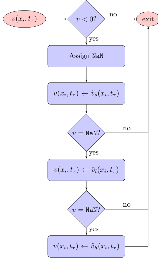
Figure 3.6: Algorithm applied for imputation. Left-hand side: Algorithm sequence / Right-hand side: Flow diagram to illustrate data work flow
