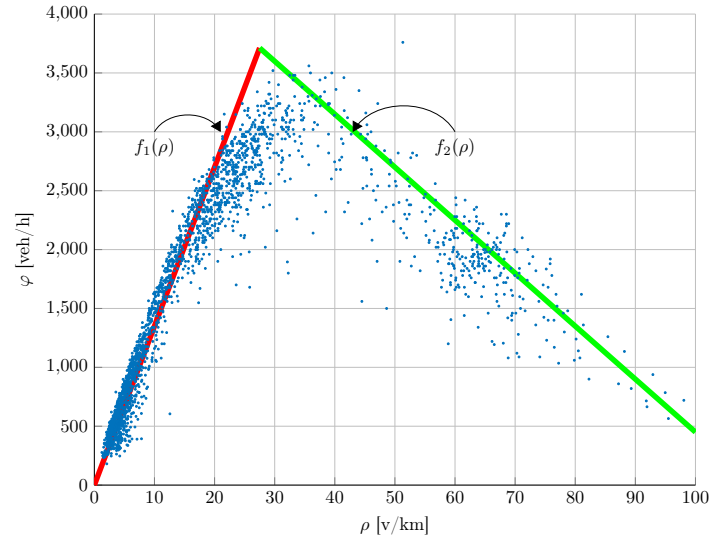
Figure A.2: Density- flow data relationship. Section Meylan | - A41. Analyzed date: 21, May 2015
