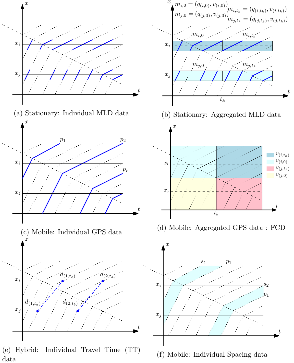
Figure 2.3: Measurement technologies in traffic systems
