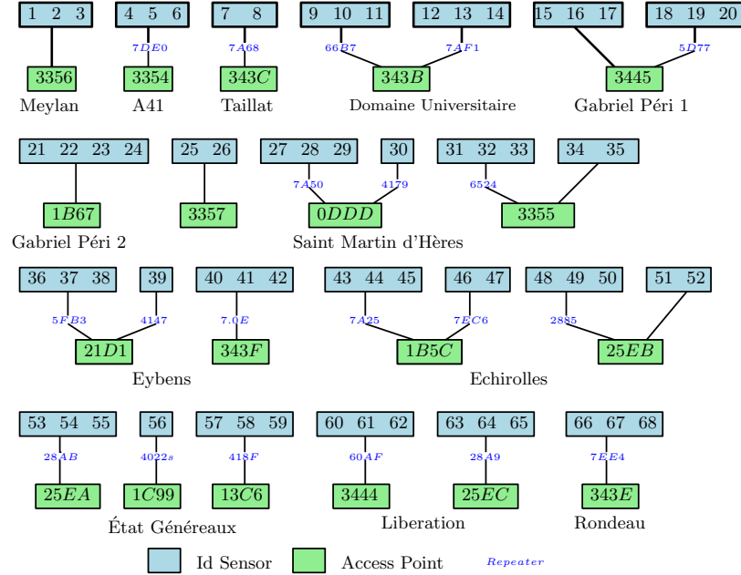
Figure 7.3: Network representation of Station / Collection Points and sensors within the Rocade Sud in the direction east-west. Each sensor identified with a number is grouped in a collection of sensors denominated SCP. Each SCP is connected to an AP in a direct form or throughout a repeater
