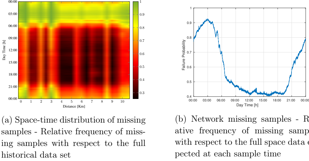
Figure 3.3: Missing data evaluation of the GTL from September 1 st , 2015 to March 31 st , 2016. The figure on the left panel illustrates the distribution of missing samples analyzed from an historical view point. At each sample time and specific location the amount of missing samples is counted within the historical data set. The right panel displays the distribution of missing samples along the day, as a remark the peaks of missing data are concentrated out of the peak hours which benefits the algorithm in this study.
