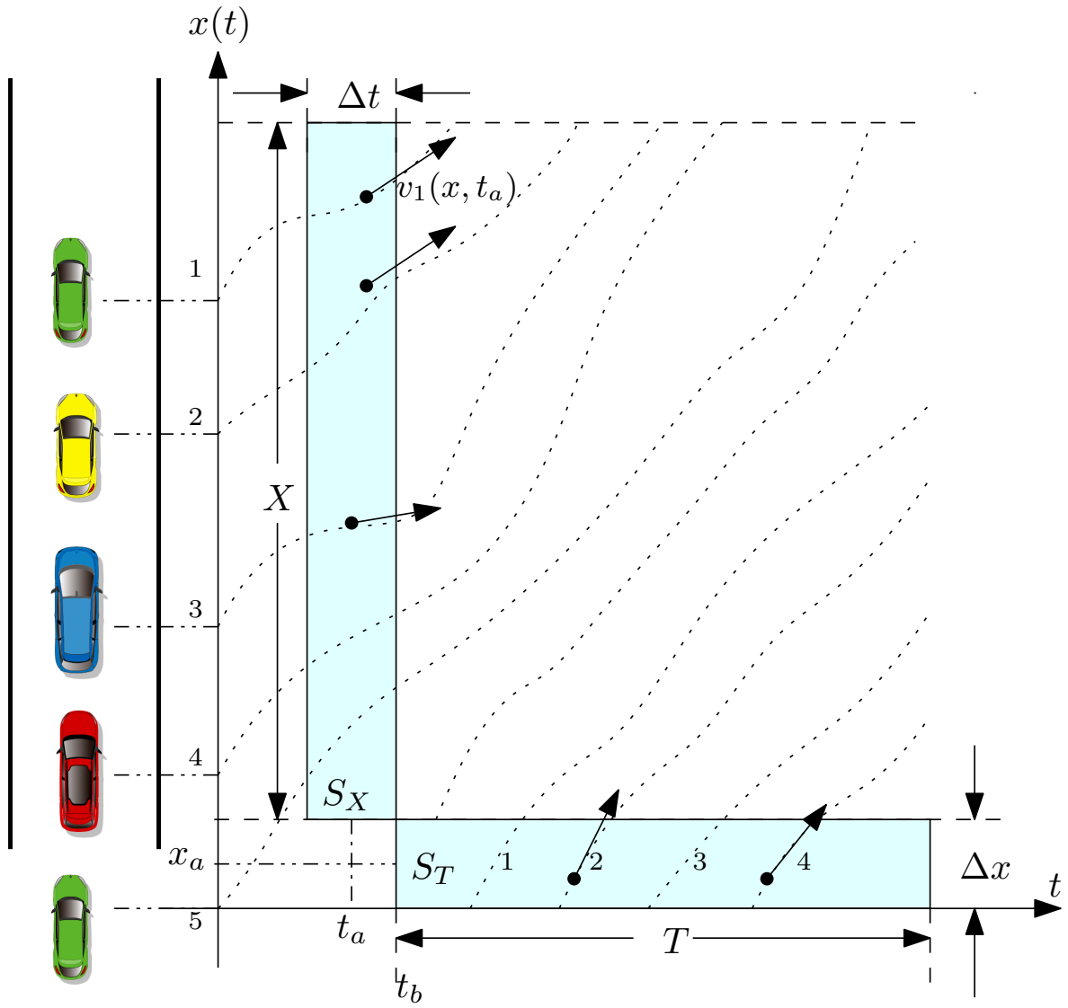
Figure 3.1: Relationship between microscopic and macroscopic variables
