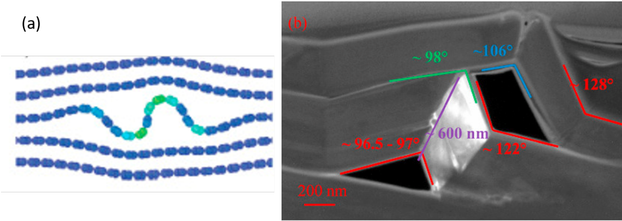
Figure 4.6. (a)schematic illustration of bulk ripplocation in graphite(b) TEM image of bulk ripplocation formed in Ti_3SiC_2 by indentation [35].
