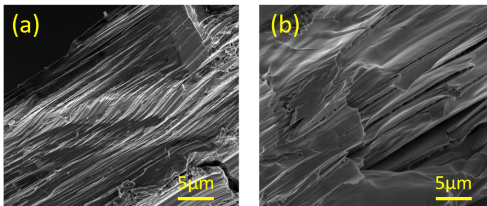
Figure 2.29. cross-section of broken crystal Cr 2 AlC (a) raw (b) after chrono-amperometric anodization at 900mV for 6h in EDTA with ammoniac buffer.
