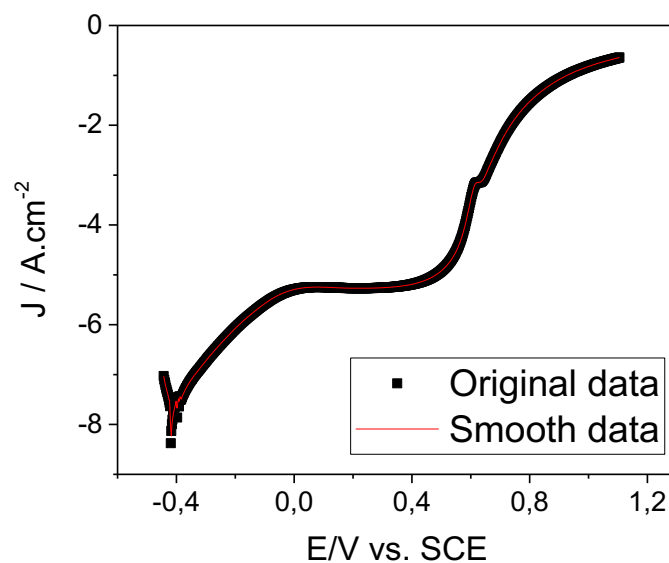
Figure 4.17. Smoothed polarization curve of Cr 2 AlC c-plane working electrode in H 2 SO 4 from OCV (-0.4V) to 1.2V vs SCE with sweep rate of 1mV/s.
