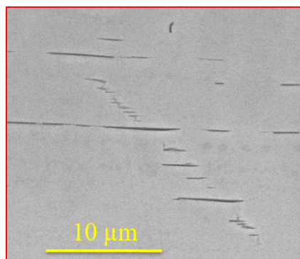
Figure 4.13. Fine polished Cr 2 AlC sample(C-0.03μ) polarized from OCV to 0.75V vs. SCE in 1M H 2 SO 4 with sweep rate of 1mV/s
