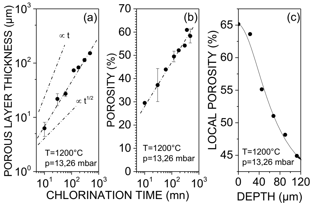
Figure 3.22. (a) Converted layer thickness versus time, (b) porosity as a function of time and (c) local porosity as a function of depth for an exposition \Delta t=5\text{h} . In all experiments T=1200^\circ\text{C} . Solid lines are guides to the eye.
