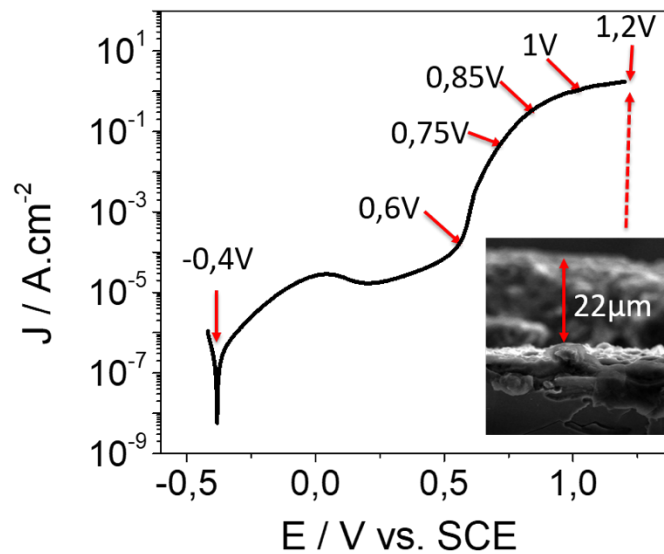
Figure 4.9. Typical polarization diagram for the Cr 2 AlC single crystal in 1M H 2 SO 4 from OCV to 1.2V vs. SCE with sweep rate of 1mV/s. The voltages, where the sample cross-section is observed by SEM, are indicated. Inset: SEM micrograph for a side view of a fine polished sample (C-0.03 µm) polarized from OCV to 1.2V vs. SCE with sweep rate of 1mV/s in 1M H 2 SO 4
