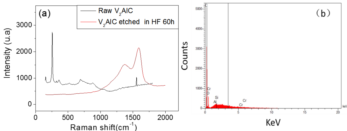
Figure 2.4. (a) Raman spectra of raw crystal V_2AlC and V_2AlC etched in HF 60hours. Wavelength: 473 nm. Hole: 200 \mu m . Network: 1800. Exposure time: 10s and 8 cycles (b) EDS analysis of V_2AlC etched in HF 60 hours.
