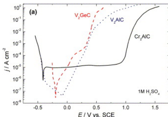
Figure 2.17. Cr_2AlC polarization curve (black) in H_2SO_4 1mol/L with sweep rate of 1mv/s [42].
