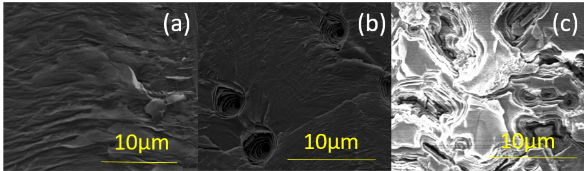
Figure 2.3. SEM observation of V_2AlC single crystal after 16h HF 48% treatment(a) layer exfoliation(b) defect holes(c) defect by HF etching
