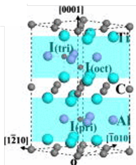
Figure 4.22. (a) Schematic defect-in-supercell model of possible interstitial sites (smallest atoms) in Ti_2AlC
