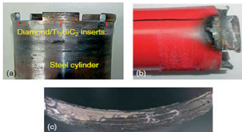
Figure 1.22. (a) Diamond/ Ti_3SiC_2 insert (b) Diamond/Co inset, both brazed on steel hollow cylinder after dry drilling of concrete, (c) insert detail of MAX based inset after dry drilling. (Products of 3-ONE-2.). [42]
