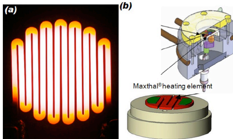
Figure 1.19. (a) An example of Ti_2AlC -based heating element resistively heated to 1450^{\circ}C in the air (Products of 3-ONE-2 Inc.). (b) Maxthal 211 heating elements in reactor cell for three-way catalyst
