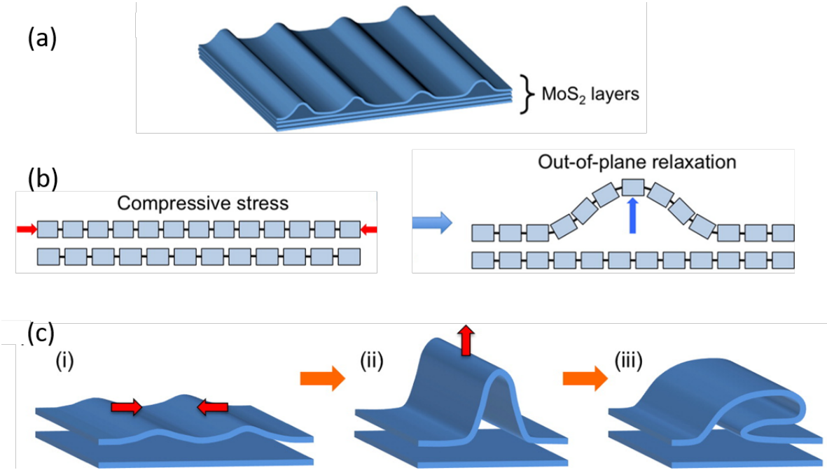
Figure 4.5. (a) schema of surface ripplocation of MoS_2 layer[34](b)schematic explanation of the formation of ripplocation ,simulated by DFT, by inserting an extra-line of layer in the MoS_2 bi-layer structure (c) schematic DFT simulation of the aggregation and self-folding of the ripplocations.
