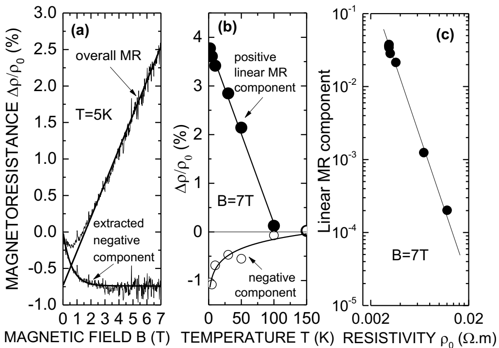
Figure 3.10. Magnetoresistance (MR) of the same sample as in Fig.9. (a) MR versus magnetic field at T=5K , (b) linear positive MR component at B=7T and saturated negative MR component at B=7T as a function of T and (c) variation of the linear positive MR component at B=7T as a function of the overall resistivity \rho_0 at B=0 .
