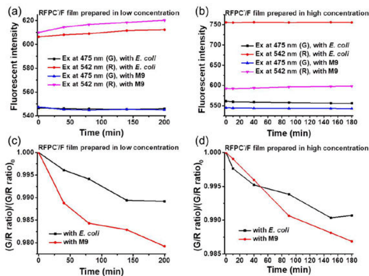
Figure 5.15. Fluorescence intensity of RFPC/fluorescein surface that were prepared with low (a) and high (b) concentration deposition solutions in the presence of E. coli bacteria as a function of time. A control was also recorded: RFPC/fluorescein surface in the presence of modified M9 minimal medium. The excitation wavelength was 475 nm or 542 nm. (c and d) Normalized Green/Red fluorescence ratio of the RFPC/fluorescein surface as a function of time. Green and Red indicate the fluorescence intensity of the ratiometric surface at \lambda_{ex} = 475 nm and 542 nm, respectively.
