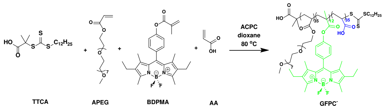
Scheme 3.5. Synthetic scheme employed for the RAFT synthesis of P(APEG- co -GBDPMA- co -AA) (GFPC - ).
