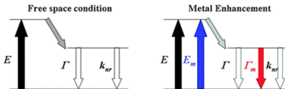
Scheme 3.1. Classical Jablonski diagram for the free-space condition and the modified form in the presence of a metallic surface. E: excitation rate, E m : metal enhanced excitation rate, and Γ m : radiative rate in the presence of a metal. From Geddes and Lakowicz [3].
