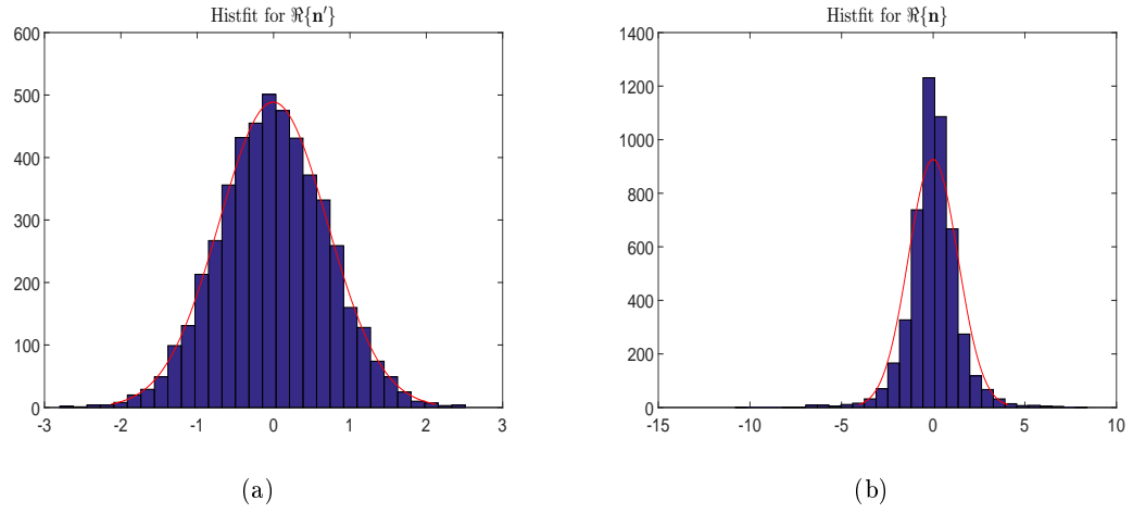
Figure 3.3: Histograms with fitted normal distribution for (a) \Re\{\mathbf{n}'\} and (b) \Re\{\mathbf{n}\} .
