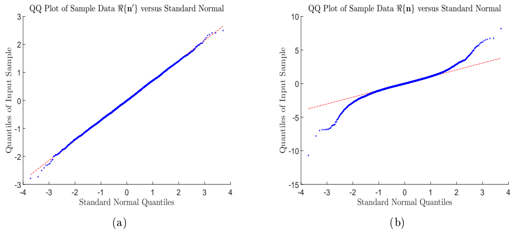
Figure 3.4: Quantile-quantile plots for (a) \Re\{\mathbf{n}'\} and (b) \Re\{\mathbf{n}\} .
