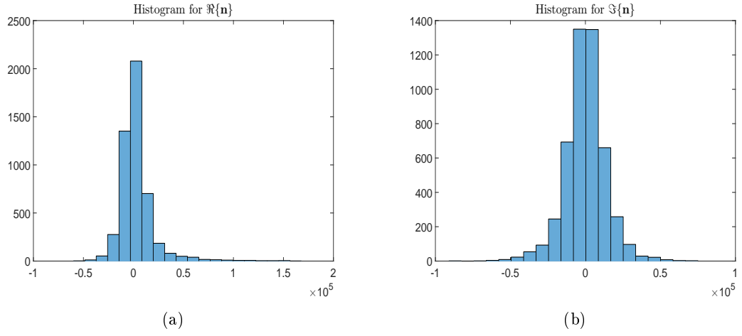
Figure 3.2: Histograms for (a) \Re\{\mathbf{n}\} and (b) \Im\{\mathbf{n}\} (realistic case).
