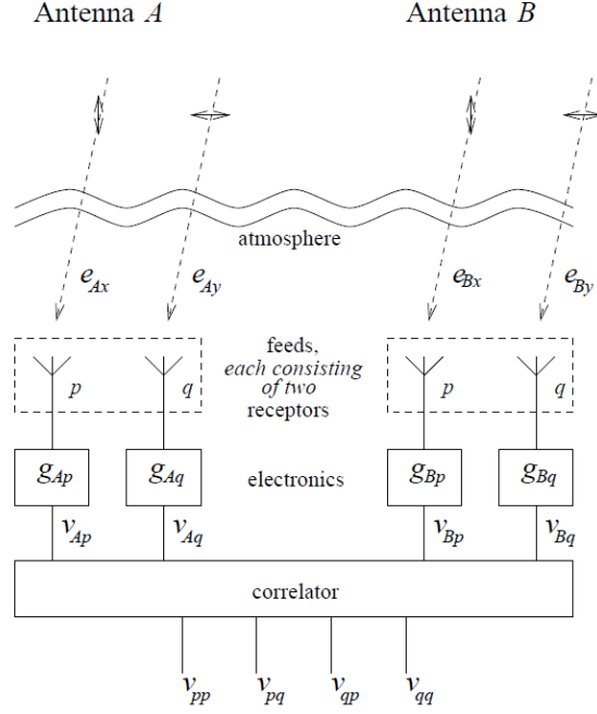
Figure 2.5: Interferometric system (after [5]).
