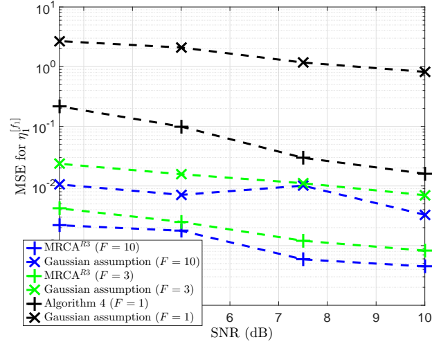
Figure 4.3: MSE of \eta_1^{[f_1]} vs. SNR, for D = 2 bright signal sources, M = 8 antennas and D' = 4 weak background sources.
