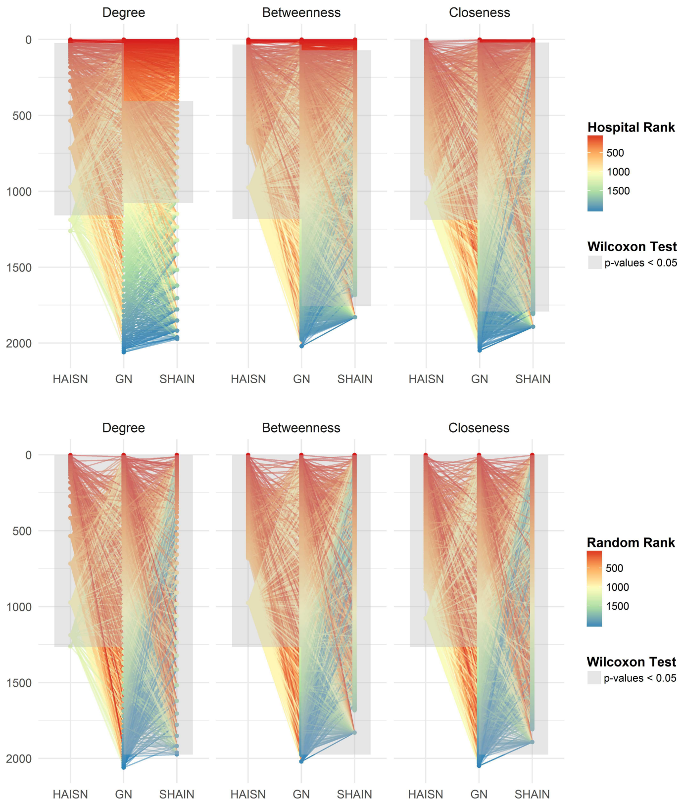
Fig 1. Hospital rankings by degree, betweenness, and closeness across the networks. Hospitals in the HAI-specific network (HAISN) ( n = 1266 ), suspected-HAI network (SHAIN) ( n = 1975 ), and general network (GN) ( n = 2063 ) are displayed vertically and plotted against their ranking by degree, betweenness, and closeness centrality measures (top row). Only the hospitals shared between the HAISN and GN or the SHAIN
