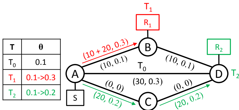
Figure 3.3: Example of L2BM functioning
