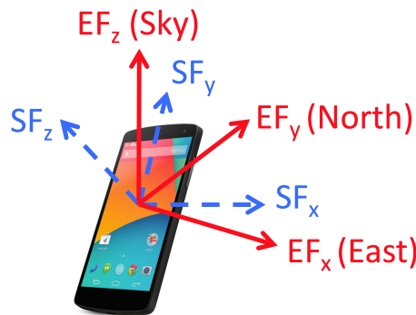
Figure 1.7: The Smartphone-Frame SF (dashed line) and ENU-Frame EF (solid line).
