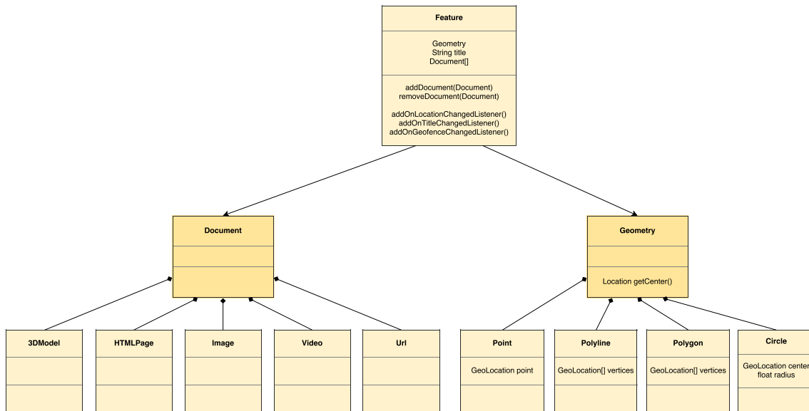
Figure 5.1: Hierarchy of features and documents handled by our format.
