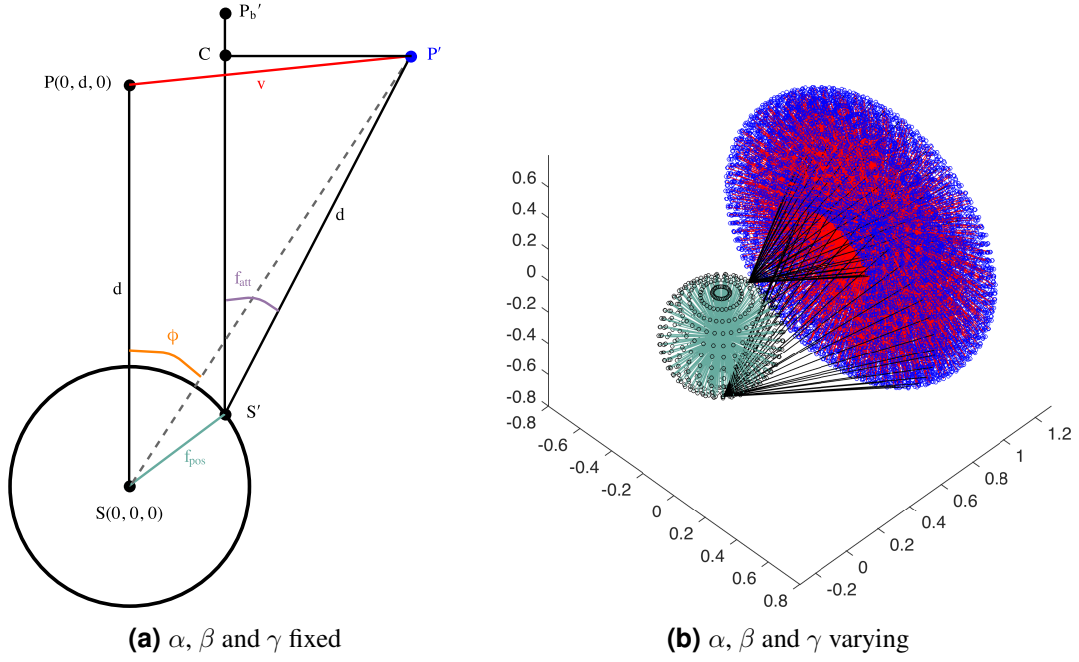
Figure 4.4: Evaluation model where f_{\text{att}} and f_{\text{pos}} are fixed
