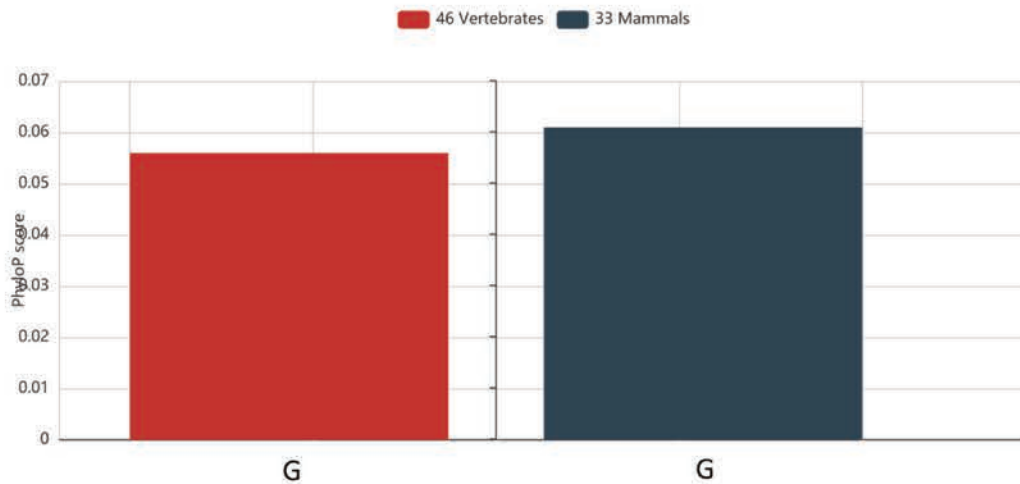
Sup. Figure 1: PhyloP scores of 46 vertebrates and 33 mammals for the guanine of rs6918289
