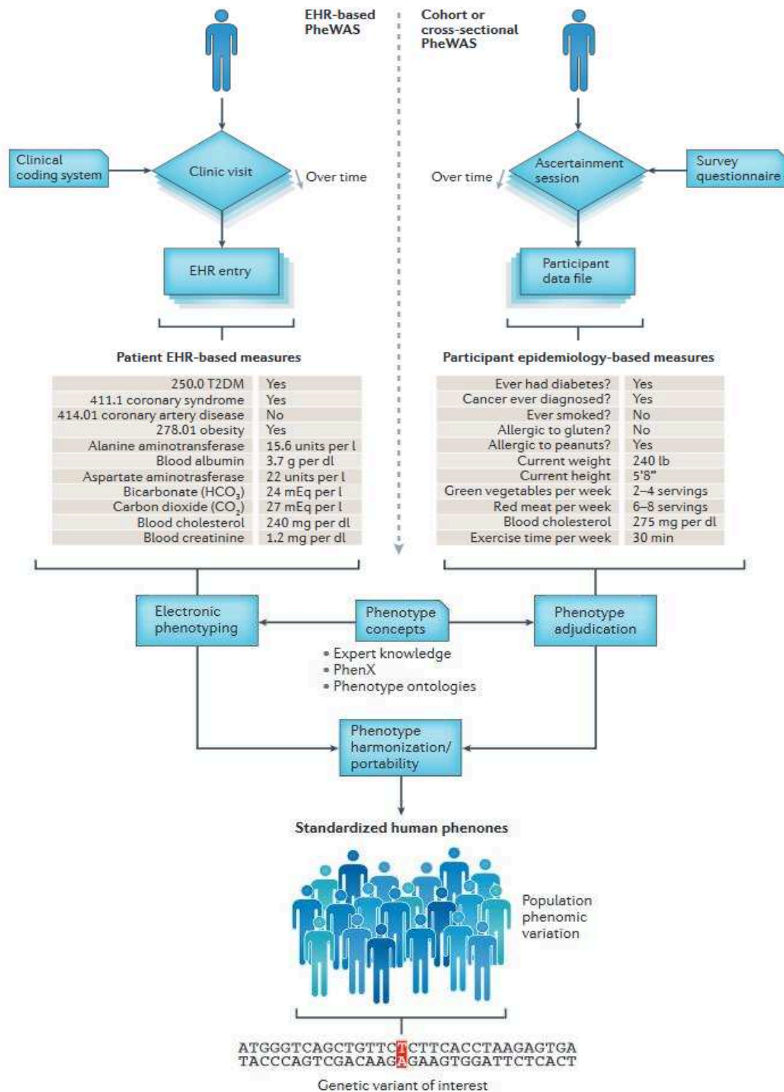
Figure 27: Characterization of human phenome for PheWAS. Human phenome characterization requires a broad data collection system, either an EHR system or an epidemiological study (a cohort or cross-sectional study).
