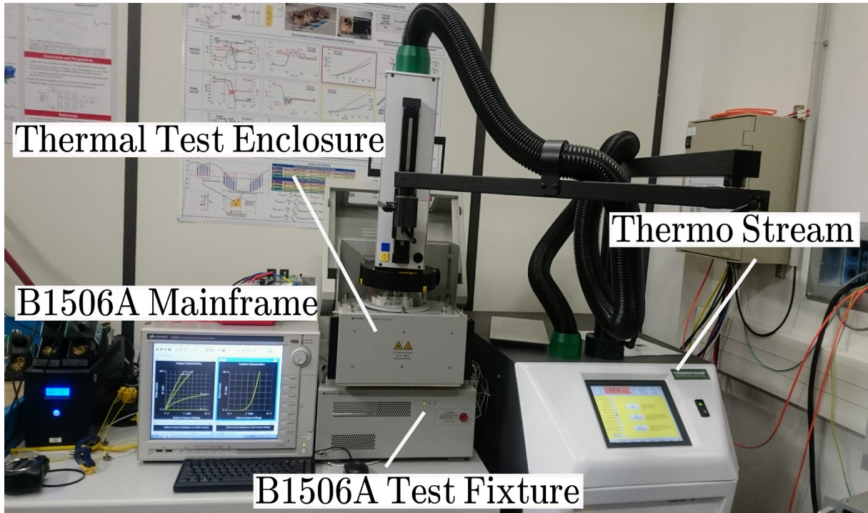
Fig. 5.2: Monitoring the electrical parameters using the B1506A Analyser with the Thermo Stream
