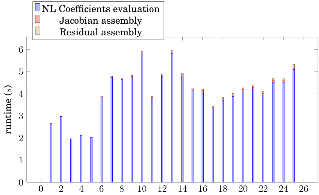
Figure 7.9 – Opus Application without Stabilization: Runtime of the main phases for the online resolution. Mean value for 50 runs. Other contributions are negligible
