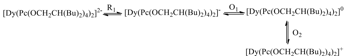
Scheme IV.2. The one-electron redox processes of 4
