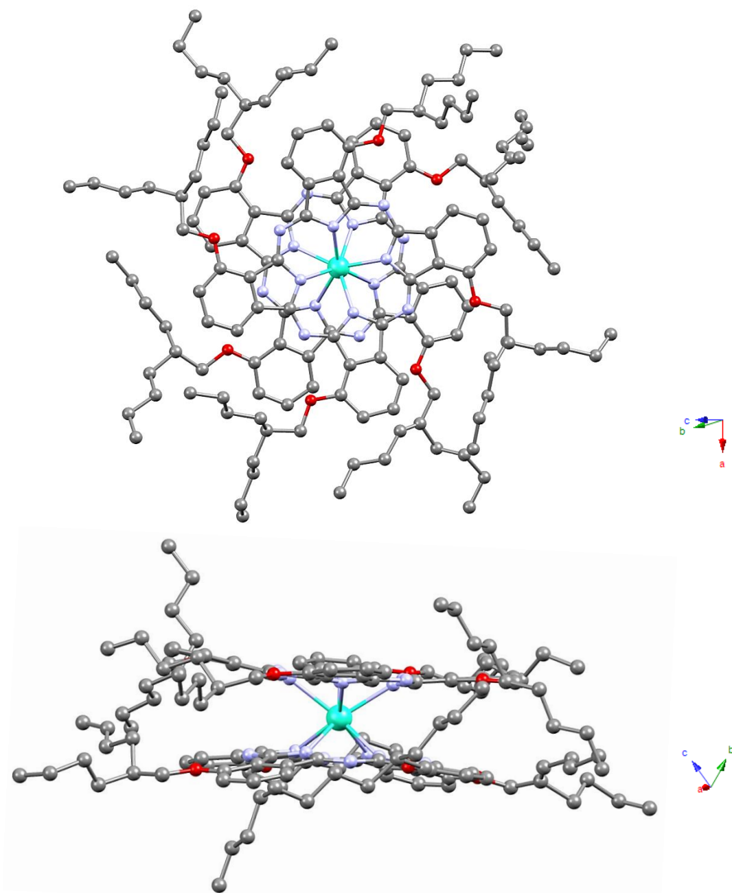
Figure IV.20. Molecular structure of the C 4h isomer of [Dy{Pc(OCH 2 CH(Bu) 2 ) 4 } 2 ] 0 ( 4* ) viewed along a axis (top) and viewed from the side (bottom). Color scheme: C gray, Dy emerald, N blue, O red.
