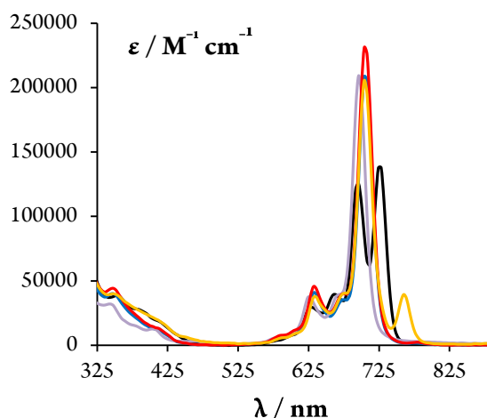
Figure II.16. Absorption spectra ( 5\mu\text{M} in \text{CH}_2\text{Cl}_2 ) of the \text{H}_2\text{Pc}(\text{OCH}_2\text{CHPent}_2)_4 ( 3b ) (black) and corresponding metal(II) phthalocyaninates, 4b (Co, blue), 5b (Ni, purple), 6b (Cu, red), 7b (Zn, yellow).
