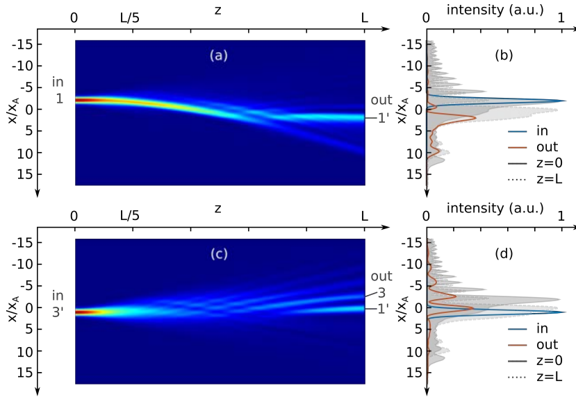
Figure 4.13: Linear probe beam propagation in the waveguide structure induced by misaligned Airy beams [Figs. 4.11(c)-(d)]: (a) Intensity distribution and (b) transverse profiles of a Gaussian beam guided along 1 \rightarrow (1', 3) , (c)-(d) guided along 3' \rightarrow (1', 3) .
