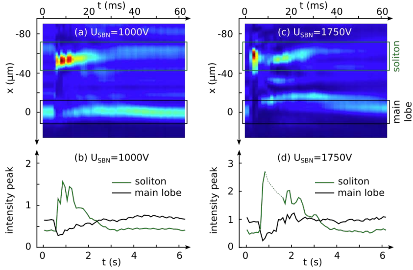
Figure 4.19: Influence of the external bias electric field on the waveguiding strength and stability, with D = -x_A , P_A = 60 \mu\text{W} and x_A = 9.5 \mu\text{m} . (a) (resp. (c)) Experimental transverse intensity distribution of the output beam at z = L along time and (b) (resp. (d)) temporal evolution of the energy concentrated around the linear forward main lobe's position and around the solitonic output position (enhanced by the backward main lobe) for U_{\text{SBN}} = 1000 \text{V} (resp. U_{\text{SBN}} = 1750 \text{V} ).
