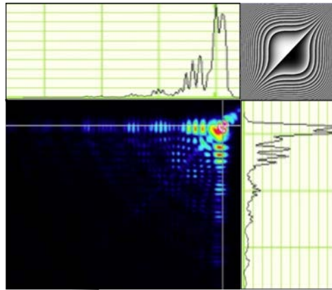
Figure A.2: Experimental optical beam after a 2D cubic phase modulation through the SLM. Airy-like intensity distribution after the Fourier transformation. Right corner: phase modulation applied on the SLM.
