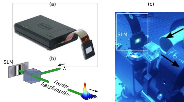
Figure A.1: SLM-based Airy beam generation. (a) Spatial Light Modulator PLUTO Holo-eye. (b) Schematic view of the experimental setup. (c) Illustration of the SLM-setup in our experiment.
