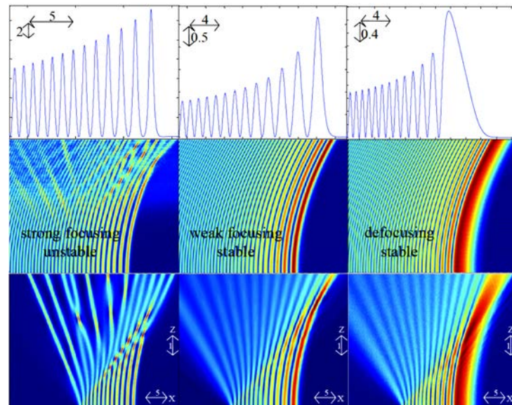
Figure 2.4: Self-accelerating beams in Kerr media. Top row: Intensity profiles at z = \frac{1}{4} o . Middle row: Propagation of self-accelerating beams with infinite tails and 2 % noise. Bottom row: Propagation of self-accelerating beams with finite tails. Left column: Strong focusing nonlinearity. Middle column: Weak focusing nonlinearity. Right column: Defocusing nonlinearity. Extracted from Ref. [97].
