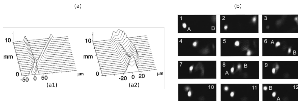
Figure 4.4: Two incoherent co-propagating Gaussian solitons launched along non parallel trajectories in photorefractive media. (a) Typical interaction scheme. Extracted from [66]. (b) Time-resolved complex rotation of a soliton pair. The sequence starts when a second beam is launched onto a steady-state soliton. The time interval between consecutive frames is 0.36 s. Extracted from [128].
