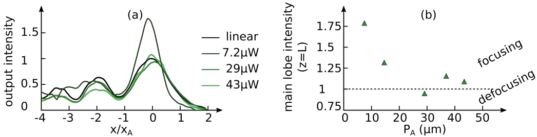
Figure 2.16: (a) Normalized intensity distribution of a self-trapped Airy beam propagating in a focusing photorefractive crystal at t = 30 s, with x_A = 14 \mu\text{m} , E_e = 4 kV/cm and L = 1 cm, (b) detailed evolution of the normalized maximum peak value of the self-focused Airy beam for increasing optical power.
