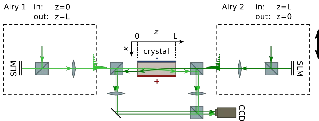
Figure 4.15: Study of two incoherent counterpropagating Airy beams in a biased focusing photorefractive (PR) crystal: experimental setup.
