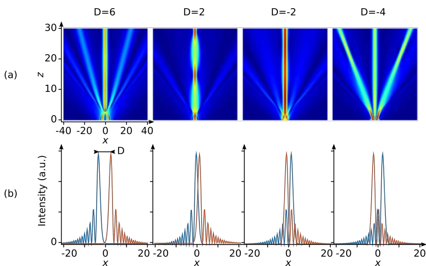
Figure 4.7: Soliton formation through the interaction of two in-phase co-propagating Airy beams in a Kerr medium. D represents the beams' shift. (a) Intensity distribution along the medium. Extracted from [140]. (b) Transverse intensity profiles of both beams at z = 0 .
