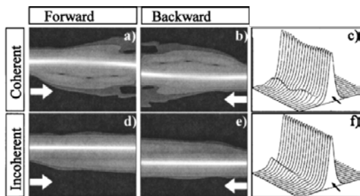
Figure 4.6: (a)–(c) Coherent interactions between the counterpropagating (a),(c) forward and (b) backward solitons. (d)–(f) Incoherent interactions between the counterpropagating (d),(f) forward and (e) backward solitons. The plots show absolute values of the field amplitudes. The arrow indicates the propagation direction of each beam. Extracted from [136].
