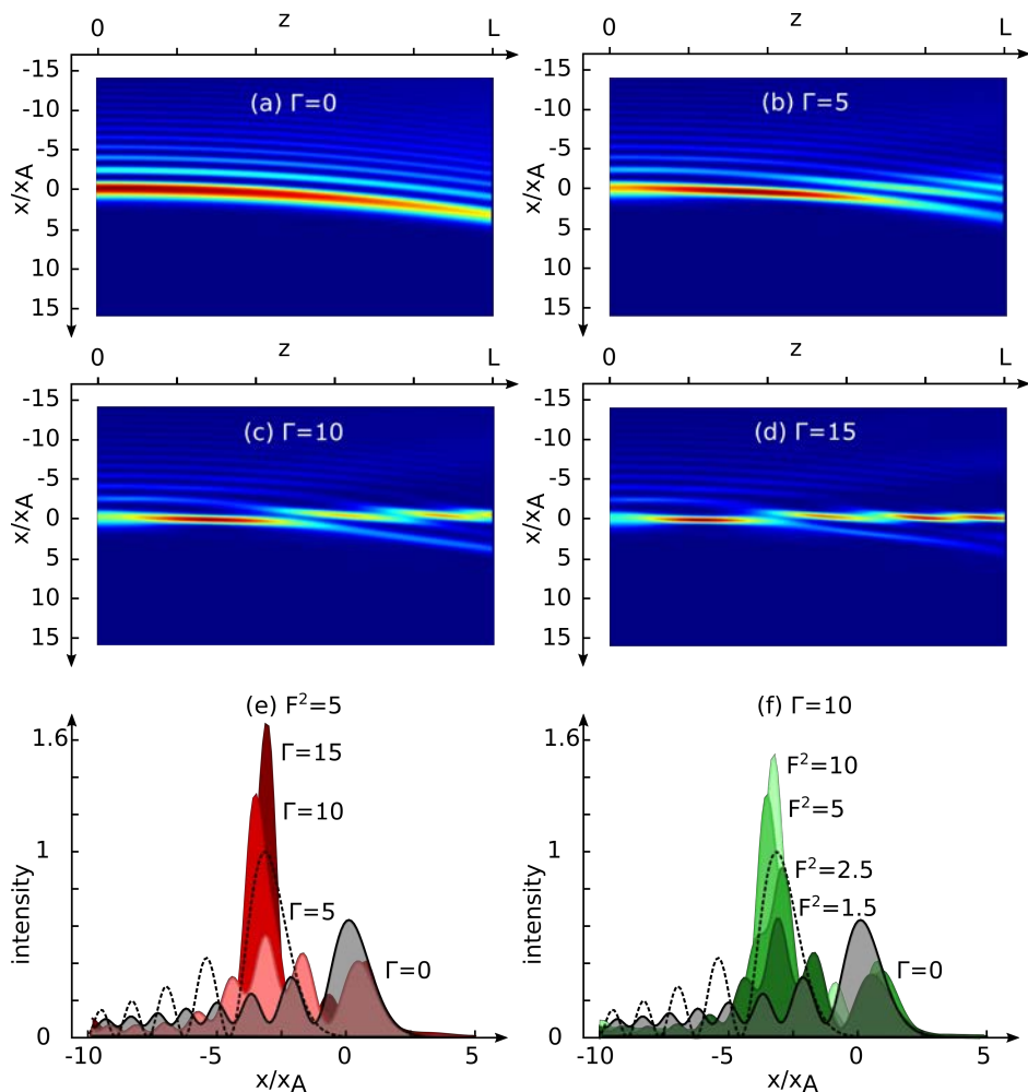
Figure 2.15: Propagation of a self-focused Airy beam propagating in a photorefractive crystal, with x_\Lambda = 10 \mu\text{m} , L = 1 \text{ cm} and t_f = 6\tau . Intensity distribution along the crystal with F_\Lambda = \sqrt{5} under (a) linear and (b)-(d) nonlinear condition with an increasing bias electric field ( \Gamma = (knx_\Lambda)^2 r_{\text{eff}} E_e ). Transverse intensity profiles of the off-shooting soliton at the output of the crystal, z = L and t_f = 6\tau , for (e) increasing electric field and (f) increasing optical power. The input Airy profile at z = 0 is plotted by a dashed line.
