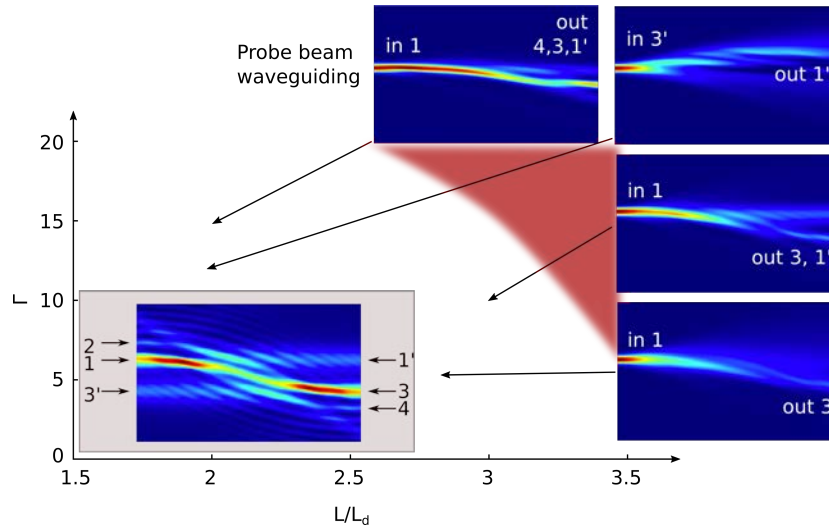
Figure 6.3: Nonlinear interactions of counterpropagating Airy beams with opposite bending directions and their waveguiding effect. Gray frame: intensity distribution of the interacting Airy beams in the biased photorefractive medium ( L = 3, \Gamma = 10 ). The other intensity distributions depict the waveguiding of a probe beam through structures photoinduced by cross-coupling of both Airy beams for various (\Gamma, L) -parameters. In the red zone, no waveguides induced by both interconnecting beams have been observed.
