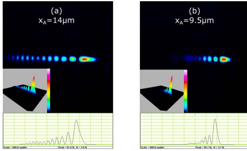
Figure 2.9: Observation of the SLM-generated Airy beam at the input side of the crystal with a CCD camera (20-times magnification). Intensity distribution and profile of (a) the largest generated Airy beam ( x_A = 14 \mu\text{m} ) and of (b) the smallest generated Airy beam ( x_A = 9.5 \mu\text{m} ) using the experimental setup of Fig. 2.8.
