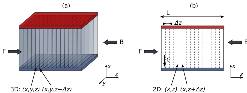
Figure C.1: Interaction scheme of counterpropagating beams in a biased photorefractive medium (a) in 3D and (b) in 2D (used for the numerical calculation in this thesis).
