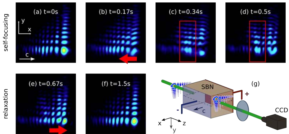
Figure 6.4: Self-focusing of an 2D-Airy beam in a biased photorefractive crystal, with x_A = 11 \mu\text{m} , P_A = 50 \mu\text{W} , L = 1 \text{ cm} and U_{SBN} = 4 \text{ kV} . (a)-(f) Intensity profile of the output beam for different times. (g) Schematic propagation setup of an 2D-Airy beam in the SBN-crystal.
