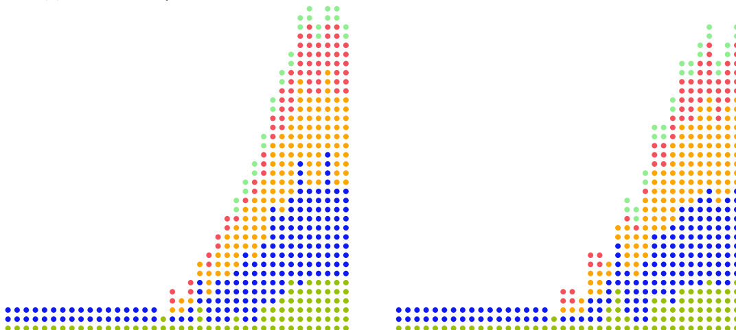
(c) The two bit heaps for 32-bit faithful results, using one DSP block for each multiplication.
