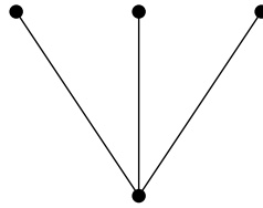
Figure 3.6: The claw graph.
