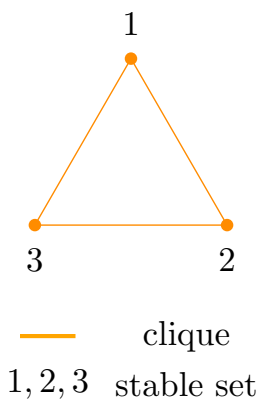
Figure 6.2: A normal covering of K_3 . The clique is in orange (the whole graph) and the three stables are numbered from 1 to 3.
