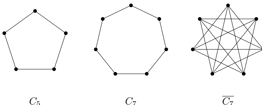
Figure 3.5: From left to right: C_5 , C_7 , \overline{C_7} .
