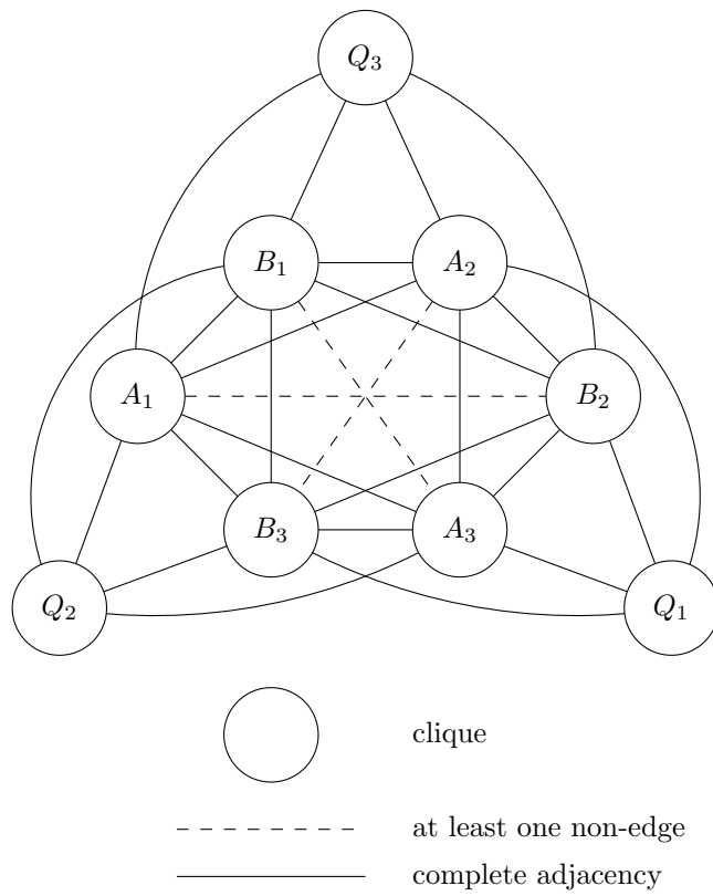
Figure 4.5: General structure of peculiar graphs.
