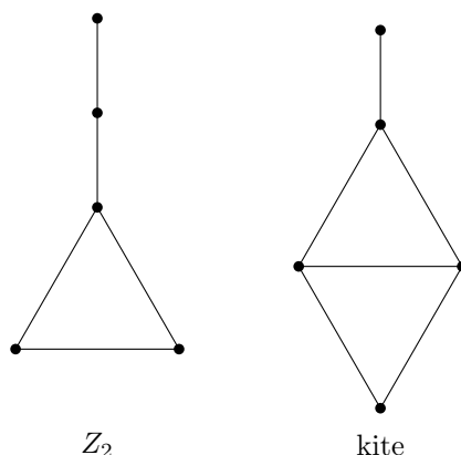
Figure 3.10: The graph Z_2 and the kite.
