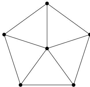
Figure 5.3: The 5-wheel graph.
