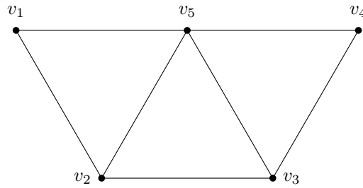
Figure 3.14: The gem graph.
