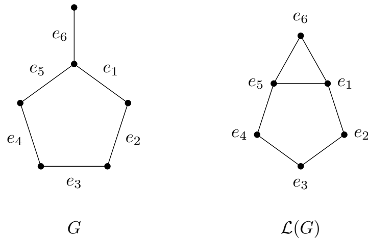
Figure 3.4: A graph G and its line-graph, \mathcal{L}(G) .
