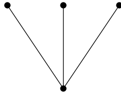
Figure 3.6: The claw graph.
