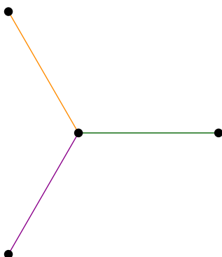
Figure 3.3: Edge coloring example.
