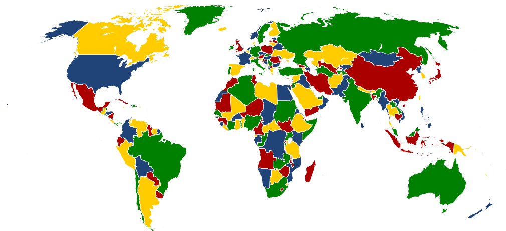
Figure 3.1: A four coloring of the world map
