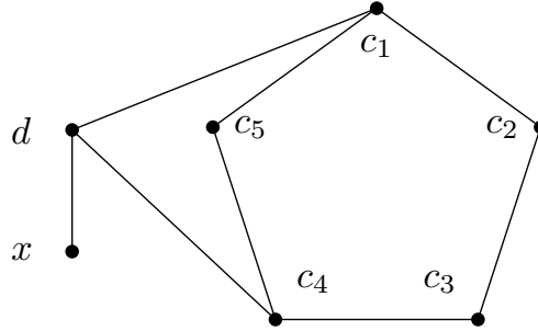
Figure 5.6: The graph G_7 .
