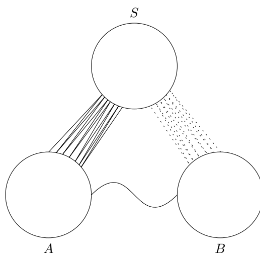
Figure 2.4: Homogeneous set S , with A complete to S and B anticomplete to S .
