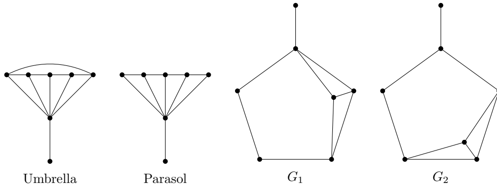
Figure 5.4: From left to right: Umbrella, parasol, G_1 , G_2 .
