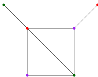
Figure 1.2: Example of an optimal coloring.
