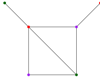
Figure 2.2: Example of an optimal coloring.
