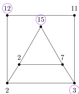
Figure 2.3: Example of an optimal set S . Picked vertices are circled in purple.
