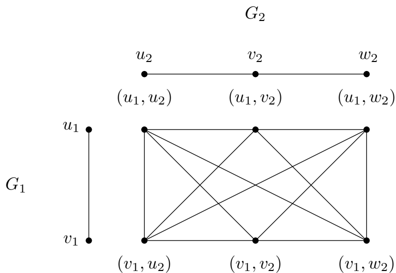
Figure 6.1: The co-normal product of a graph G_1 with another graph G_2 .
