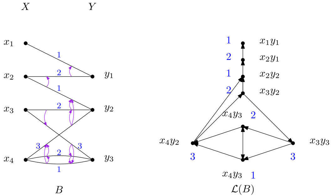
Figure 4.3: An example of Galvin’s theorem with a bipartite multigraph B and its line-graph \mathcal{L}(B) .
