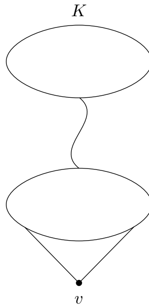
Figure 5.2: The non-neighborhood K of the vertex v .
