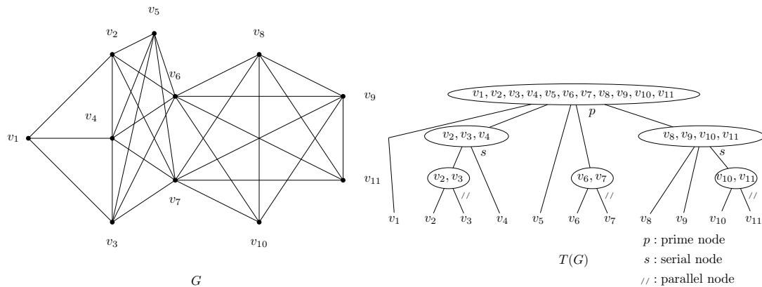
Figure 2.5: A graph G and its modular decomposition tree T(G) .
