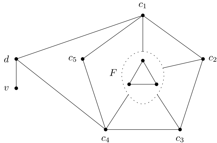
Figure 5.5: The structure of a component in the non-neighborhood of v .
