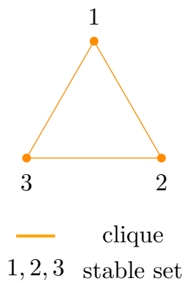
Figure 6.2: A normal covering of K_3 . The clique is in orange (the whole graph) and the three stables are numbered from 1 to 3.
