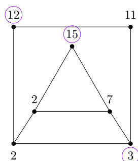
Figure 1.3: Example of an optimal set S . Picked vertices are circled in purple.
