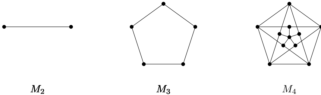
Figure 3.2: The first three Mycielski graphs.
