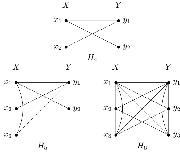
Figure 4.7: The graphs H_4 , H_5 and H_6 .
