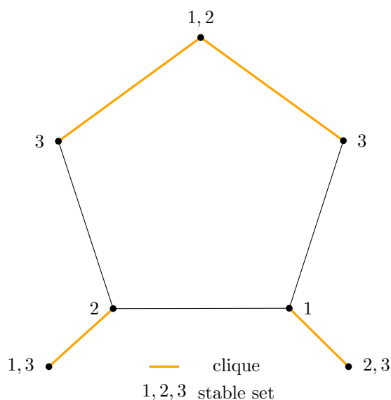
Figure 6.3: A normal graph containing an induced C_5 .
