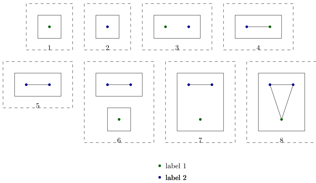
Figure 2.6: Creating a triangle in 8 operations.
