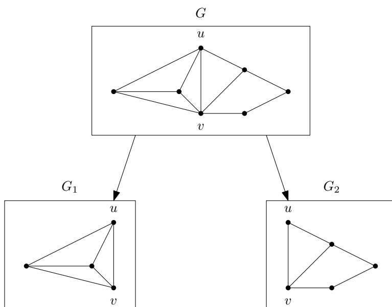
Figure 4.4: A graph G decomposed in graphs G_1 and G_2 by the clique cutset \{u, v\} .
