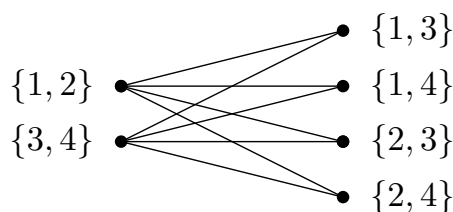
Figure 4.1: K_{2,4} is not 2-choosable.
