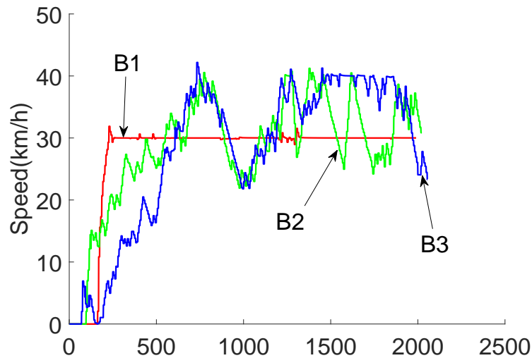
FIGURE 10.17 – Vehicles' speeds in train T_B
