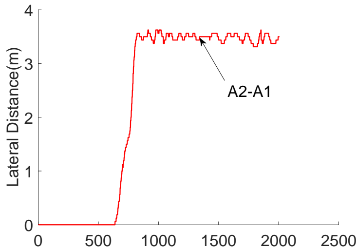
FIGURE 9.6 – Lateral distance between V_{A1} and V_{A2}
