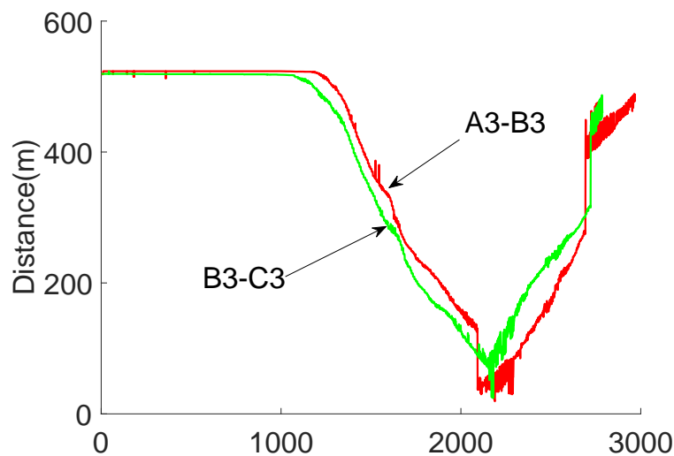
FIGURE 10.34 – Distances between V_{A3} , V_{B3} and V_{C3}
