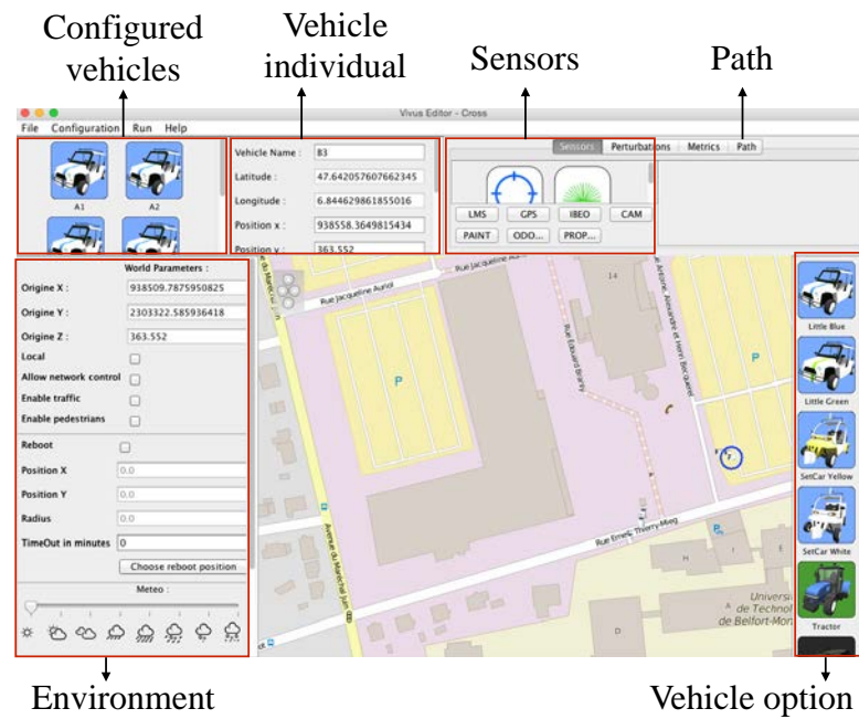
FIGURE 8.4 – VIVUS editor for configure vehicles
