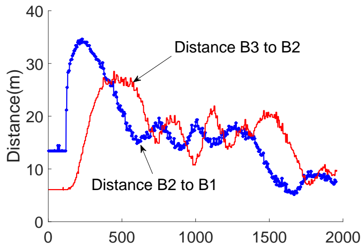
(b) Distances in train T_B
