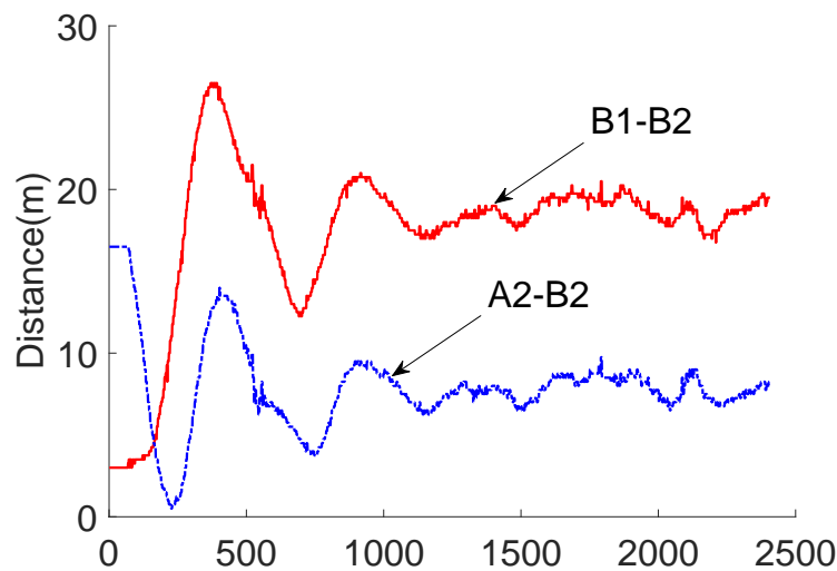
FIGURE 9.11 – Distance from V_{B1} and V_{A2} to V_{B2}
