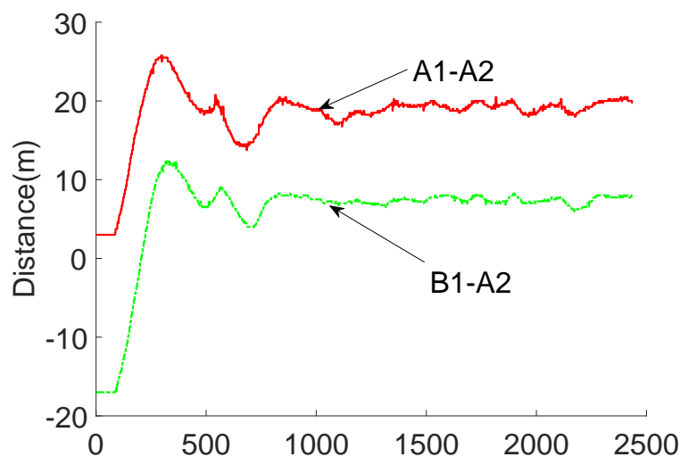
FIGURE 9.9 – Distances from V_{A1} and V_{B1} to V_{A2}
