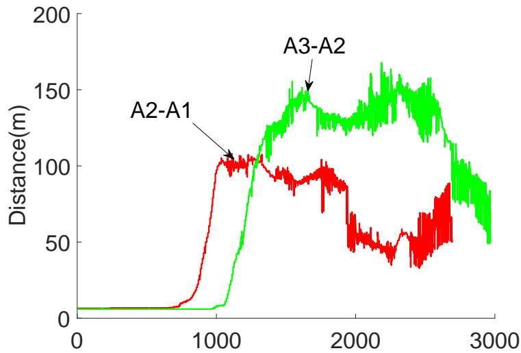
FIGURE 10.35 – Distances between vehicles in train T_A
