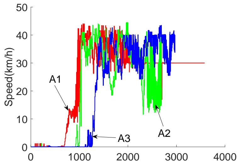
FIGURE 10.36 – Speeds of vehicles in train T_A
