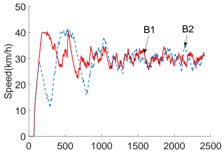
FIGURE 9.14 – Speeds of vehicles in train T_B
