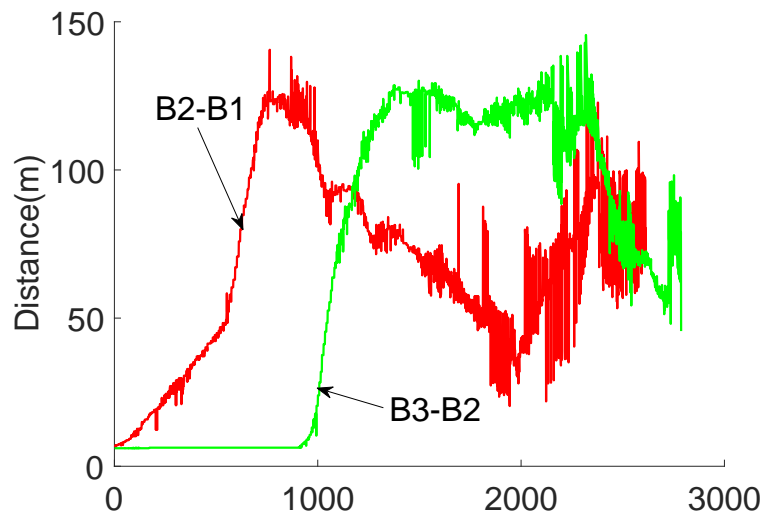
FIGURE 10.37 – Distances between vehicles in train T_B
