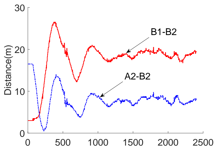
FIGURE 9.11 – Distance from V_{B1} and V_{A2} to V_{B2}
