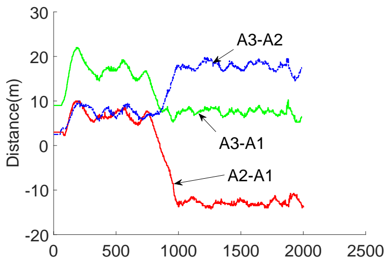
FIGURE 9.5 – Longitudinal distances between vehicles
