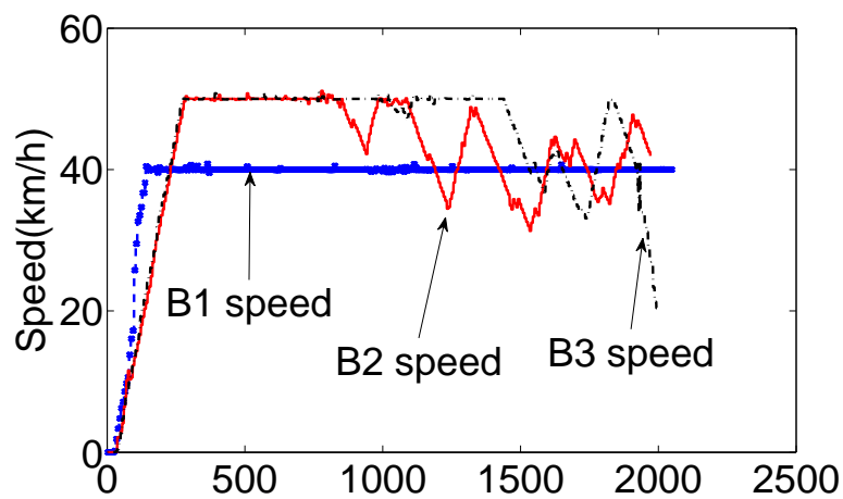
(b) Speeds of train T_B
