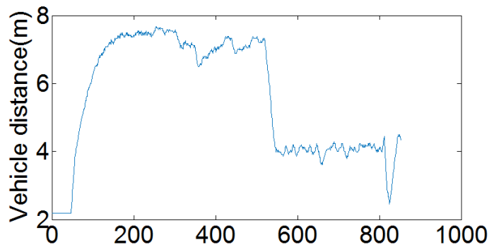
(b) Distance changing in train T_B
