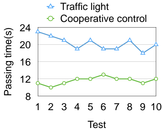
(a) Crossing distance = 7 meters
