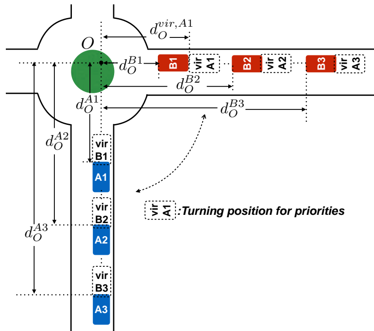
FIGURE 7.3 – Priorities decision
