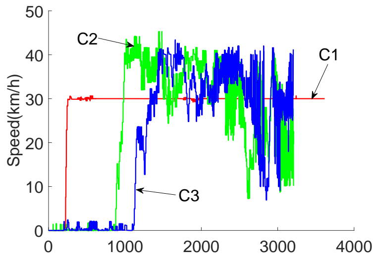
FIGURE 10.40 – Speeds of vehicles in train T_C
