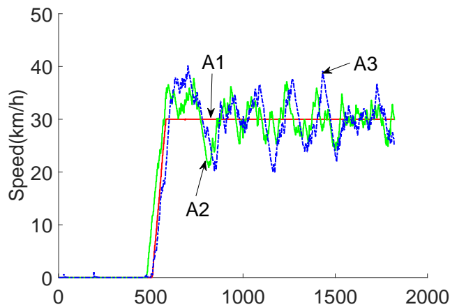
FIGURE 9.3 – Vehicles' speeds
