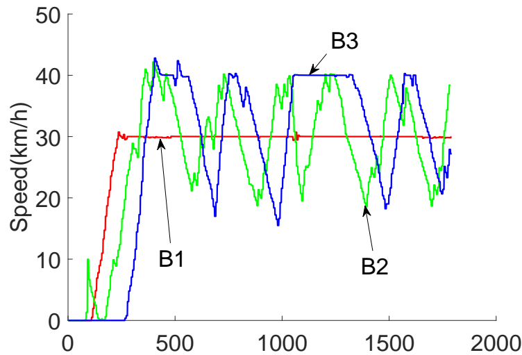
FIGURE 10.28 – Speeds of vehicles in train T_B
