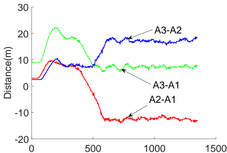
FIGURE 9.17 – Longitudinal distance between vehicles
