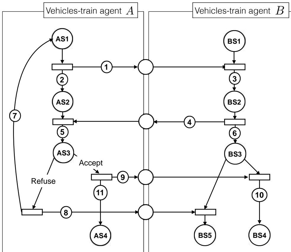
FIGURE 6.5 – Trains agents communication framework
