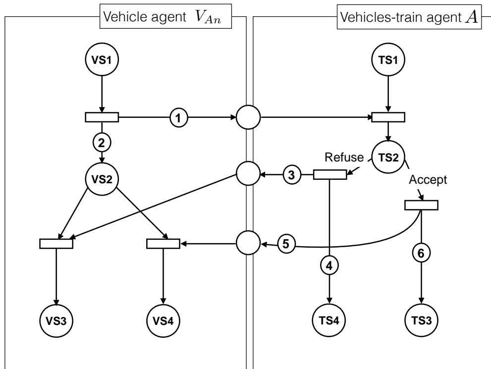
FIGURE 6.4 – Splitting communication framework
