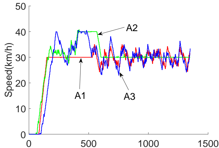
FIGURE 9.18 – Vehicles speed
