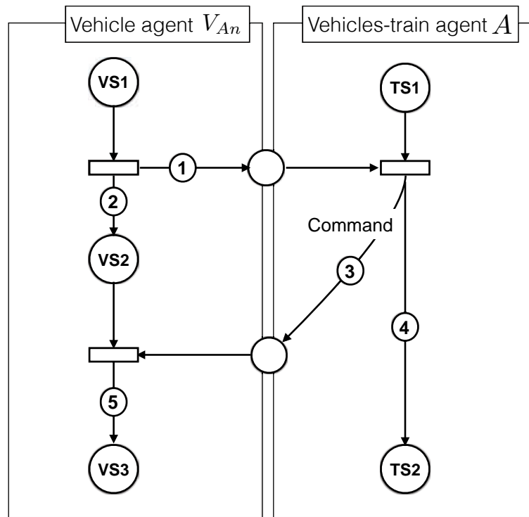
FIGURE 6.3 – Run-in-train communication framework
