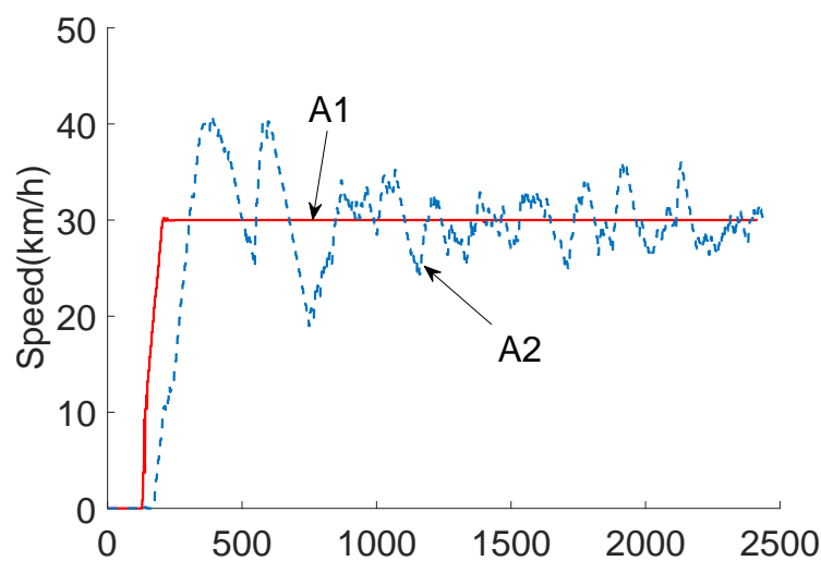
FIGURE 9.13 – Speeds of vehicles in train T_A
