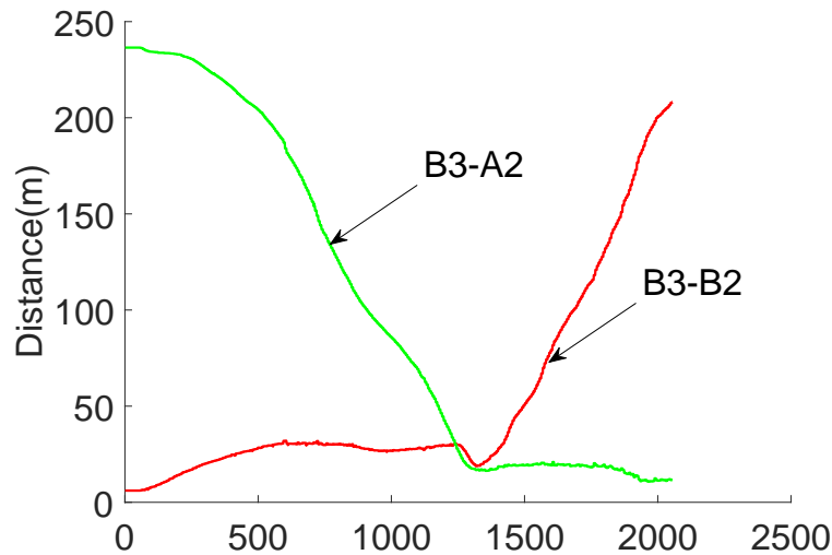
FIGURE 10.15 – Distances V_{B3} with V_{A2} and V_{B2}
