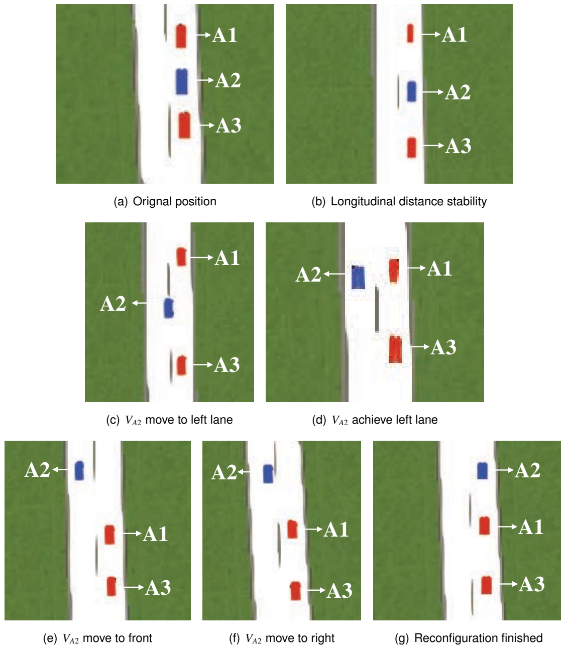
FIGURE 9.15 – Reconfiguration inner-train process
