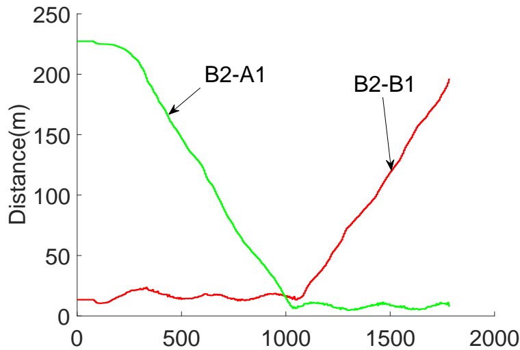
FIGURE 10.24 – Distances between V_{B2} and V_{A1} , V_{B1}
