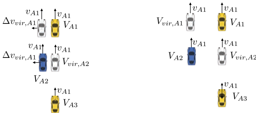
FIGURE 7.7 – Vehicle V_{A2} move to left FIGURE 7.8 – Vehicle V_{A2} arrive suitable position
