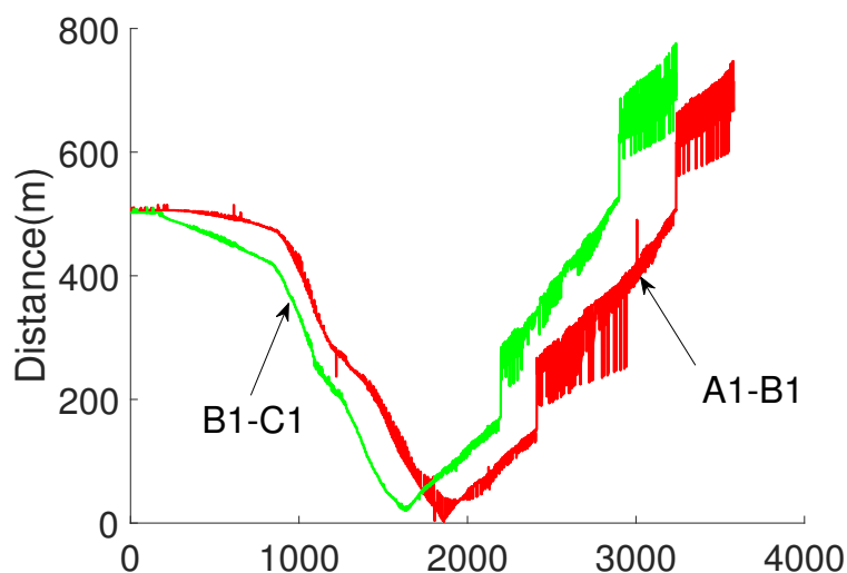
FIGURE 10.32 – Distances between V_{A1} , V_{B1} and V_{C1}
