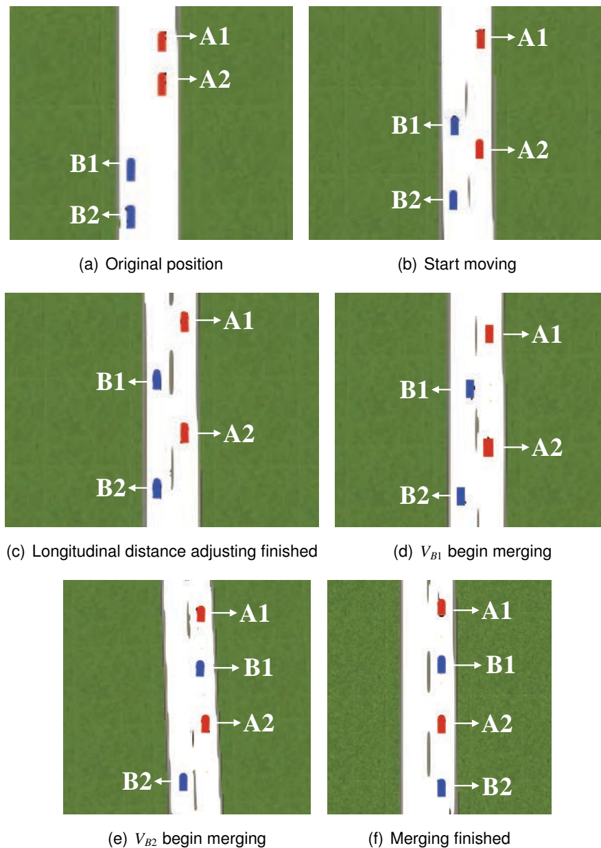
FIGURE 9.8 – Merging process
