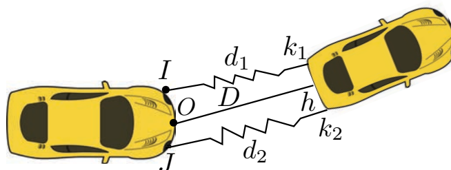
FIGURE 7.47 – Physical interaction model
