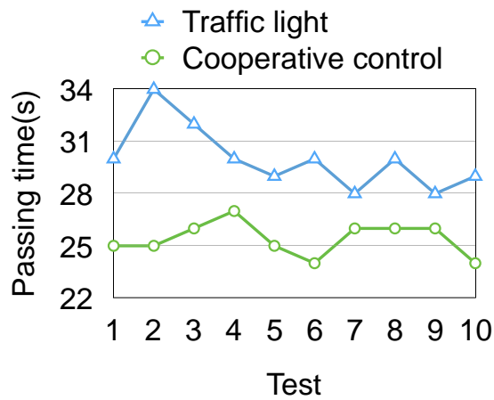
(b) Crossing distance = 18 meters
