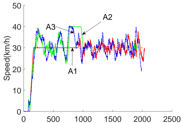
FIGURE 9.7 – Vehicles' speed
