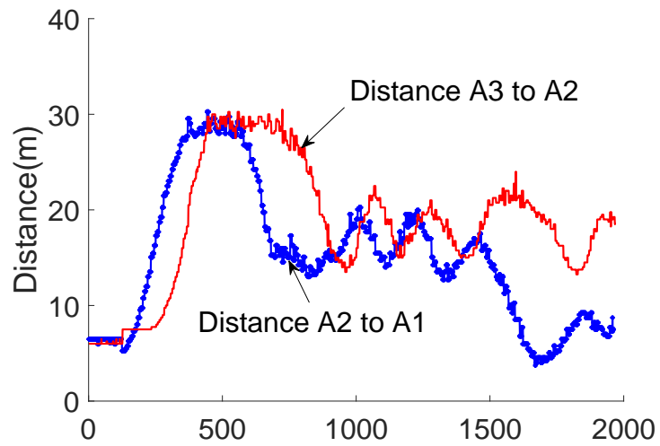
(a) Distances in train T_A
