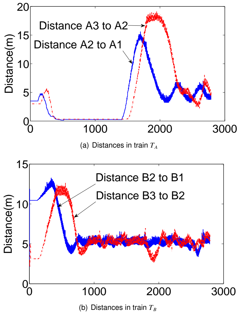
FIGURE 10.8 – Distances under the traffic light control
