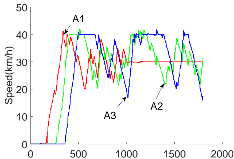
FIGURE 10.27 – Speeds of vehicles in train T_A
