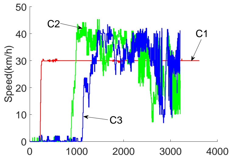
FIGURE 10.40 – Speeds of vehicles in train T_C
