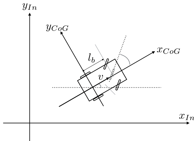
FIGURE 5.4 – Vehicle kinematic model
