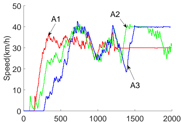
FIGURE 10.16 – Vehicles' speeds in train T_A
