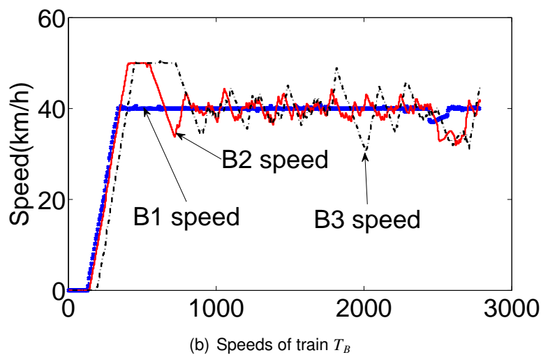
FIGURE 10.6 – Speeds under the traffic light control
