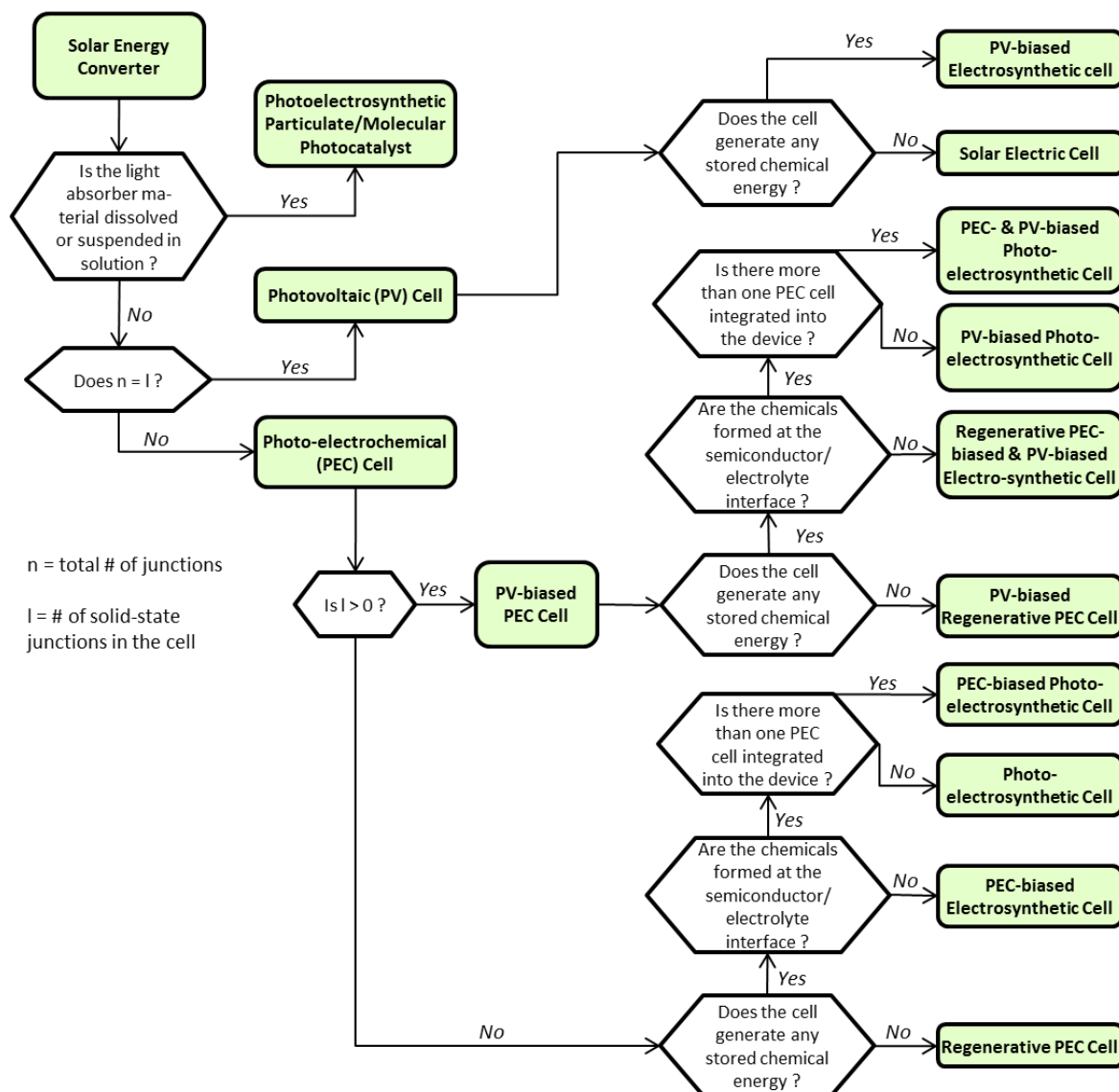
Fig. 7. A taxonomy for the classification of solar energy converters. For a device of interest, identify n (total number of junctions), m (number of semiconductor/electrolyte junctions), and l (number of buried junctions), then proceed through the flow chart to determine the appropriate name for the device. Note that the taxonomy does not address devices designed to use light to drive exergonic processes. Reproduced from Ref. 16 with permission from The Royal Society of Chemistry.
