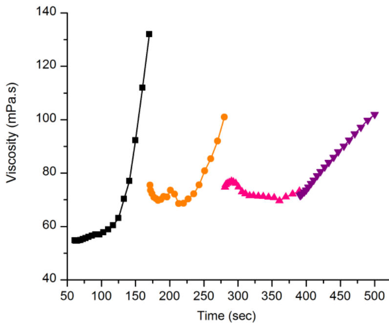
Fig. 67- Viscosity as a function of time, for different shear rates (SR), for the non-diluted ink. Black (squares), \text{SR}=10\text{ s}^{-1} ; Orange (rounds), \text{SR}=100\text{ s}^{-1} ; Pink (triangles), \text{SR}=1000\text{ s}^{-1} ; Purple (inverted triangles), \text{SR}=10\,000\text{ s}^{-1} .
