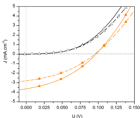
Fig. 105- Example of J-V characteristics of a NiO*-4L-(8) (plain trace) and NiO-4L-(8) (dashed trace), under 1 Sun (AM 1.5 standard) (orange traces, filled triangles) and in the dark (black traces, empty triangles).
