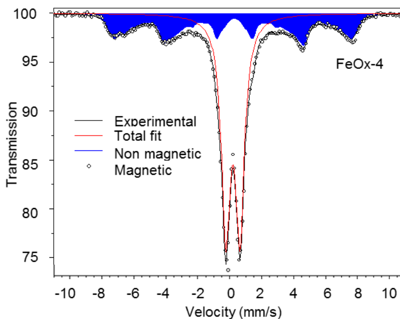
Figure 3.23. Mössbauer spectroscopy realized at room temperature confirms the presence of the maghemite phase only in FeOx-4
