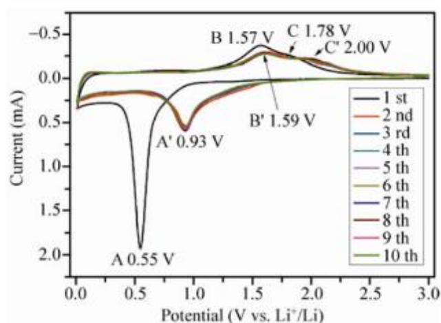
Figure 1.12. Cyclic voltammograms of the \text{ZnFe}_2\text{O}_4 electrode at a scan rate of 0.1 \text{ mV/s} in the voltage range of 0.01\text{V}-3.0\text{V} vs. \text{Li/Li}^+ 81
