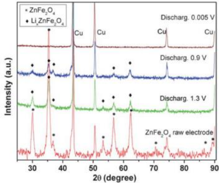
Figure 1.14. Ex-situ XRD at different steps of the first discharge for ZnFe_2O_4 80
