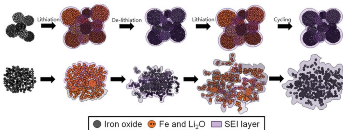
Figure 4.9. Formation of the SEI around iron oxides depending on different particles morphologies 21
