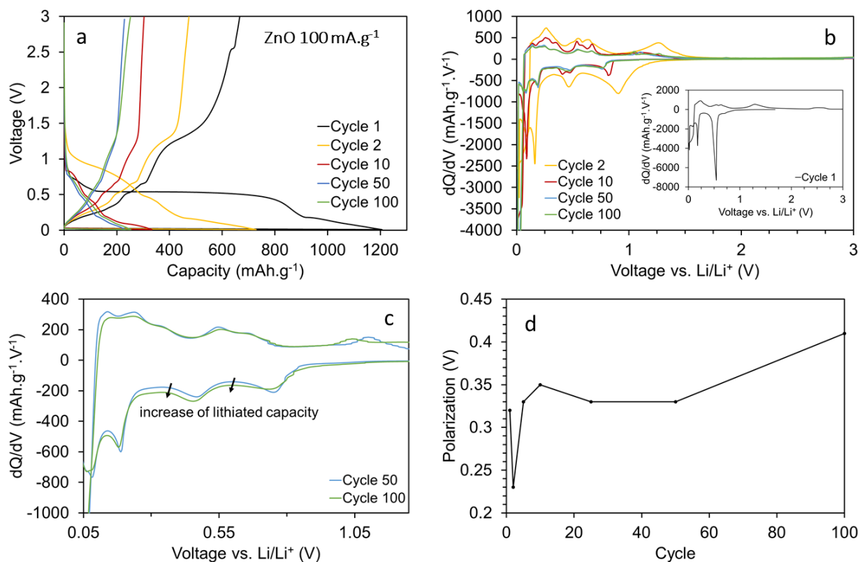
Figure 4.29. Charge/discharge profiles (a), dQ/dV curves (b, c) and polarization (d) for ZnO cycled at 100 \text{ mA.g}^{-1}
