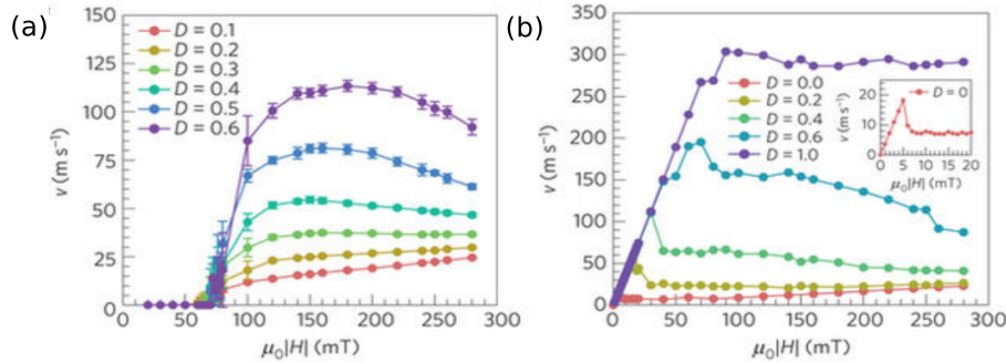
Figure 5.30: Simulated v(H_z) curves in asymmetric Co/Ni wires for different values of the DMI. (a) In the presence of defects. (b) In perfect wires. Taken from Ref. [125]
