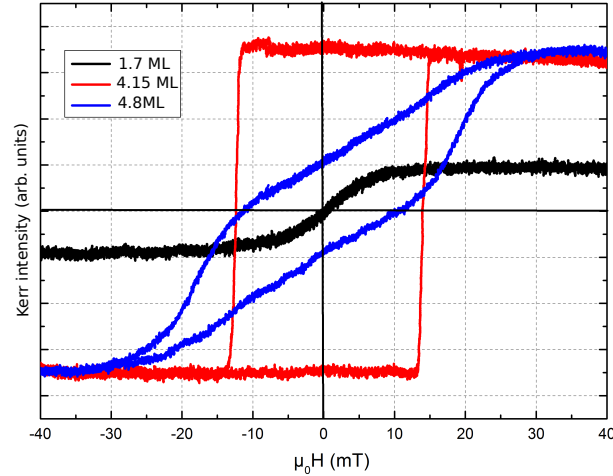
Figure 5.26: Hysteresis loops obtained by focused polar Kerr on different positions along a Co wedge in Au/Co/W(110).
