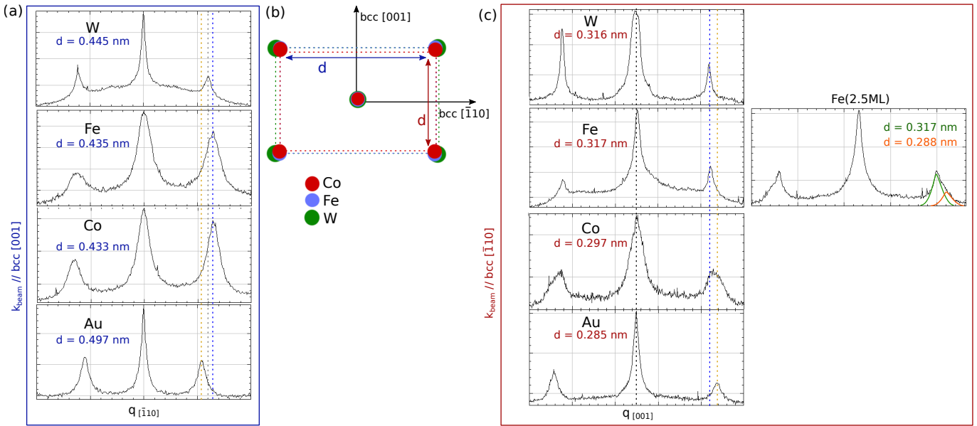
Figure 5.64: (a) RHEED pattern intensity plots for the different materials as a function of the moment q_{[\bar{1}10]} when the electron beam is parallel to the bcc[001] direction. (b) Sketch of the relationship between the W (green), Fe (blue) and Co (red) crystal structures. (c) RHEED pattern intensity plots for the different materials when the electron beam is parallel to the bcc[ \bar{1}10 ] direction
