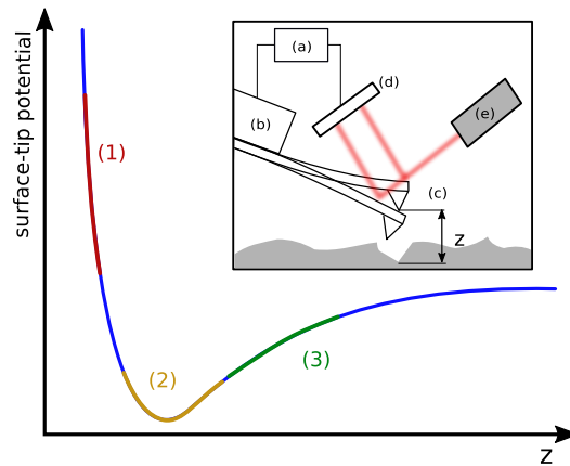
Figure 3.15: Plot of a generic surface potential as a function of the distance from the surface ( z ). ( insertion ) Sketch of the fundamental components of an AFM set-up. (a) Feedback loop electronics (b) High-precision piezoelectric motors for scanning the surface and set the cantilever height. (c) Cantilever with atomically sharp tip. (d) Photo-diode. (e) Laser generator.
