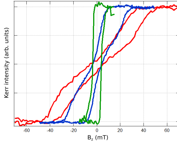
Figure 5.58: Polar Kerr hysteresis loops as a function of an out-of-plane magnetic field for different positions along the Co wedge.(green 3 ML, blue 3.8 ML and red 4 ML)
