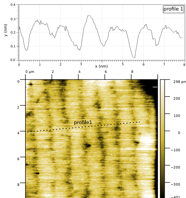
Figure 5.9: AFM microscopy in tapping mode of the surface of a commercial \text{Al}_2\text{O}_3 wafer shows the presence of atomic terraces. The plot shows the surface height along the black line (profile 1)
