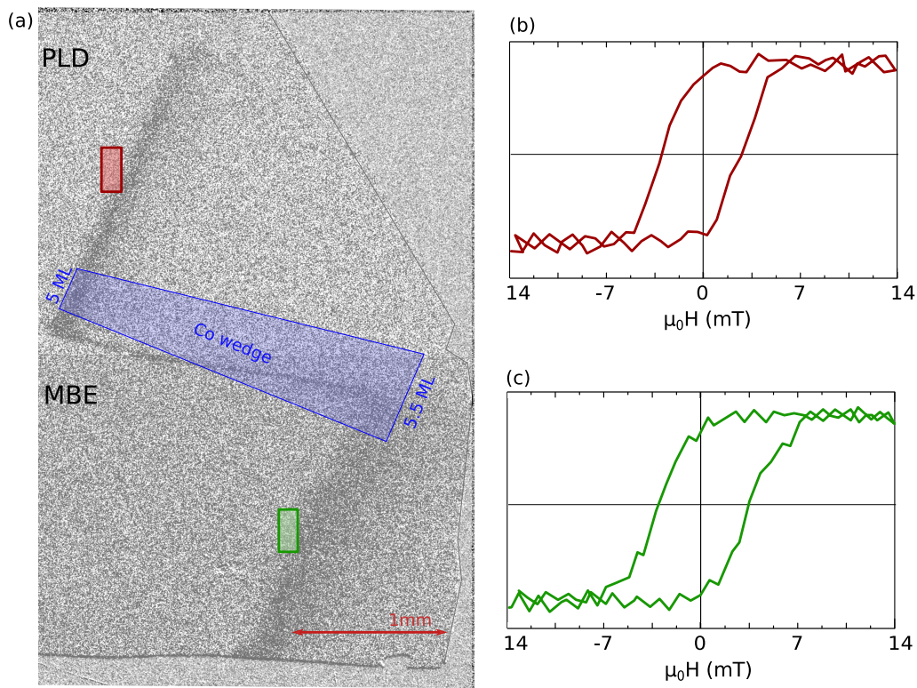
Figure 5.47: (a) Differential Kerr image after the sample saturation with an out-of-plane field. The green and the red rectangles indicate the areas where the polar Kerr hysteresis loops are acquired: (b) (red) in the Au PLD capped area (c) (green) in the Au MBE capped area. The blue trapezium shows the Co thickness along the wedge.
