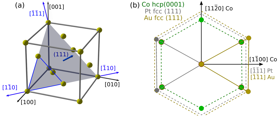
Figure 5.6: (a) Crystal structure of a fcc lattice. The plane (111) is lighted in blue. (b) Epitaxial relationship between the Co hcp (0001) and the Pt fcc (111) surface.
