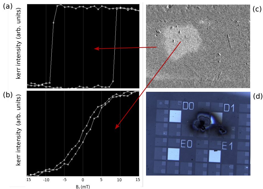
Figure 5.51: (d) Optical image of the consequence of discharges in the PEEM set-up (c) Differential Kerr image of a continuous out-of-plane magnetized system after the application of an out-of-plane field pulse of 10 mT for 10 \mu s. The lighter part is the region modified by the discharges. (b) and (a) Polar Kerr hysteresis loops from the region struck by a discharge and as deposited under the application of an out-of-plane magnetic field. The square loop indicates the presence of an out-of-plane magnetisation whereas the loop in (b) shows that the normal of the sample is no longer the system easy axis. It means that the anisotropy is decreased in the area struck by the discharge.
