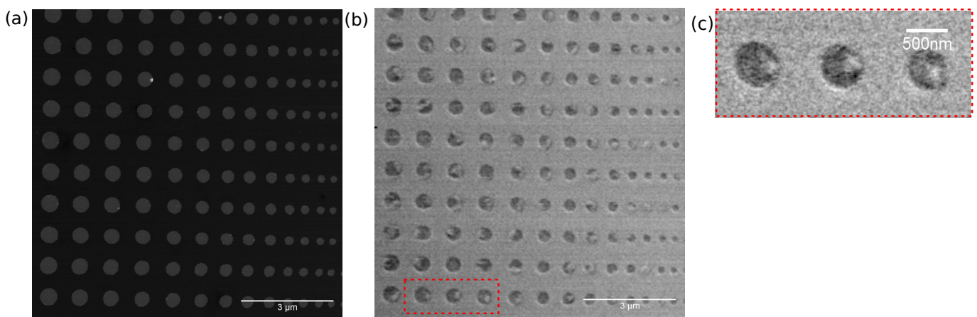
Figure 5.50: (a) AFM Topography image of nanopatterned dots of W\Co\Au. (b) Second pass phase shift MFM image with a 20 nm Cr-Co tip lifted 10 nm ( 10 \mu\text{m} \times 10 \mu\text{m} ) (c) Second pass phase shift MFM image with a 20 nm Cr-Co tip lifted 8 nm ( 3 \mu\text{m} \times 1.2 \mu\text{m} ) on the red zone in (b)
