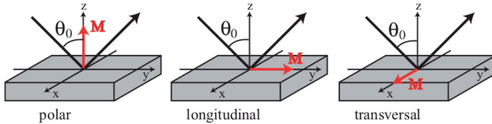
Figure 3.18: Schematic representation of the different Kerr geometries
