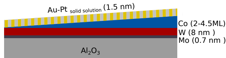
Figure 5.55: Sketch of the W\Co\Au-Pt solid solution structure
