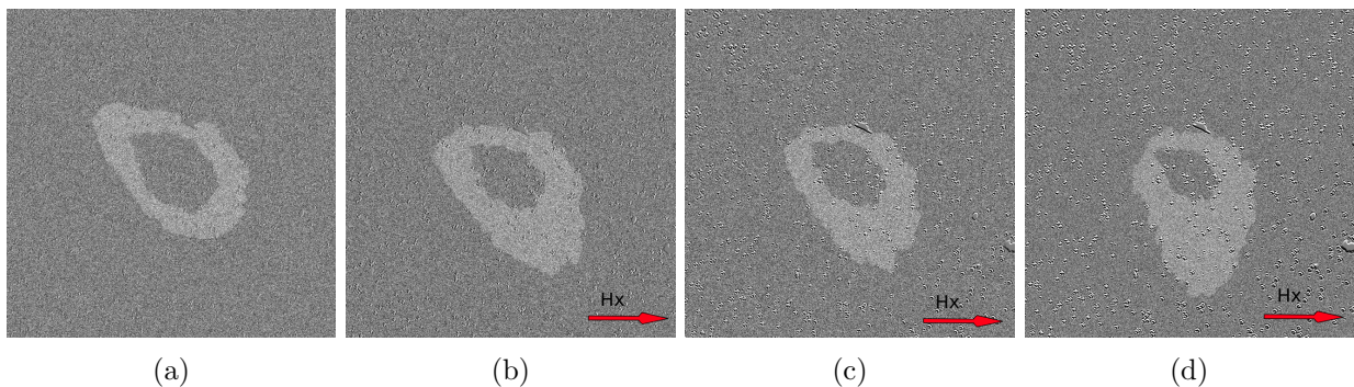
Figure 5.39: Differential Kerr images of the DW expansion of a single magnetic domain with B_{in} along a direction that makes an angle of 37^\circ with respect to the easy axis under two pulses of B_z = 4.6 mT. The pictures are taken with different values of B_{in} [a) = 0 ; b) = 13.9 mT ; c) = 19.2 mT ; d) = 30.1 mT)
