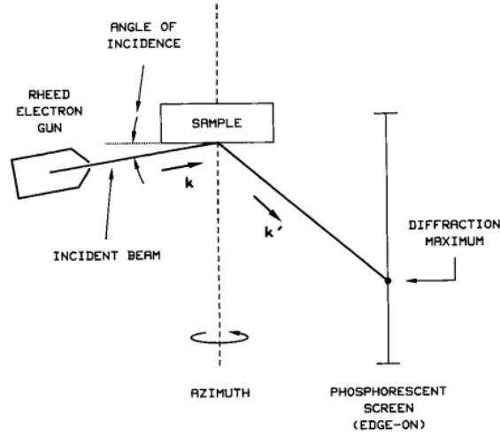
Figure 3.11: [53] Geometry of a RHEED experimental set-up
