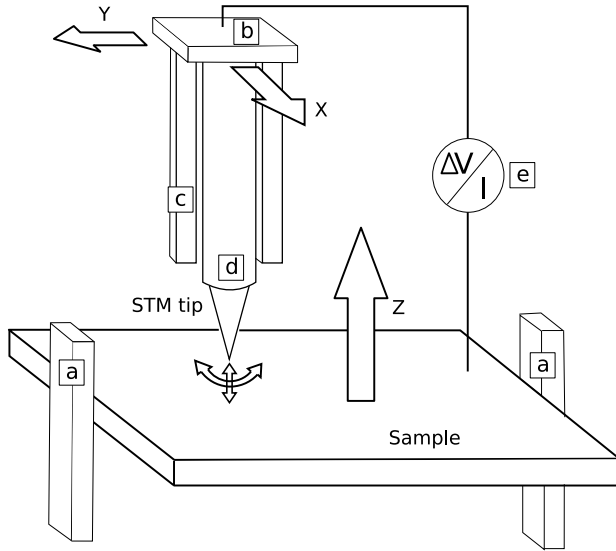
(a) Sketch of tip and sample degrees of freedom in a STM set-up. (a) Two piezo rails moving the sample along the z direction allow the STM tip to approach the surface. (b) Two piezoelectric motors allow to place the tip in different areas of the sample surface ( x, y ) in the figure. (c) Finally two precision piezoelectric motors allow the z motion and (d) the oscillation in the ( x, z ) or ( y, z ) planes. (d) Tip-sample bias voltage and current measurement.
