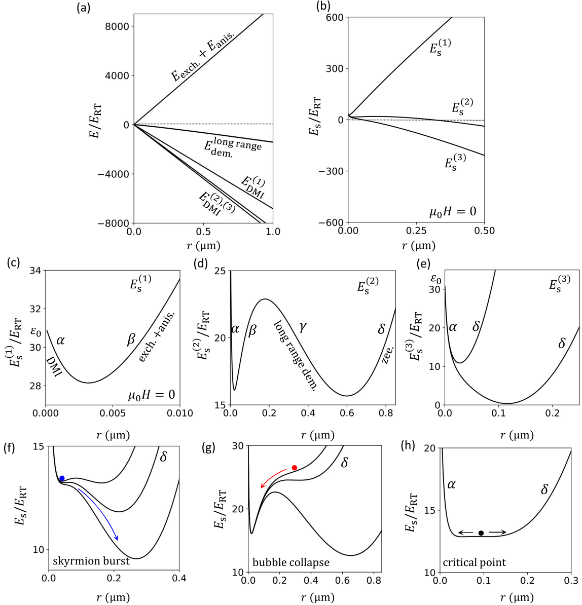
Figure 4.24: (a) Energies versus soliton radius calculated from eq. (4.99) with the same parameters M_s = 1 MA/m, K_u = 1.6 MJ/m, A_{ex.} = 10 pJ/m, t = 0.5 nm, for zero applied magnetic field and D^{(1)} = 2.8 mJ/m 2 , D^{(2)} = 3.46 mJ/m 2 and D^{(3)} = 3.6 mJ/m 2 . (b) Total soliton energies E_s^{(1)} , E_s^{(2)} and E_s^{(3)} calculated with the same parameters as in (a). (c), (d) and (e) Soliton energies E_s^{(1)} , E_s^{(2)} and E_s^{(3)} for applied magnetic fields of respectively \mu_0H = 0 (c), \mu_0H = 0.28 mT (d), \mu_0H = 2 mT and \mu_0H = 7 mT (e). The \alpha , \beta , \gamma , and \delta letters are indicating the different parts of the E_s(r) curve showing a monotonous dE_s/dr variation.
