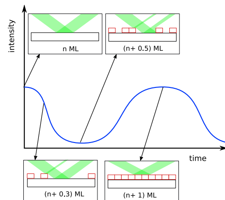
Figure 3.6: RHEED intensity oscillations as a function of the surface order during a layer-by-layer deposition process.
