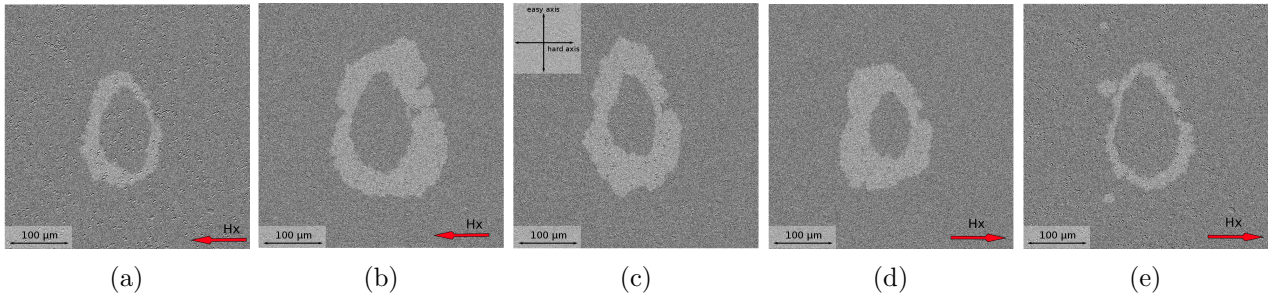
Figure 5.37: Differential Kerr images of DW expansion of a single magnetic domain with B_{in} along the hard axis direction with two pulses of B_z = 4.6 mT. The pictures are taken with different values of B_{in} [a) = -22.5 mT ; b) = -11.4 mT ; c) = 0 mT ; d) = +11.5 mT ; e) = +22.5 mT]
