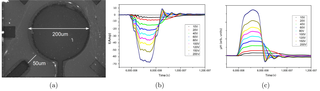
Figure 3.24: (a) Optical image of the micro coil geometry. Lighter contrast : copper layer, darker contrast : Si substrate. (b) Current in the microcoil during the pulse measured with an oscilloscope connected with the electronics. (c) Magnetic field during the pulse measured with a 1mm-diameter coil
