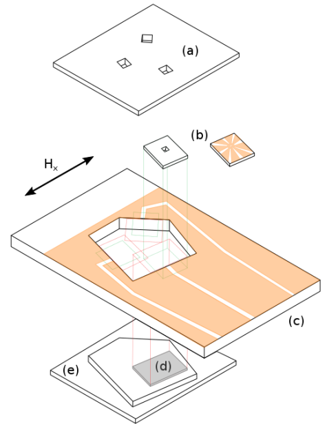
Figure 3.26: Sketch of the set-up designed for mounting the microcoil (b) on the sample surface (d). The green dashed lines show the possible slots for the microcoil and the red lines the relative position of the sample. On the sample-holder base (c) the areas are shown that are covered by copper to guarantee the possible electrical contact for all the microcoil slots. It is done by screwing the element (a) on the base (c) where windows allow the observation of the sample surface. The element (e) is also screwed on the base (c) to guarantee the parallelism of the sample and microcoil surfaces
