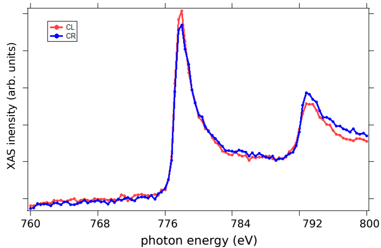
Figure 5.53: XAS spectra at the Co L_2 and L_3 edges with two photon polarisation, (red) circular left (blue) circular right.
