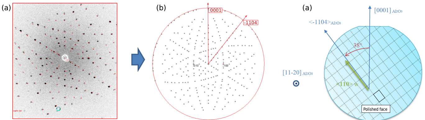
Figure 5.7: (a) Laue diffraction pattern from the sapphire wafer (b) Expected diffraction pattern for a (11 \bar{2} 0) \text{Al}_2\text{O}_3 surface and fit of the experimental data (c) Sketch of the crystallographic directions necessary for the wafer cutting.
