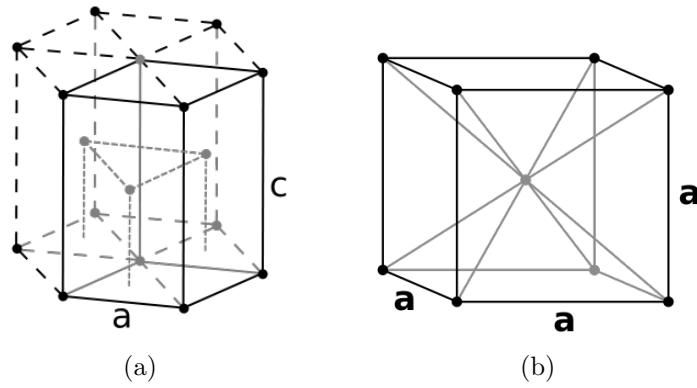
Figure 5.2: Crystal structures: (a) hexagonal close-packed (b) body-centred cubic
