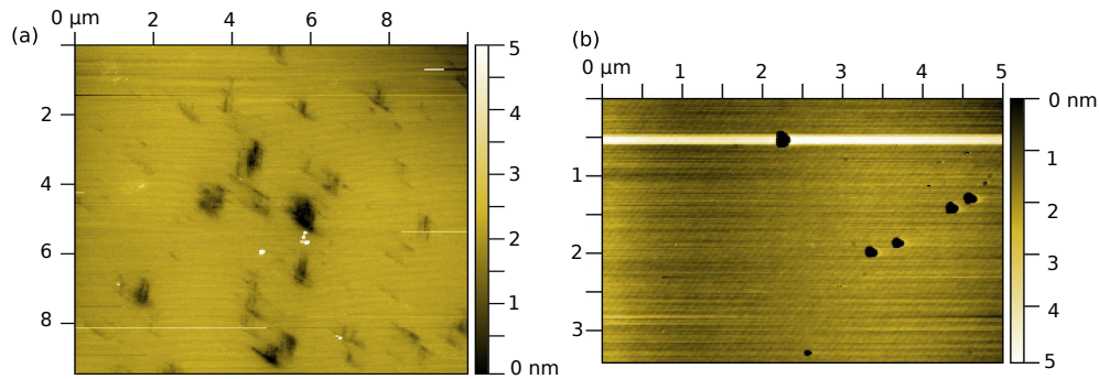
Figure 5.8: AFM microscopy in tapping mode of the surface of commercial \text{Al}_2\text{O}_3 wafers (a) atomically flat surface with the presence of 2-5 nm deep scratches (b) atomically flat surface with the presence of holes deeper than 3 nm.
