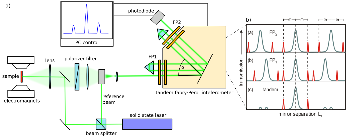
Figure 3.31: (a) Sketch of the main components of a BLS spectroscopy set-up. b) Working principle of a tandem 3x2 Fabry-Perot interferometer
