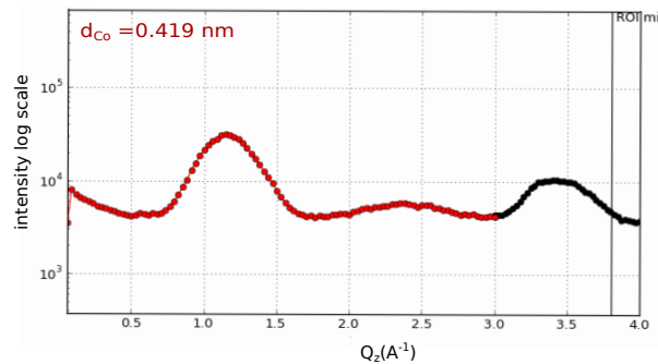
Figure 5.22: Scan along the Q_z direction with fixed values of (Q_x, Q_y) on the Co(\bar{1}20) peak
