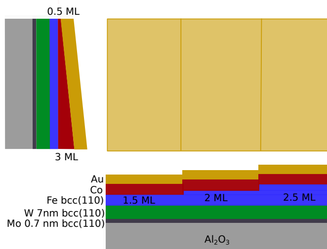
Figure 5.63: Sketch of the W\Fe\Co\Au sample
