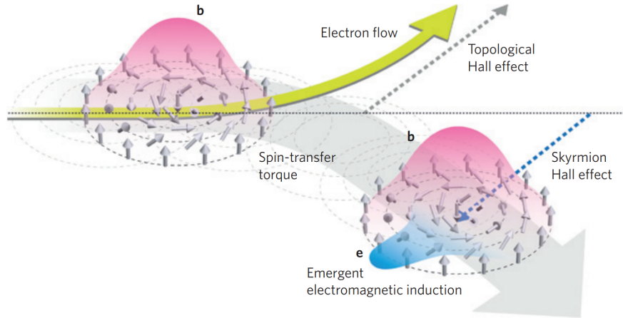
Figure 4.6: "Schematic picture of skyrmion motion and associated physical phenomena under the flow of electrons. Electron current drives the flow of a skyrmion by means of the spin-transfer torque mechanism. Electrons are deflected by the Lorentz force due to the emergent magnetic field \mathbf{b} of the skyrmion. The motion of the skyrmion is accompanied by the time-dependent emergent magnetic field \mathbf{b} (pink), and hence the emergent electric field \mathbf{e} , that is, emergent electromagnetic induction." Taken from [72]
