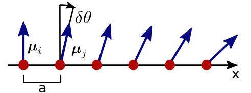
Figure 2.2: Expansion of exchange with \theta to link discrete exchange to continuous theory.
