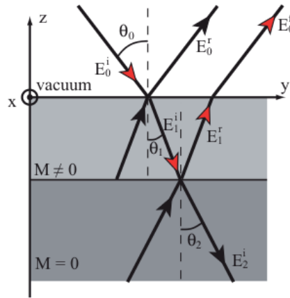
Figure 3.19: Sketch of the system under investigation showing the different incoming and reflected electromagnetic waves
