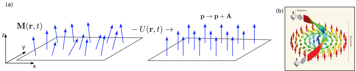
Figure 4.5: (a) Illustration of the effect of the local transformation on the magnetisation felt by a free electron (b) Sketch of the effect of the emergent field from a skyrmionic spin configuration on the motion of a free electron (From ref. [69])
