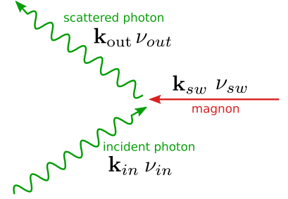
Figure 3.27: Feynman diagram of the Brillouin light scattering phenomenon
