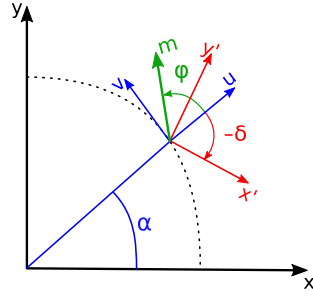
Figure 4.18: Frameworks used for the calculation of the polarisation angle \varphi . The new framework (x', y') corresponds to the coordinate system where the anisotropy matrix (eq. 4.76) takes a diagonal form
