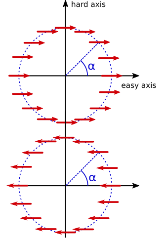
Figure 4.17: Polar plot of the polarisation angles promoted by a biaxial anisotropy
