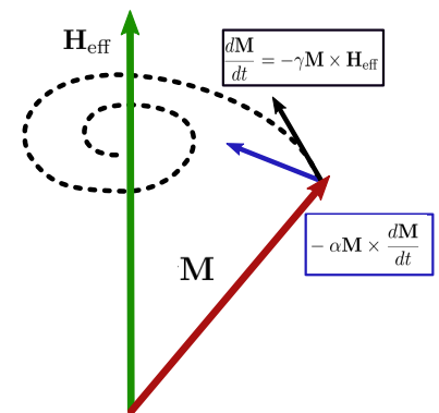
Figure 2.13: Sketch of the vectorial component of eq:5.8
