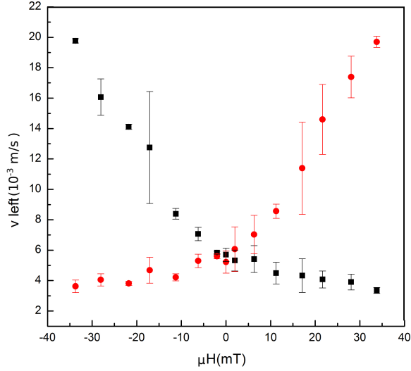
Figure 5.36: Plot of the DW speed versus B_{in} . The red spots are for the right DW whereas the black spots are for the left DW in Fig. 5.35. The experimental error is estimated from the standard deviation calculated from the DW speeds extrapolated from 5 differential Kerr images with the same B_{in} .
