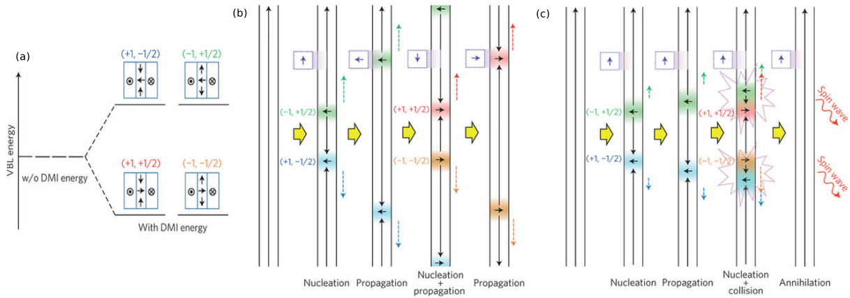
Figure 5.31: [125] (a) Energy splitting of the four BLs when a DMI that promotes clockwise DWs is introduced. The BLs are characterized by a magnetic charge Q = \pm 1 and a topological charge N_{1D} = \pm 1/2 . (b) Propagation of BLs in absence of DMI. (c) propagation of BLs in the presence of DMI.
