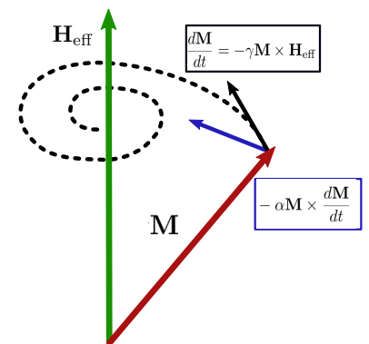
Figure 5.27: sketch of the vectorial component of eq:5.8
