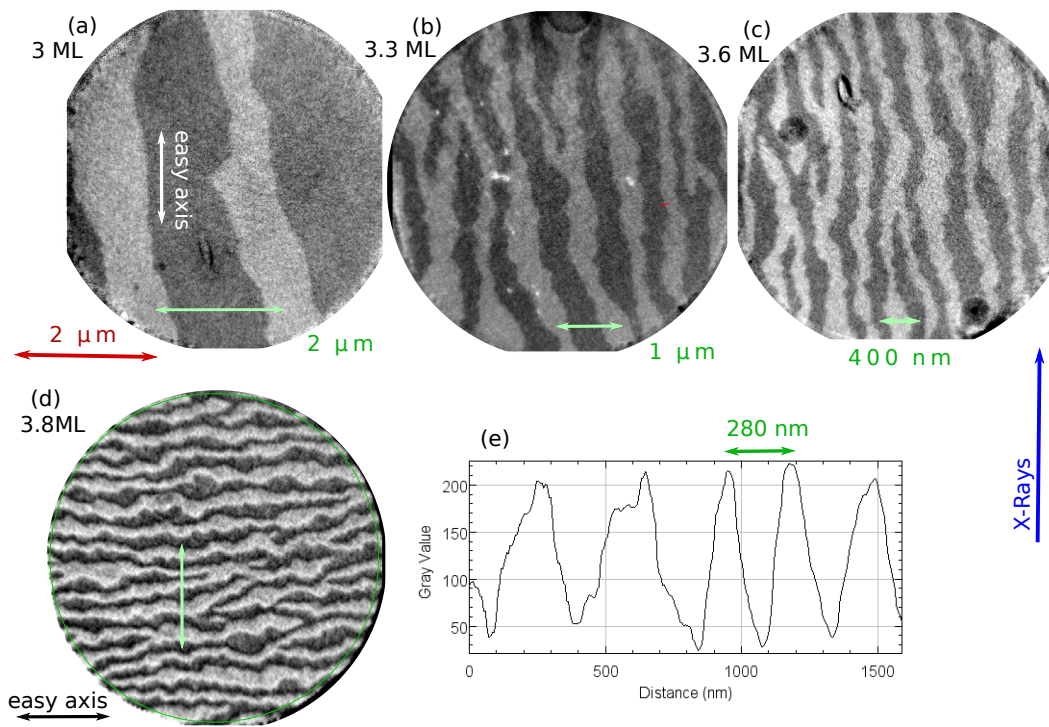
Figure 5.61: XMCD-PEEM images with the x-rays parallel to the easy axis for (a), (b) and (c) and parallel to the hard axis for (d), with a 5 \mu\text{m} field of view. (e) Contrast profile along the green line in Fig. (d).
