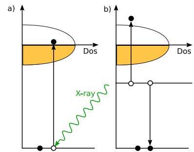
Figure 3.33: a) X-ray absorption and electron transition b) Auger processes
