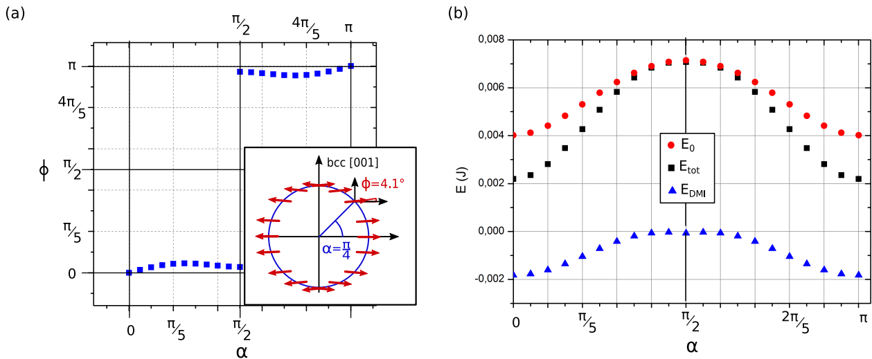
Figure 5.46: (a) Plot and polar plot of the numerical solution of Eq. 4.89 in Sec. 4.3.5 with the magnetic parameters obtained from the BLS measurements (b) Plot of the total energy (black), of the DMI component (blue) and of the subtraction of the two terms (red) for a 1D modulation propagating in the \alpha in-plane direction
