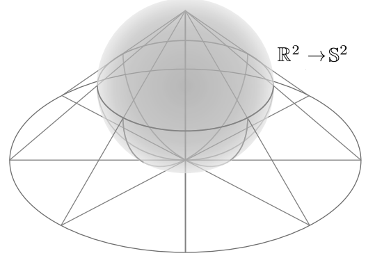
Figure 4.1: Sketch of a stereographic projection from a plane to the surface of a sphere: \mathbf{f} : \mathbb{R}^2 \rightarrow \mathbb{S}^2
