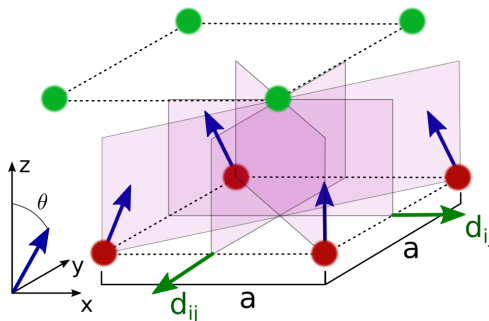
Figure 2.8: Sketch of magnetic moments (blue arrows) in a magnetic square lattice (red) with a C_{4v} symmetry. Four mirror planes (red) pass through the heavy atoms at the interface (green).
