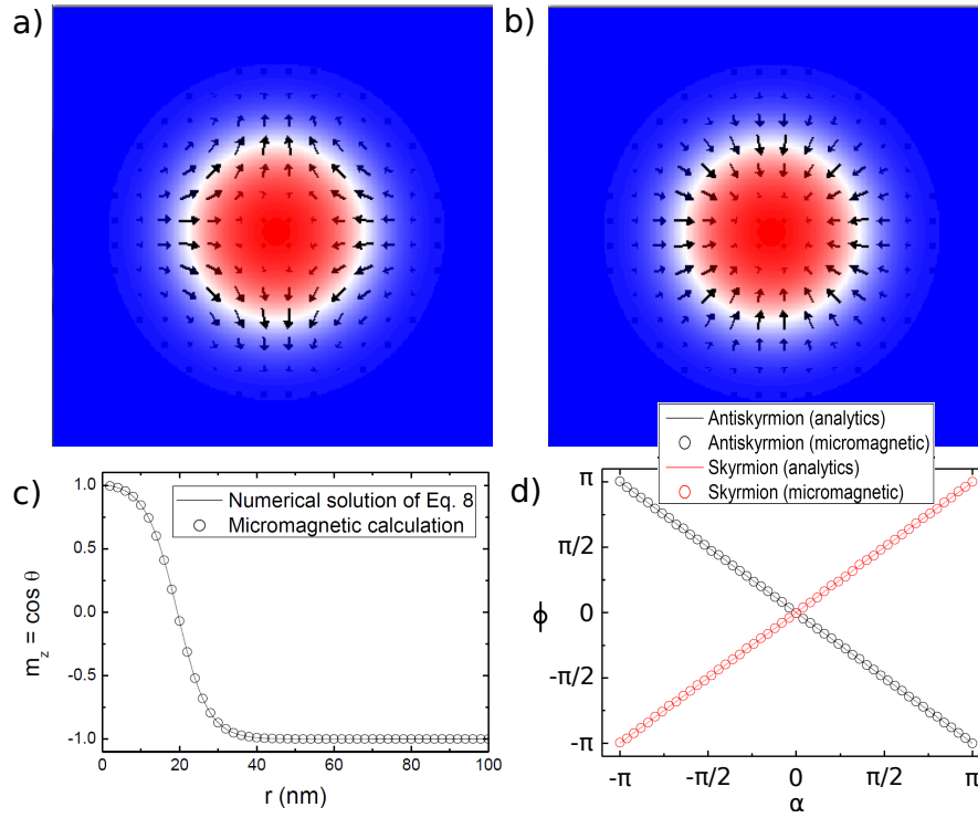
Figure 4.28: Micromagnetic simulations of the magnetisation maps for a skyrmion (a) and an anti-skyrmion (b) (scalebar : 10 nm). The arrows represent the in-plane magnetisation and the color code the out-of-plane magnetisation (red = up, white = in-plane and blue = down). (c) and (d) Comparison between analytic modelling and simulations of the m_z profile and the \phi(\alpha) relationship, for Sk and ASk. In (c) the Sk and ASk profiles are indiscernable.
