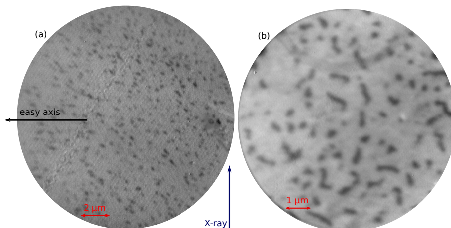
Figure 5.54: XMCD images with the X-Rays perpendicular to the in-plane easy axis with 20 \mu\text{m} (a) and 10 \mu\text{m} (b) fields of view.
