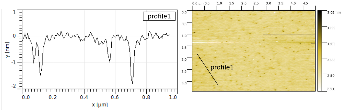
Figure 5.14: AFM microscopy in tapping mode on the surface of a commercial \text{Al}_2\text{O}_3 wafer after the exposure to 15 min. with 20W of \text{O}_2 plasma. (a) The depth and dimensions of the holes are shown in the height plot along the black line (profile 1) (b) It shows the presence of a high density of holes of small size.
