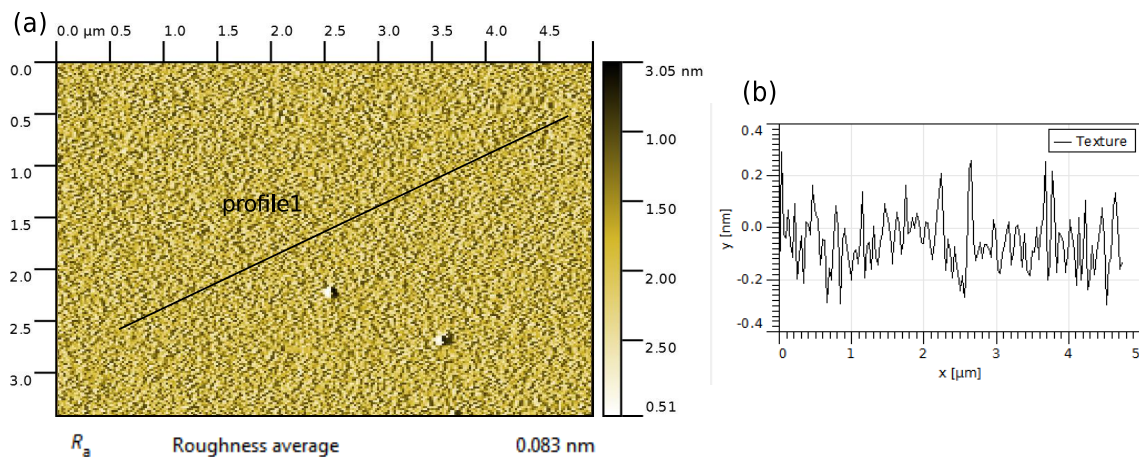
Figure 5.13: AFM microscopy in tapping mode on the surface of a commercial \text{Al}_2\text{O}_3 wafer after the exposure to 15 min. with 10W of \text{O}_2 plasma. (a) The surface is atomically flat and without atomic terraces for a wide area 5 \times 3.5 \mu\text{m}^2 . (b) The height plot along the black line (profile 1) shows surface modulations of \pm 0.2 nm
