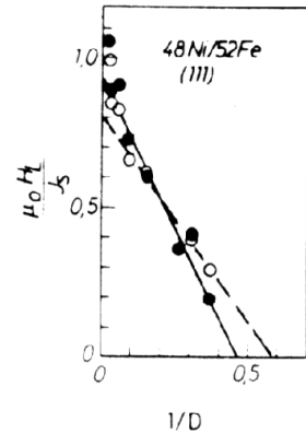
Figure 2.10: Historical example of the 1/t behaviour of the interfacial anisotropy in pitaxial 48Ni/52Fe (111) films [36]
