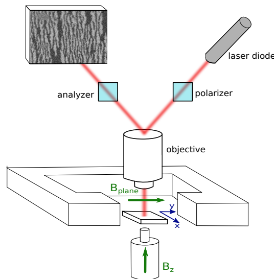
Figure 3.23: Sketch of the set-up assembled on the Kerr microscope stage for the domain wall manipulation
