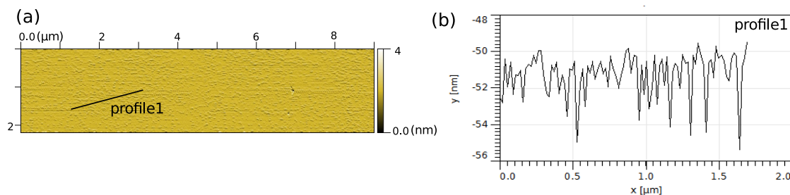
Figure 5.11: (a) AFM microscopy in tapping mode of the surface of a commercial \text{Al}_2\text{O}_3 wafer after the modified RCA protocol with \text{H}_2\text{SO}_4 + \text{H}_2\text{O}_2 18+4 min exposure time. The surface presents a high density of small holes. (b) The size and the depth of the holes is shown in the height plot along the black line (profile 1)
