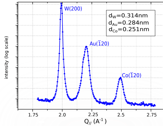
Figure 5.20: GIXRD measurements performed scanning the momentum transfer parallel to the surface plane, along the bcc(001) direction
