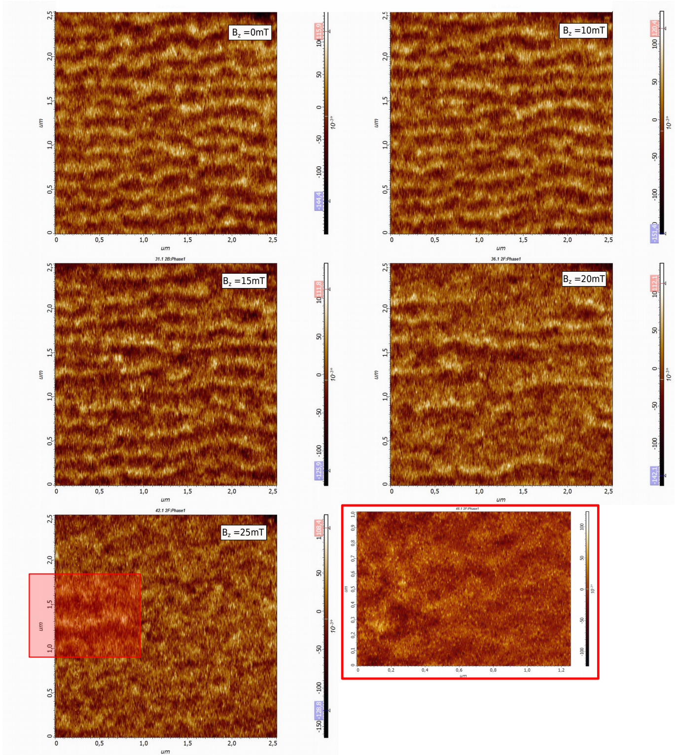
Figure 5.59: The phase shift of the MFM cantilever during the second pass in a 2.5 \times 2.5 \mu\text{m}^2 zone as a function of an out-of-plane magnetic field. The red profile in the bottom left image indicates the area where the bottom right image is taken.
