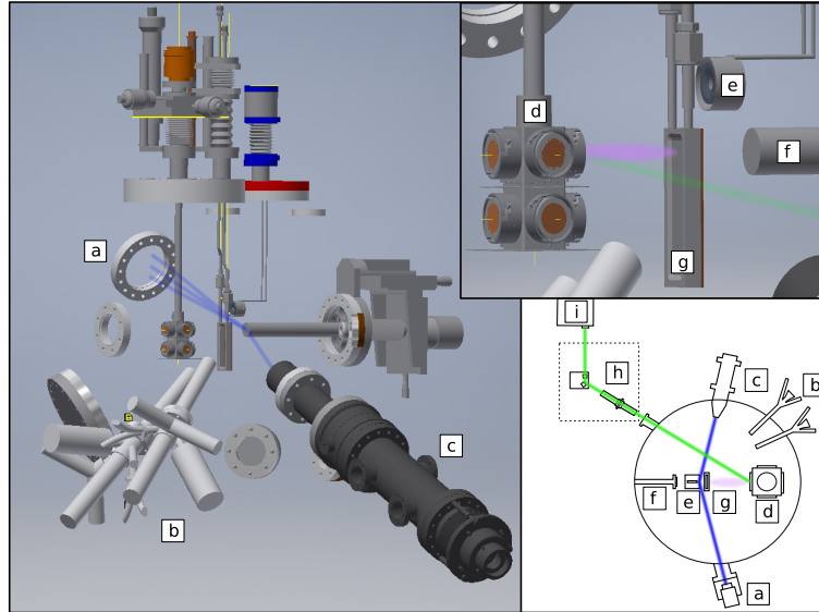
Figure 3.3: Ribber chamber experimental set-up. (blue line) electron beam trajectory for RHEED spectroscopy; (green line) laser trajectory (violet line) plasma plume. (a) RHEED fluorescent screen (b) MBE evaporators (c) RHEED electron gun (d) targets holder (e) quartz micro balance (f) sample holder (g) mask (h) laser optics (i) laser
