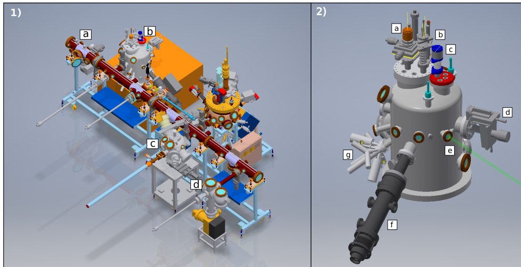
Figure 3.1: (1) Sketch of the complete Ultra High Vacuum system. (a) pre-lock chamber (b) Riber chamber (c) analysis chamber (d) STM chamber. (2) Riber chamber: (a) target holder manipulator, step-motors and cooling system (b) mask step-motor and cooling system (c) quartz micro balance manipulator and cooling system (d) sample holder manipulators, oven and thermocouple connections (e) laser window (f) RHEED electron gun (g) MBE evaporators
