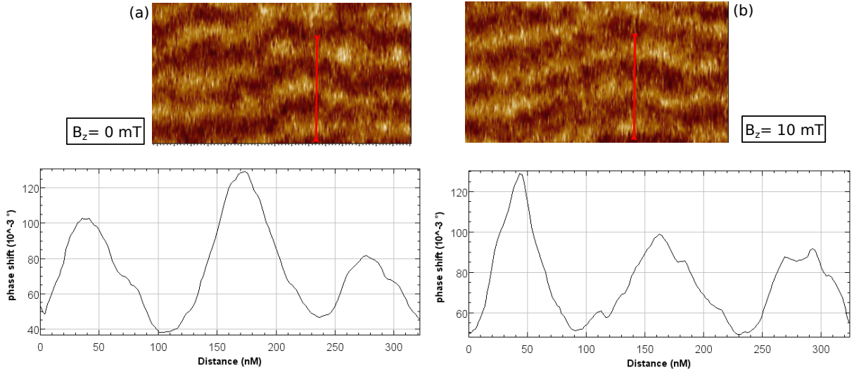
Figure 5.60: MFM images under the application of (a) B_z = 0 and (b) B_z = 10 mT. The plot shows the phase shift variation along the red line in the MFM images.
