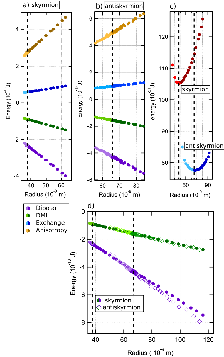
Figure 4.32: Magnetic energies of a skyrmion (a) and an anti-skyrmion (b) as a function of the radius for a given set of magnetic parameters ( M_s = 1.25 \cdot 10^6 A/m, A_{ex} = 16 pJ/m, K_{eff} = 2 \cdot 10^5 J/m 3 , D = 2.0 mJ/m 2 ). (c) Total energy for a skyrmion (red) and an anti-skyrmion (blue) as a function of the radius. (d) Comparison between the DMI (green) and the dipolar interaction (violet) for a skyrmion (dots) and an anti-skyrmion (squares) as a function of the radius. The vertical dotted lines in all panels correspond to the equilibrium radius of Sk and/or ASk
