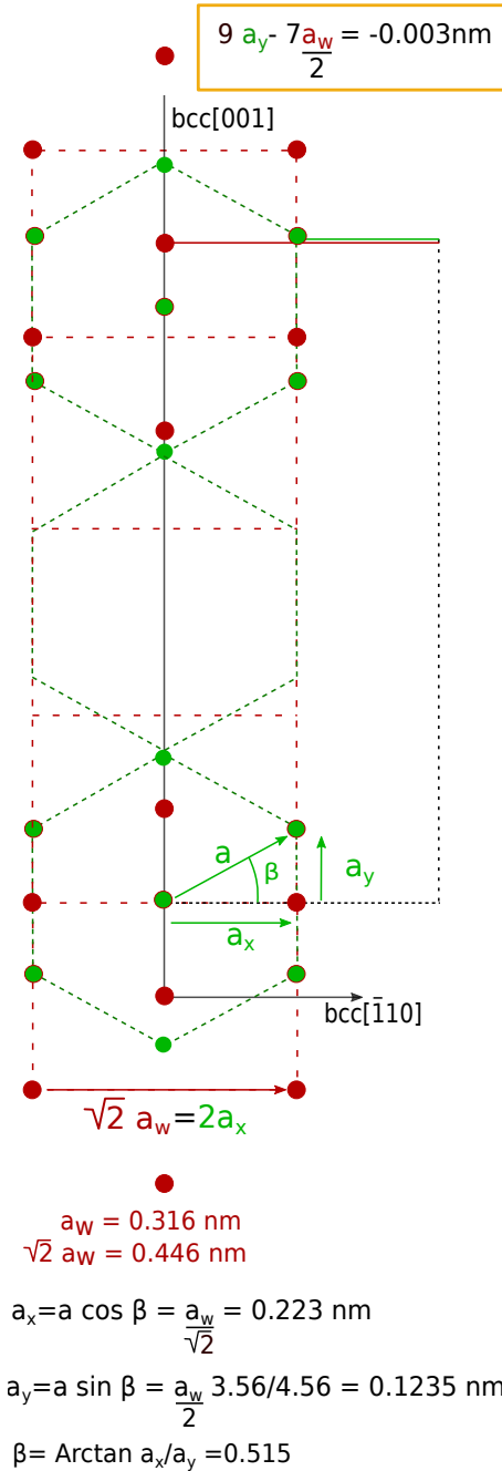
Figure 5.16: Sketch of the complete Co/W superstructure.
