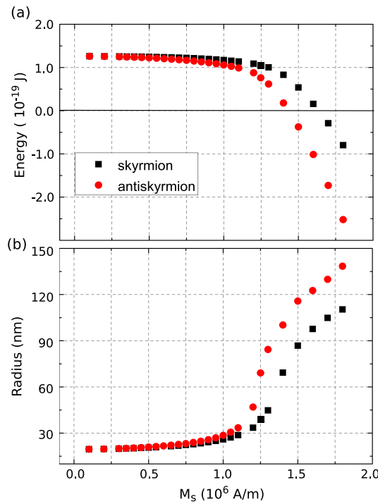
Figure 4.30: Energy (a) and radius (b) of a skyrmion (black) and an anti-skyrmion (red) as a function of the spontaneous magnetisation M_s . The simulations are performed in circular dots of 400 nm diameter and 1 nm thickness with a fixed out-of-plane effective anisotropy K_{\text{eff}} . A_{\text{ex}} = 16 pJ/m K_{\text{eff}} = 2 \cdot 10^5 J/m 3 D = 2.0 mJ/m 2 )
