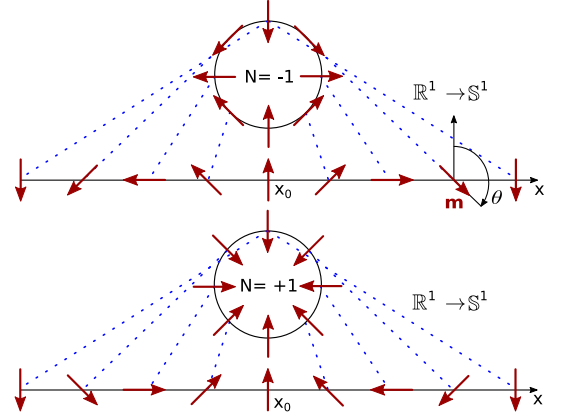
Figure 4.2: Sketch of a stereographic projection from a line to a circle: \mathbf{m} : \mathbb{R}^1 \rightarrow \mathbb{S}^1 . The red arrows indicate the direction of the magnetisation field. The shown magnetic configurations, known as a 360^\circ domain wall, have an integer topological number.
