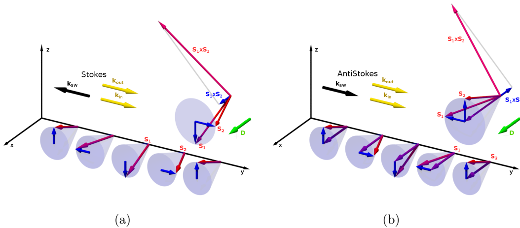
Figure 3.30: Sketch of the BLS phenomenon: ( bottom ) surface SW propagating along the y direction, red arrow = spin located at the atom position, blue arrow = spin projection on the plane (y,z). ( top-left ) direction of the wavevectors in the S (a) and AS (b) processes, yellow arrow incoming and outgoing photon wavevectors, black arrow SW wavevector. ( top-right ) representation of the vectorial product between two spins during the SW propagation ( green arrow ) and projection along the DM vector ( green arrow ).
