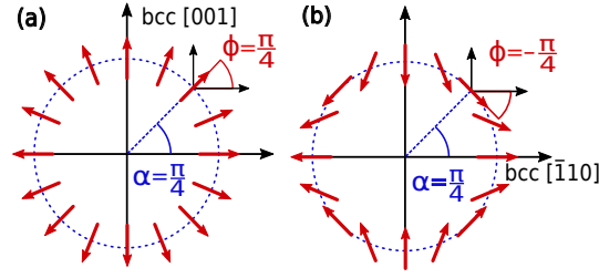
Figure 4.16: Polar plot of the magnetisation direction ( \phi ) promoted by DMI as a function of the in-plane direction of variation \alpha (Eq. 4.63) for different (D_s^{(x)}; D_s^{(y)}) values: (a) D_s^{(x)} = D_s^{(y)} (b) D_s^{(x)} = -D_s^{(y)}
