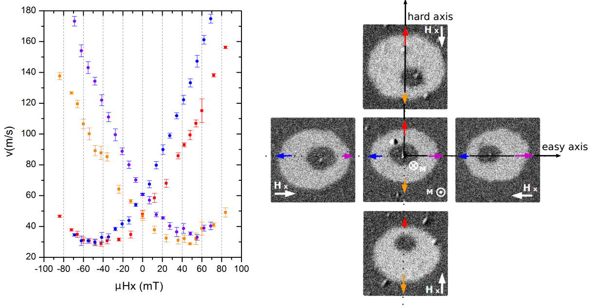
Figure 5.42: Plot of the DW speed as a function of the in-plane field B_{\text{in}} along the easy (blue, violet) and hard (orange, red) axes under the application of a B_z of 60 mT for 20 ns. The differential Kerr images show the DW expansion and the direction of the applied field (white arrows)
