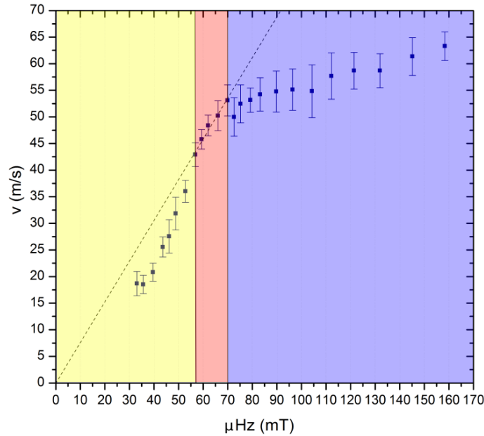
Figure 5.41: Plot of the DW speed as a function of the out-of-plane magnetic field B_z . Three dynamics regimes can be found: (yellow) creep regime, (red) steady flow regime and (blue) soliton motion regime
