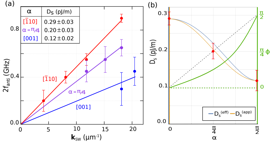
Figure 5.45: (a) S-AS frequency shift ( 2f_{\text{anti}} ) as a function of SW wave-vector ( k_{\text{SW}} ) for different in-plane directions \alpha . The dots are the experimental data and the lines are linear fits yielding the DMI strength ( D_s ). (b) Blue and orange lines : micromagnetic calculated D_s^{(\text{eff})} (Eq.5.38) and D_s^{(\text{app})} (Eq.5.37) as a function of the in-plane directions ( \alpha ); red dots: D strength evaluated from the experimental data; green line: micromagnetic calculated magnetisation direction promoted by DMI (Eq.4.63) as a function of the crystallography directions; dashed line: Néel-like cycloid
