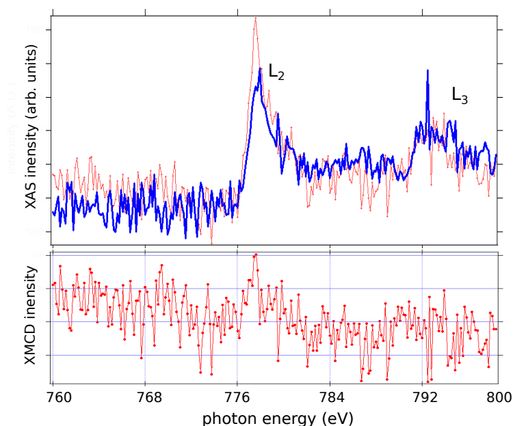
Figure 5.52: XAS spectra with two photon polarisations, (red) circular left (blue) circular right. The XMCD spectrum is obtained by the subtraction of the two XAS spectra.
