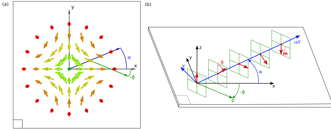
Figure 4.27: (a) Sketch of the magnetisation of an anti-skyrmion in the system plane. (b) Frame for describing the space in circular coordinates (\alpha, r) and for the magnetisation in polar coordinates (\phi, \theta)
