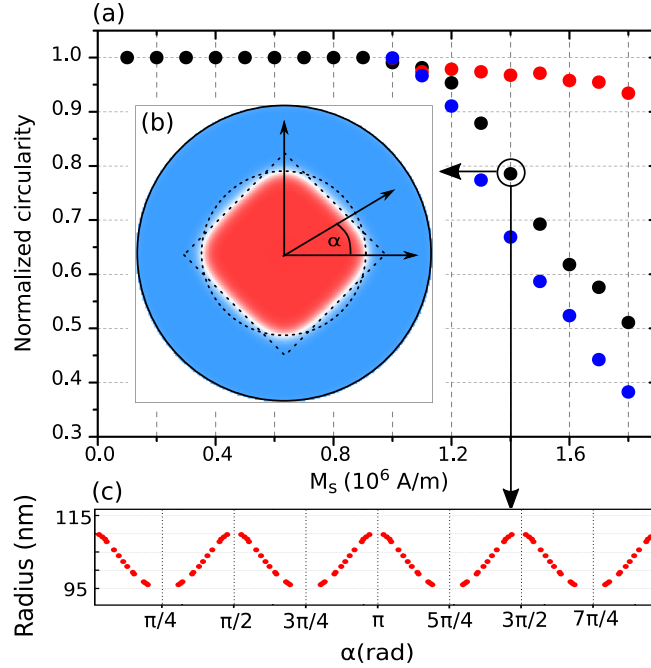
Figure 4.31: (a) Normalized circularity factor C_n as a function of M_s for an anti-skyrmion stabilized in dots with a diameter of 500 nm (blue), 400 nm (black) and 200 (red). (b) Magnetic configuration of an anti-skyrmion ( M_s = 1.4 \cdot 10^6 A/m, A_{\text{ex}} = 16 pJ/m, K_{\text{eff}} = 2 \cdot 10^5 J/m 3 , D = 2.0 mJ/m 2 ) with a sketch that shows the square-circular shape. (c) Radius of an anti-skyrmion as a function of the in-plane angle \alpha
