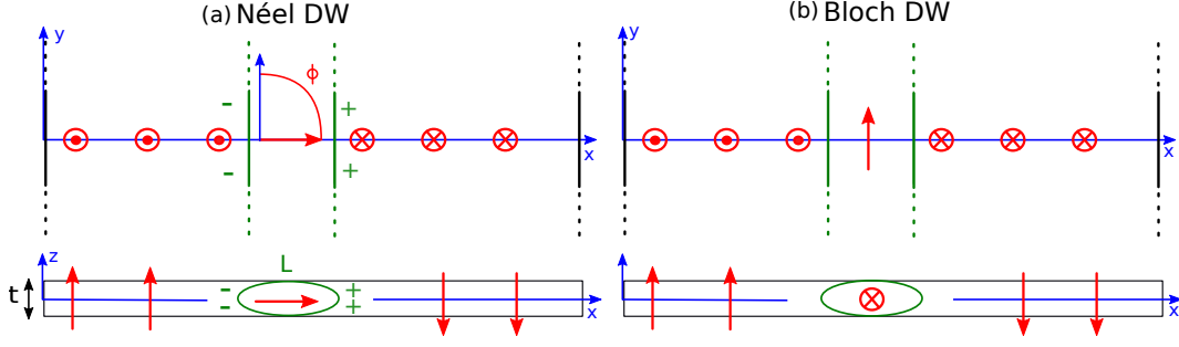
Figure 4.12: (a) Néel DW and (b) Bloch DW in a three dimensional system. (red) magnetisation vectors. (green) demagnetisation ellipsoid and volume magnetic charges.
