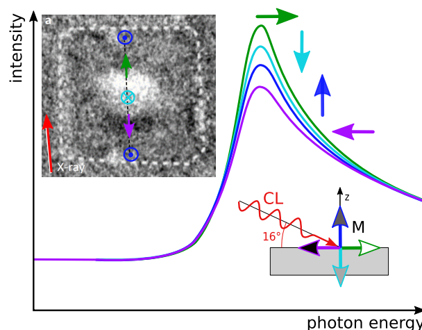
Figure 3.34: Spectra of L_3 edge taken with CL x-rays for different magnetisation directions. insertion ) XMCD-PEEM image of a skyrmion stabilized in a square dot [6].
