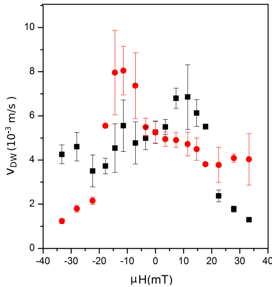
Figure 5.38: Plot of the speed DW versus B_{in} . The red spots are for the right DW whereas the black spots are for the left DW.
