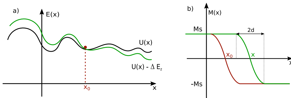
Figure 2.16: a) Energy distribution U(x) and its change ( U(x) - \Delta E_z ) when a magnetic field is applied. b) Profile of the magnetisation before and after the application of a magnetic field
