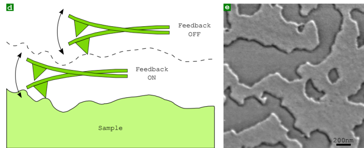
Figure 3.35: (d) Scheme for the two-pass MFM procedure. (e) 2 \times 2 \mu\text{m}^2 MFM domain pattern of a 4 nm-thick epitaxial FePt(001) film with perpendicular magnetisation (sample and image courtesy: A. Marty and O. Fruchart).
