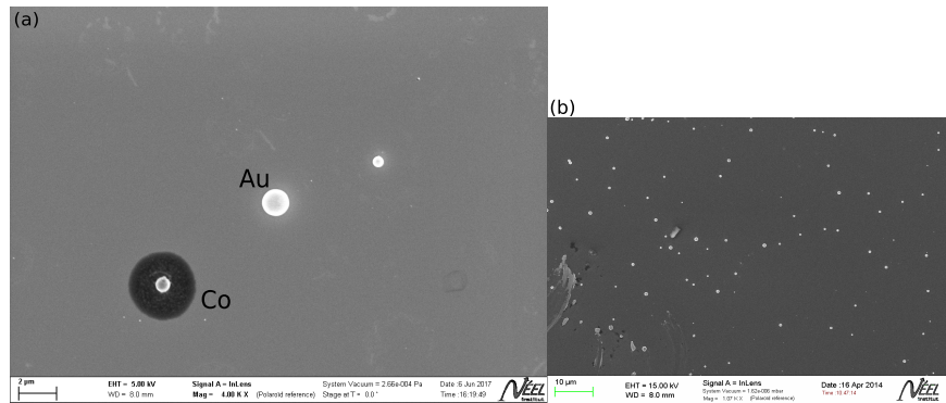
Figure 5.18: EDSX image of a continuous Au film with the presence of Au droplets.
