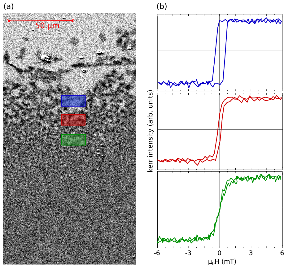
Figure 5.56: (a) Differential polar Kerr image taken after saturation of the system by the application of a strong out-of-plane field (b) Polar Kerr hysteresis loops as a function of an out-of-plane field, the plot colors indicate the areas in (a) where the Kerr signal is collected.
