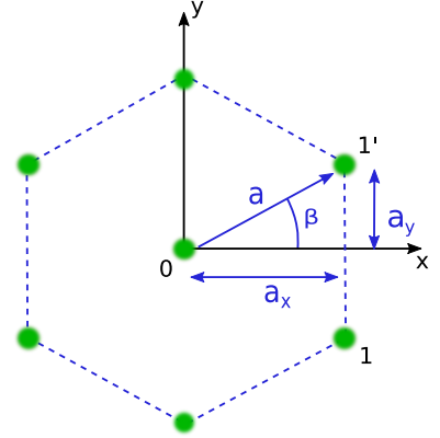
Figure 2.3: Sketch of a strained hcp (0001) surface
