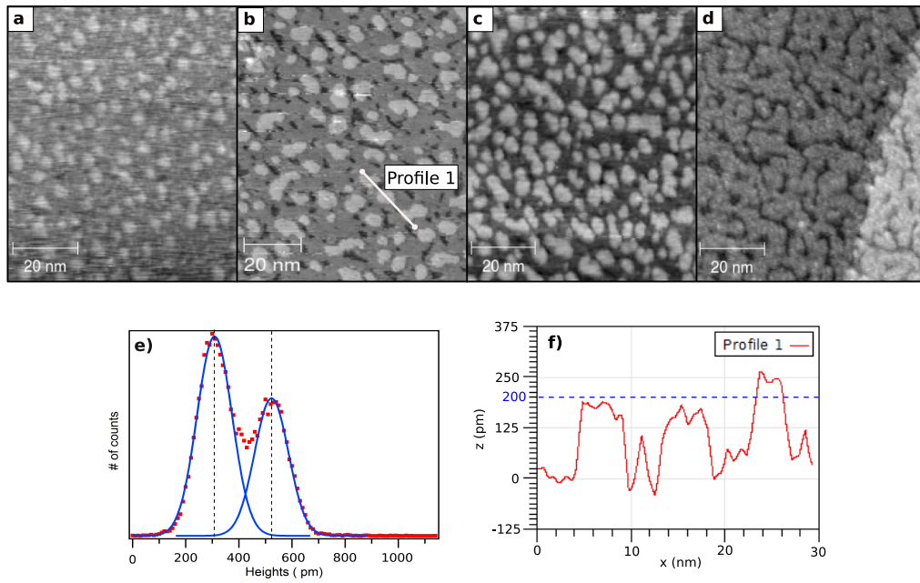
Figure 5.23: STM pictures of Co islands during a quasi-layer-by-layer deposition in different positions along a Co wedge. a) 1.15 ML b) 1.45 ML c) 1.62 ML d) 1.93 ML are the thickness of the Co layer that can be calculated studying the coverage ratio of Co islands. e) Plot of the heights of the islands as a function of the STM picture (b). f) plot of the island heights along profile 1 in the STM picture (b)
