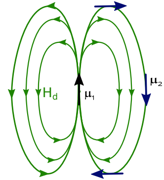
Figure 2.12: Sketch of the stray field ( \mathbf{H}_d ) produced by a magnetic moment \boldsymbol{\mu}_1 and three positions of the moment \boldsymbol{\mu}_2 that minimizes the dipolar energy.
