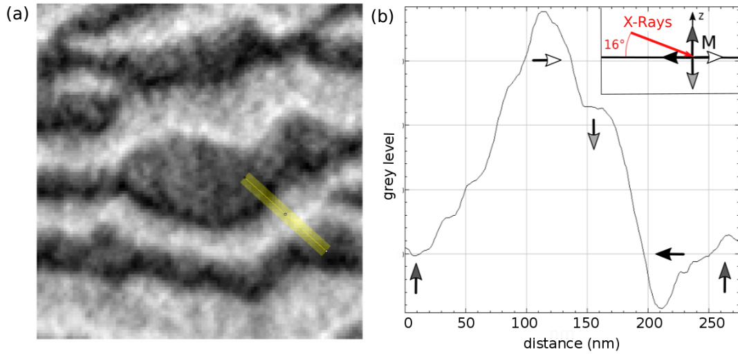
Figure 5.62: (a) XMCD images with the X-Rays parallel to the hard axis (zoom of the image in Fig. 5.61(d)). (b) Profile of the contrast along the yellow line in (a).
