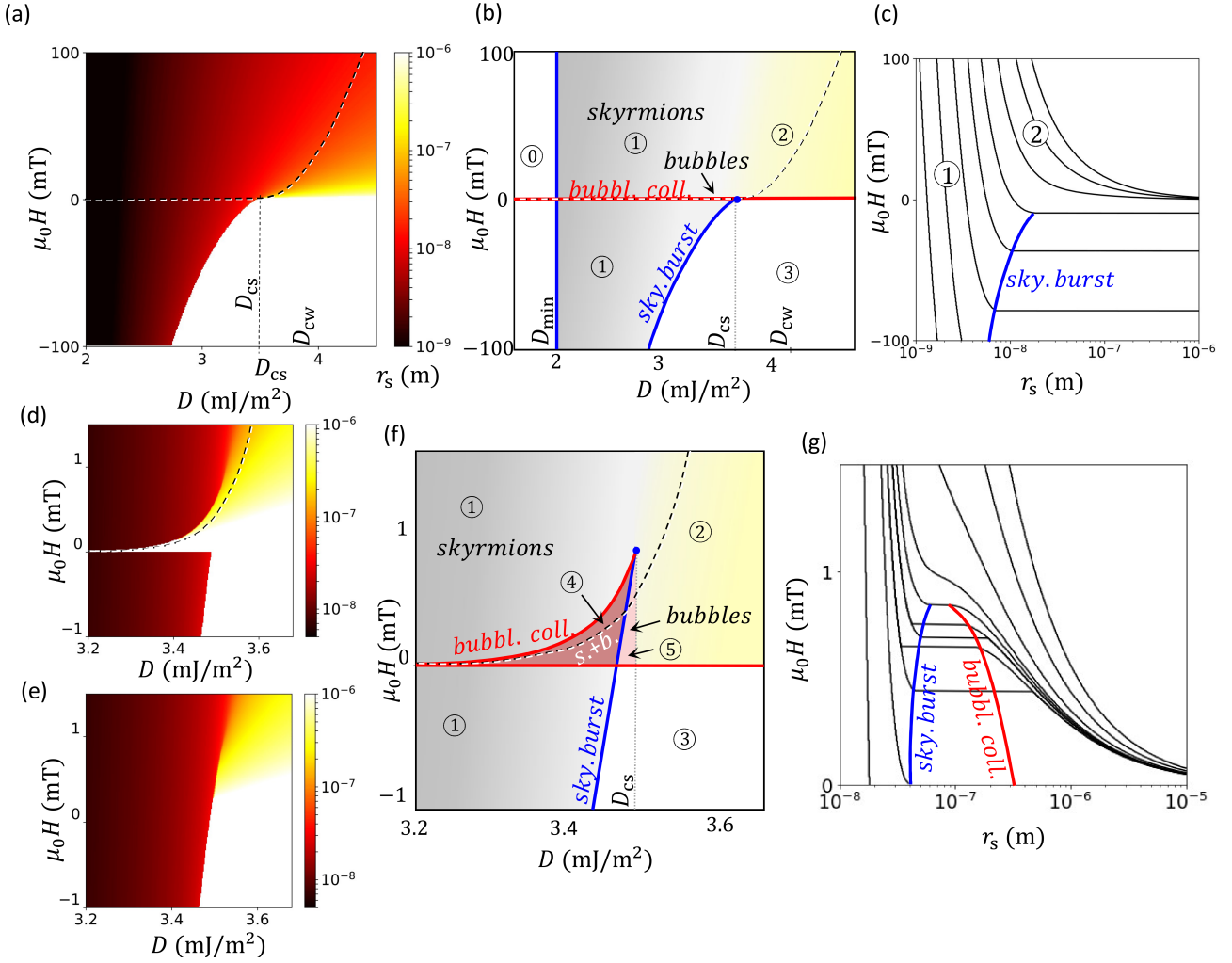
Figure 4.25: (a), (d) and (e) Soliton equilibrium radius as a function of applied magnetic field and parameter D , calculated with the same parameters as in Fig. 4.24. (d) and (e) shows respectively the radius corresponding to the larger/smaller solution, when two solutions coexist. (b) and (f) Schematic representations of characteristic lines appearing in Fig. 4.25a and Fig. 4.25d and defined in Sec. 4.4.2: dashed black line: limit for isolated solitons, green line: bubble collapse line, blue line: skyrmion busting line. (c) and (g) Soliton equilibrium radius as a function of magnetic field for fixed D values. The D values are ranging close to the critical point from D = 3.476 mJ/m 2 to D = 3.524 mJ/m 2 for (c) and from D = 2.4 mJ/m 2 to D = 4.2 mJ/m 2 for (f).
