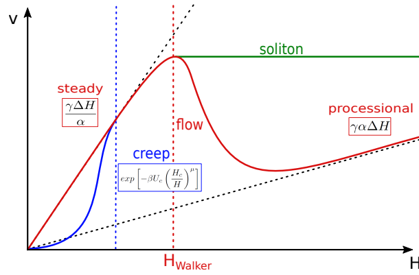
Figure 5.33: Review of the DW regimes described in this section
