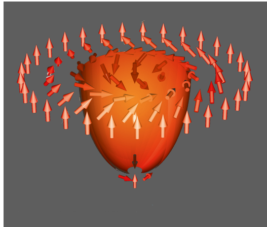
Figure 4.7: Artistic sketch of the magnetisation configuration of a Bloch skyrmion (upper object) and of a Bloch point (lower object). ( from the 2017 IFF Spring School poster .Copyright: Forschungszentrum Julich )
