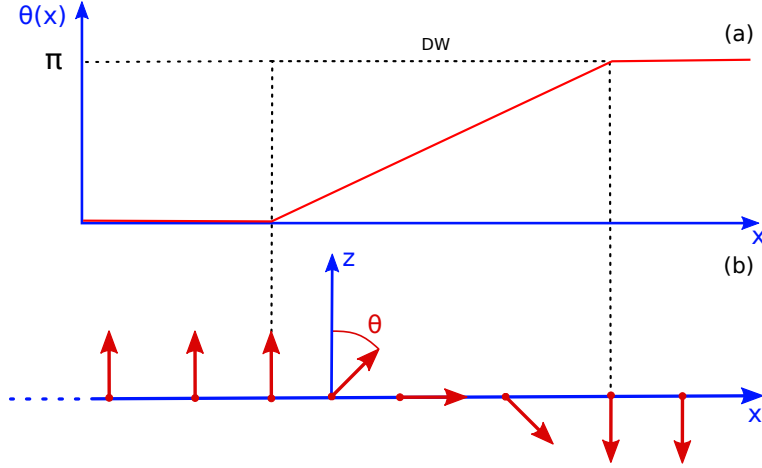
Figure 4.9: (a) Plot of a linear DW profile \theta(x) . (b) Vectorial plot of the magnetisation profile \mathbf{m}(x) in a linear DW
