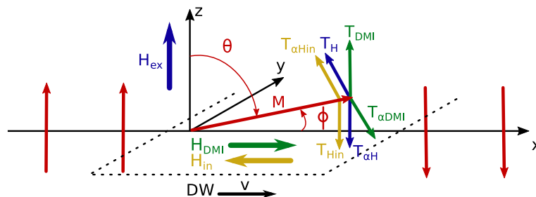
Figure 5.29: Sketch of a Néel DW and of the torques that act on the DW macrospin when two external magnetic fields are applied along the \hat{z} and the -\hat{x} directions.
