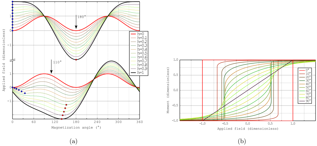
Figure 2.15: [38] (a) Energy profiles for increasing values of applied field, of a macrospin with uniaxial anisotropy. Profiles are drawn for the magnetic field applied along the easy axis ( \theta_B = \pi , top) and along an intermediate angle ( \theta_B = 110^\circ , bottom). For the latter, the series of profiles are slightly shifted vertically for clarity. The initial (resp. final) minima are marked with blue (resp. red) dots. (b) Hysteresis loops for various angles of applied field \theta_B . Equal values for angles symmetric with respect to 45^\circ are clearly evidenced.
