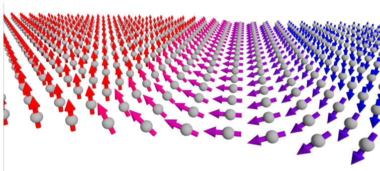
Figure 4.8: Artistic sketch of a domain wall
