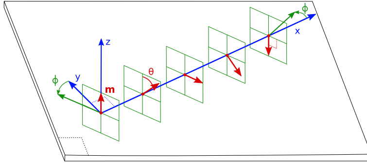
Figure 4.11: Sketch of a generic spin modulation in a thin film system.
