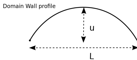
Figure 5.32: Sketch of the geometrical parameters used to describe the deformation of a DW ( u ) between two pinning points with a distance ( L )
