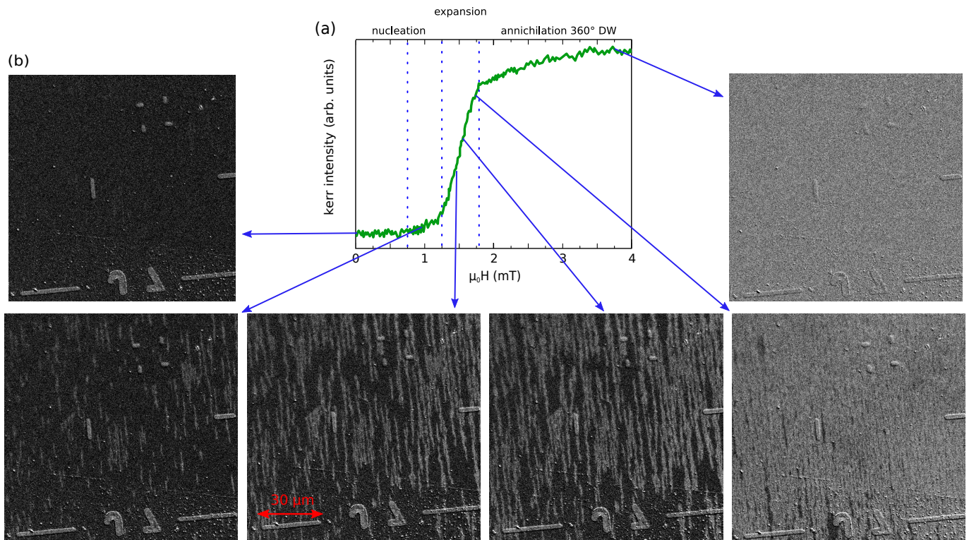
Figure 5.57: (a) Polar Kerr intensity as a function of an out-of-plane magnetic field. (b) Differential Polar Kerr images. The pictures are obtained as the difference between the image of a saturated state and the magnetic configuration after the application of the field shown with the arrows on plot (a)
