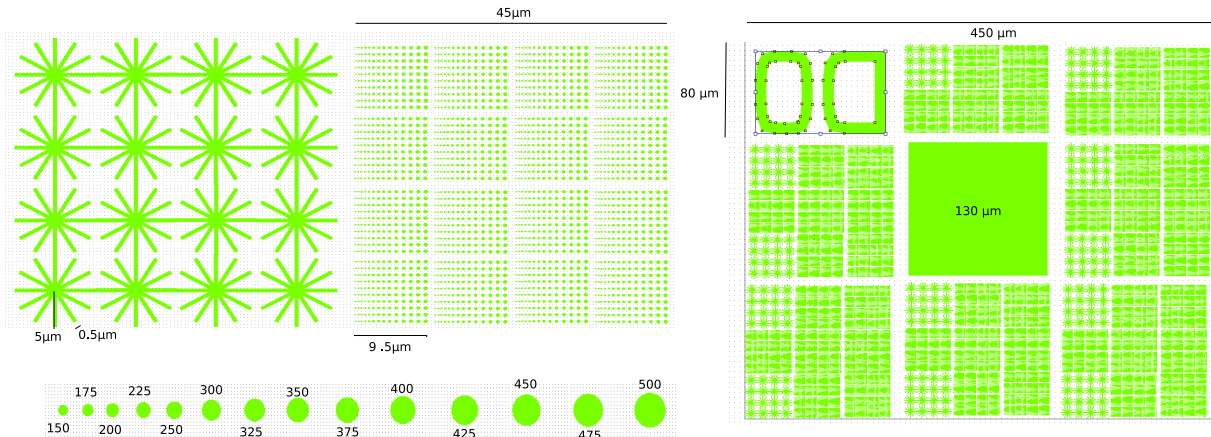
Figure 5.49: Design of the nanostructures patterned on the W\Co\Au continuous film
