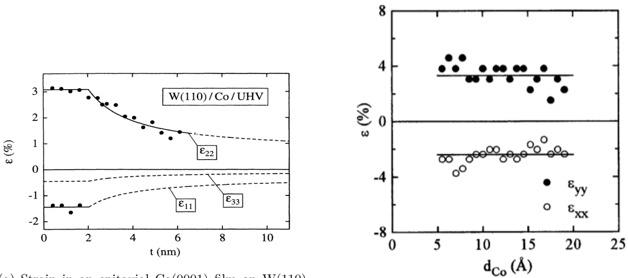
(a) Strain in an epitaxial Co(0001) film on W(110) versus thickness t . Experimental data taken by LEED spectroscopy in [120] are fitted by the full lines using the strain model explained in the chapter.
