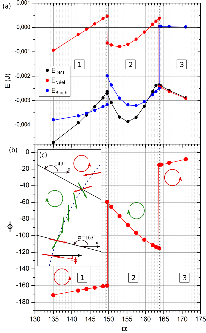
Figure 4.20: Solutions of eq. 4.89 with K_{\text{in}} = 0.3 \cdot 10^6 \text{J/m}^3 , K_{\text{out}} - K_{\text{d}} = 0.5 \cdot 10^6 \text{J/m}^3 , D^y = 1 \text{ mJ/m}^2 and D^x = -2 \text{ mJ/m}^2 (a) Plot of the DMI energy (black) and the two components promoting a Bloch (blue) and a Néel (red) DW. (b) The angle \phi as a function of \alpha in the area where the slope inversion occurs. (c) Polar plot of the function in (b). The magnetisation vectors are colored green if \phi rotates clockwise with alpha and red if it rotates anti-clockwise.
