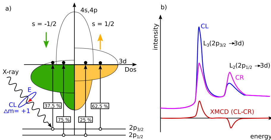
Figure 3.32: a) Sketch of the interaction between a 3d transition metal and circularly polarized light. b) Typical XMCD spectra for a transition metal
