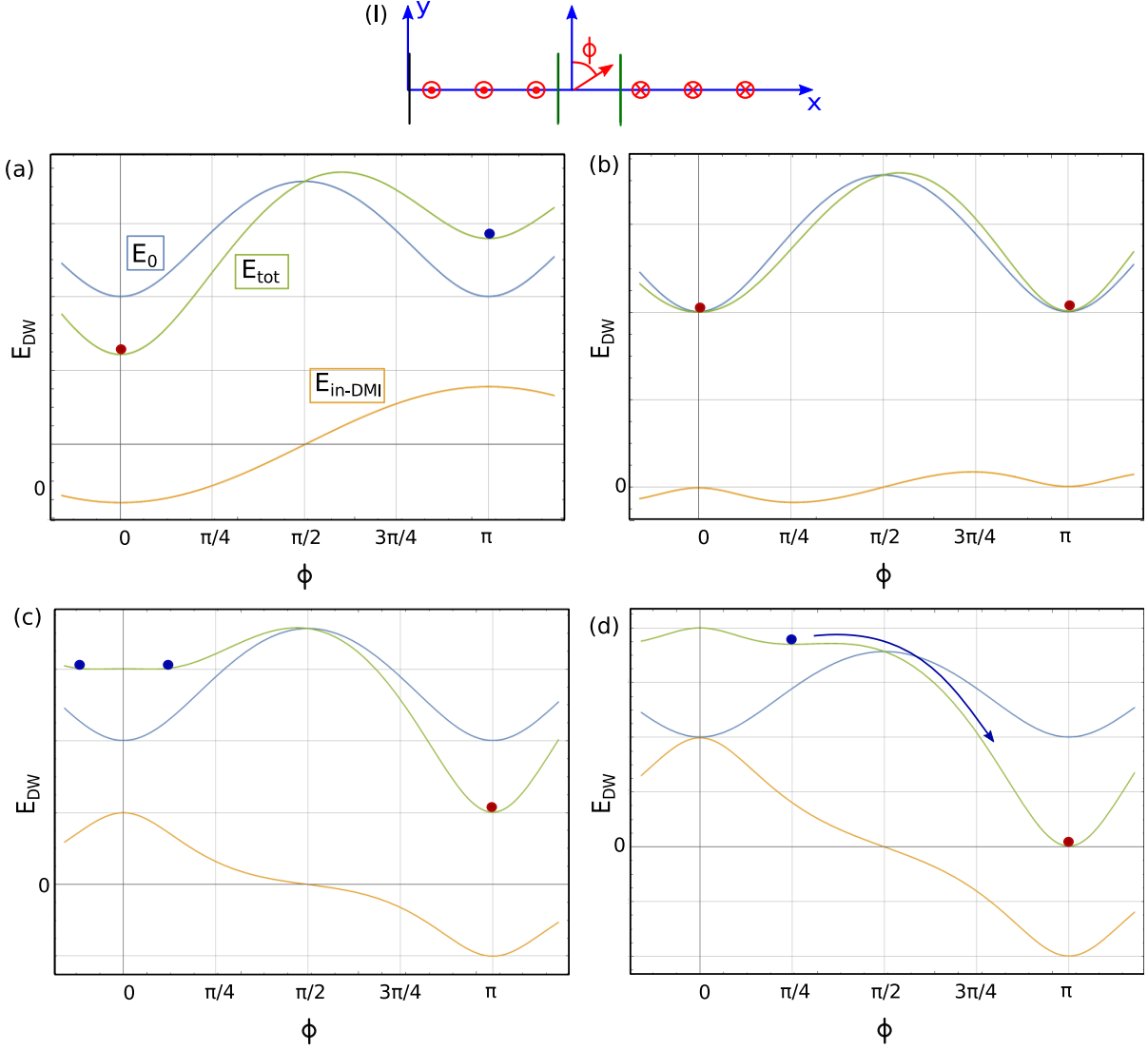
Figure 4.21: (I) frame used to describe the DW energy . (a-b-c-d) Plot of DW energies in eq. 4.91 as a function of the polarisation angle \phi for three different values of an in-plane magnetic field applied along the direction \phi = \pi . (orange) Sum of the DMI and Zeeman DW energy terms, (blue) DW energy without the DMI and Zeeman DW energy terms and (green) total DW energy.
