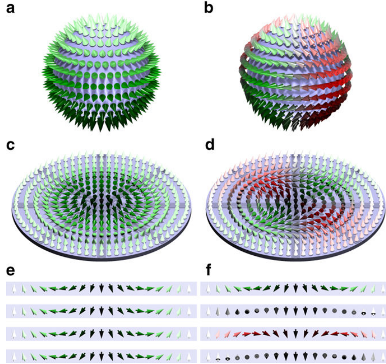
Figure 4.3: Comparison of skyrmion and anti-skyrmion. (a), (b) Néel-like skyrmion and anti-skyrmion schematically shown in (c) and (d) mapped onto a sphere. The color code represents the out-of-plane component of the spins via the brightness, with bright (dark) spins pointing up (down), and their rotational sense in radial direction going from inside out changing from red (clockwise) via gray (vanishing rotational sense) to green (counter-clockwise). (e), (f) Cross sections of the spin textures along the four highlighted directions shown in (c) and (d). Taken from Ref. [18]
