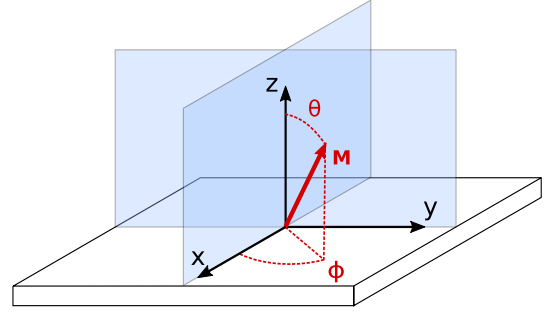
Figure 2.11: Sketch of the symmetry planes in a C_{2v} system (blue planes) and the frame used to describe the magnetisation in polar coordinates.
