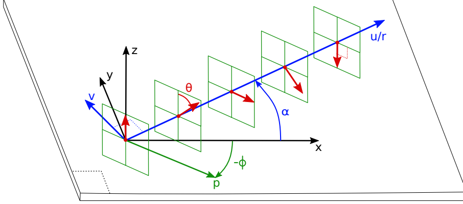
Figure 4.15: Frame used to study the DW profile and polarisation in a system with C_{2v} symmetry
