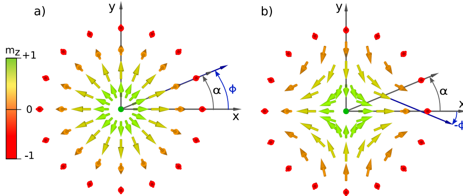
Figure 4.22: Sketch of the skyrmion and anti-skyrmion configurations. The illustration of \alpha , the space angle in the plane, and \phi , the in-plane magnetisation angle, show the difference between a skyrmion ( \phi(\alpha) = \alpha ) and an anti-skyrmion ( \phi(\alpha) = -\alpha ).
