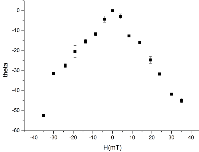
Figure 5.40: Plot of the angle of maximum DW speed \theta as a function of B_{in} applied along 37^\circ . The zero of \theta is set along the easy axis
