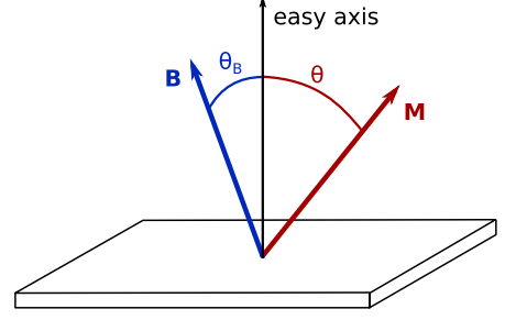
Figure 2.14: Sketch of the magnetic field \mathbf{B} and the macrospin magnetisation \mathbf{M} in a system with a volume V . \theta and \theta_B are respectively the angle between \mathbf{M} and the easy axis and between \mathbf{B} and the easy axis.
