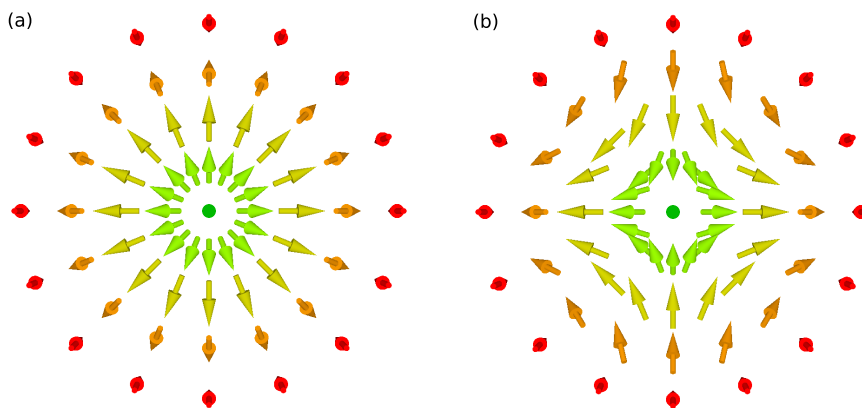
Figure 1.1: Artistic images of a skyrmion (a) and an anti-skyrmion (b) magnetic configuration
