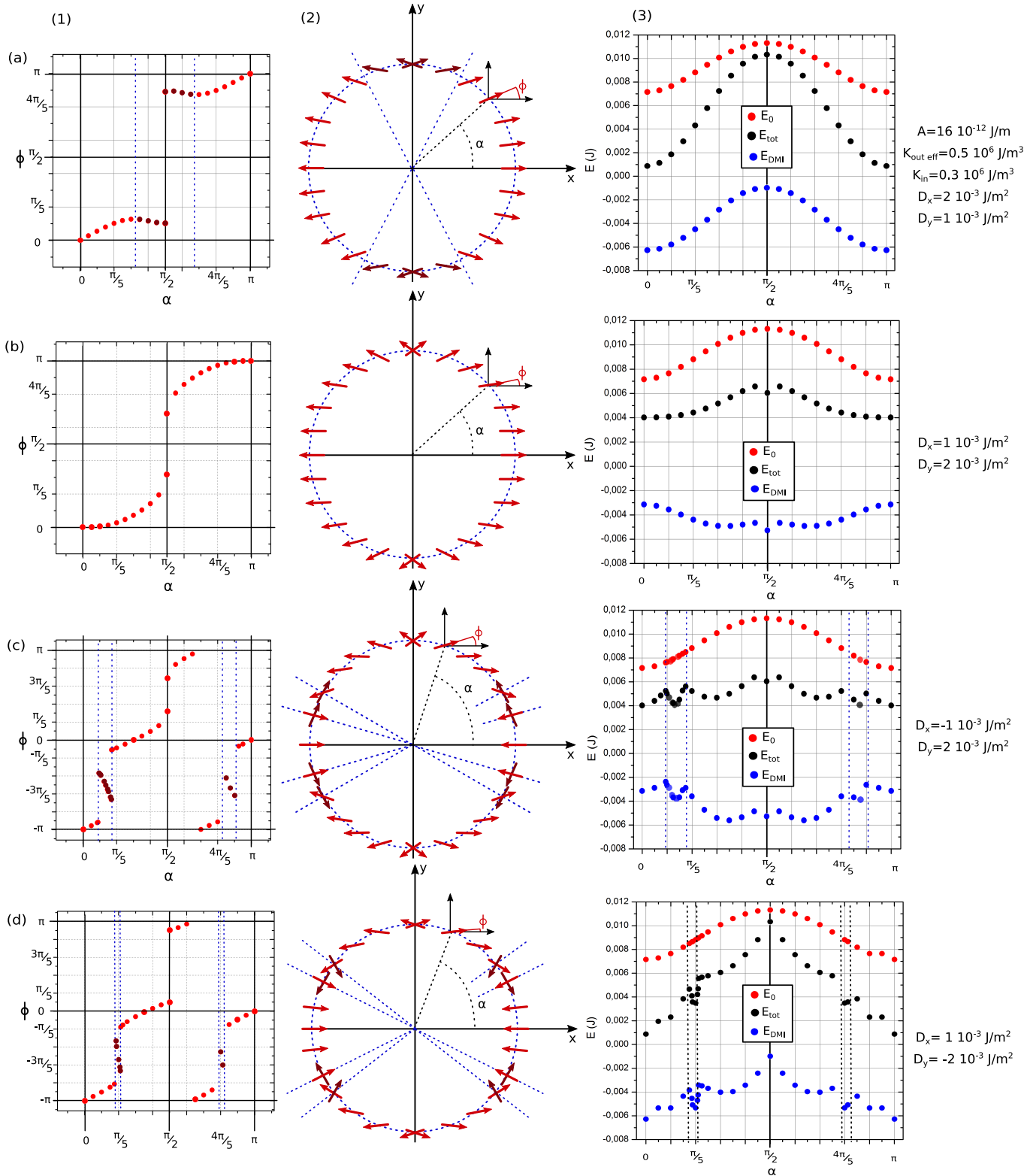
Figure 4.19: (1) Polarisation angle \phi as a function of the angle \alpha ; (2) Polar plot of graph (1) and (3) DW energy (black) and the components E_0 (red) and E_{\text{DMI}} (blue) as a function of the in-plane angle \alpha . The points are the numerical solutions of eq. 4.89. Arrows of different colors are used for positive (light red) and negative (dark red) slopes of the \phi(\alpha) function. The solutions are shown for four different physical combinations of D^y and D^x : K_{\text{in}} = 0.3 \cdot 10^6 \text{ J/m}^3 , K_{\text{out}} - K_{\text{d}} = 0.5 \cdot 10^6 \text{ J/m}^3 , (a) D^y = 1 \text{ mJ/m}^2 and D^x = 2 \text{ mJ/m}^2 ; (b) D^y = 2 \text{ mJ/m}^2 and D^x = 1 \text{ mJ/m}^2 ; (c) D^y = 2 \text{ mJ/m}^2 and D^x = -1 \text{ mJ/m}^2 ; (d) D^y = 1 \text{ mJ/m}^2 and D^x = -2 \text{ mJ/m}^2 .
