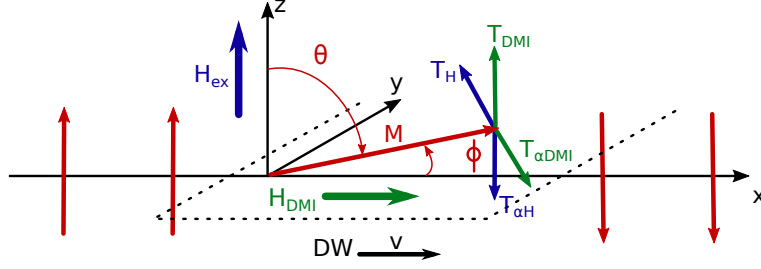
Figure 5.28: Sketch of a Néel DW and of the torques that act on the DW macrospin when an external magnetic field is applied.
