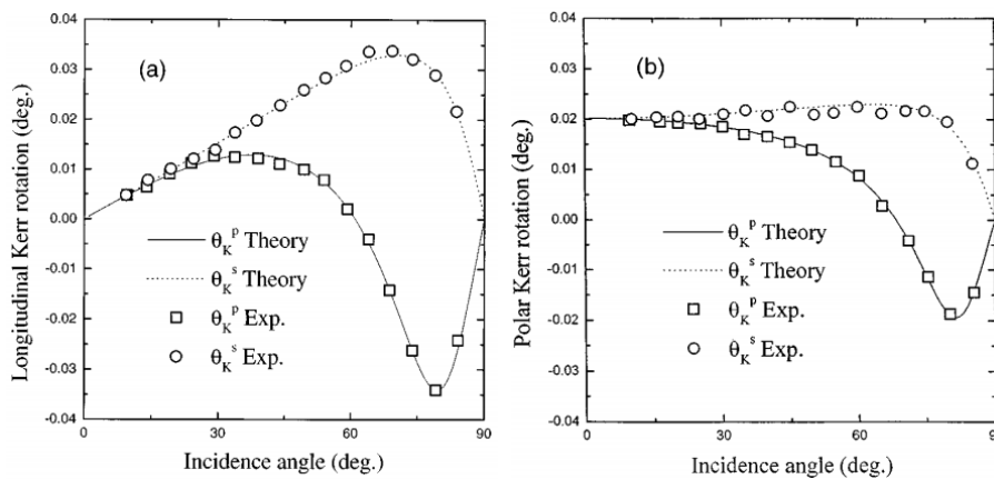
Figure 3.20: Experimental and theoretical p- and s-Kerr rotation curves of (a) a Cu/Co multilayer in the longitudinal configuration and (b) a Co/Pd multilayer in the polar configuration [55]
