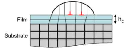
Figure 3.9: SK growth showing island formation above the critical thickness h_c . The lines represent the crystal structure and deformation. Edge dislocations at the film/island interface are highlighted in red.
