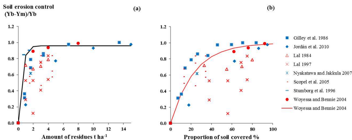
Figure 4 : Relative effect of surface crop residues on soil erosion control
