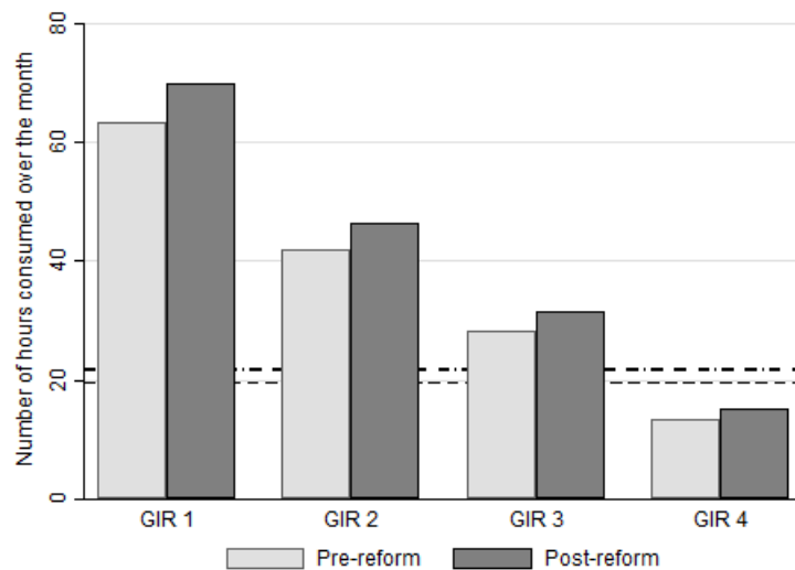
Figure 3.6 – Use of formal home care, by disability level: Pre- and post-reform comparison.
