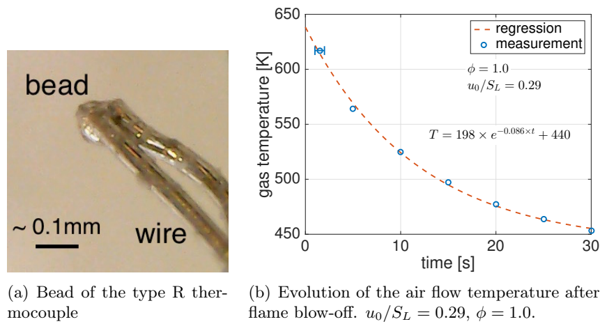
Figure 2.16: Gas temperature measurement.
