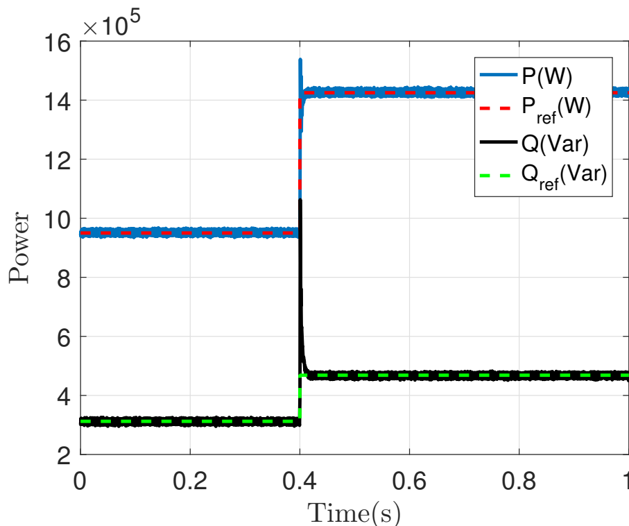
FIGURE 4.21: Power variations for the Master-Slave control case.
