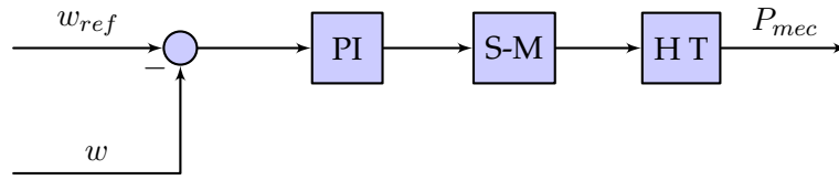
FIGURE 4.32: Hydraulic turbine block diagram.
