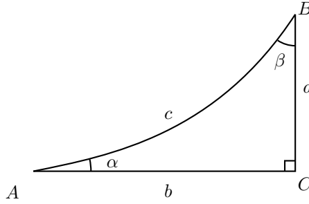
Figure 3: Right hyperbolic triangle
