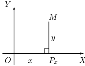
Figure 1: Equidistant coordinates (x, y) .
