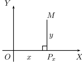
Figure 2: Equidistant coordinates (x, y)
