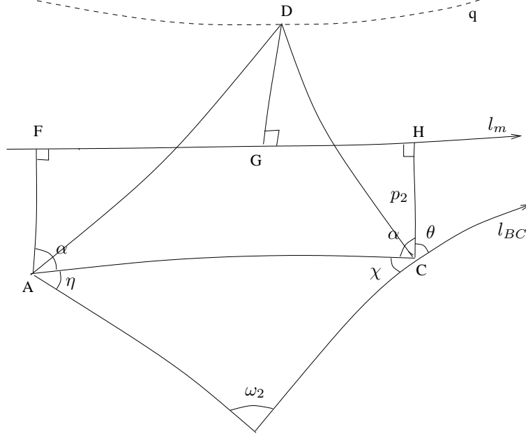
Figure 14: Non-euclidean dissection
