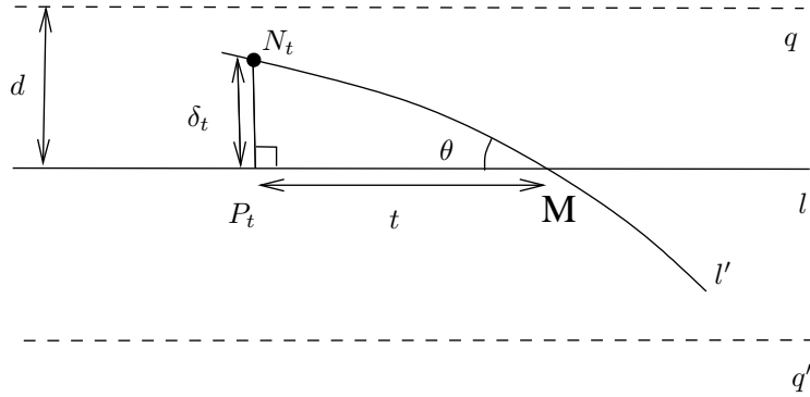
Figure 13: Proof of Lemma
