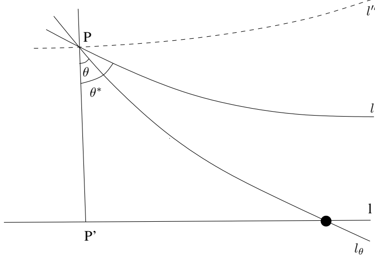
Figure 15: l' and l are parallel, l'' and l are ultra-parallel
