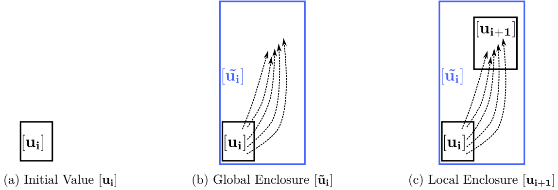
Figure 3.4: Global Enclosure [\tilde{\mathbf{u}}_i] and Local Enclosure [\mathbf{u}_{i+1}]
