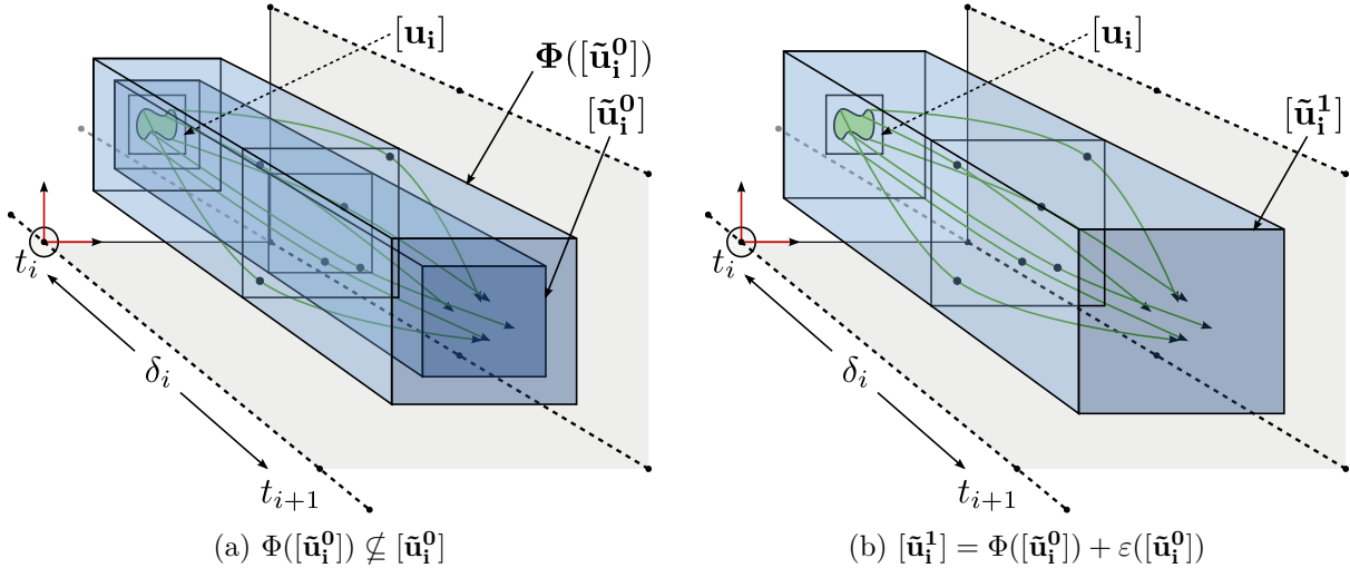
Figure 3.5: Failure of the Picard iteration, \varepsilon -inflation
