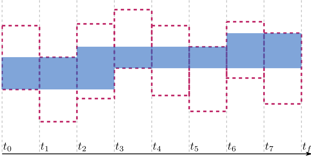
Figure 4.4: Contraction of the tube [u] with the \mathcal{C}_{increase}
