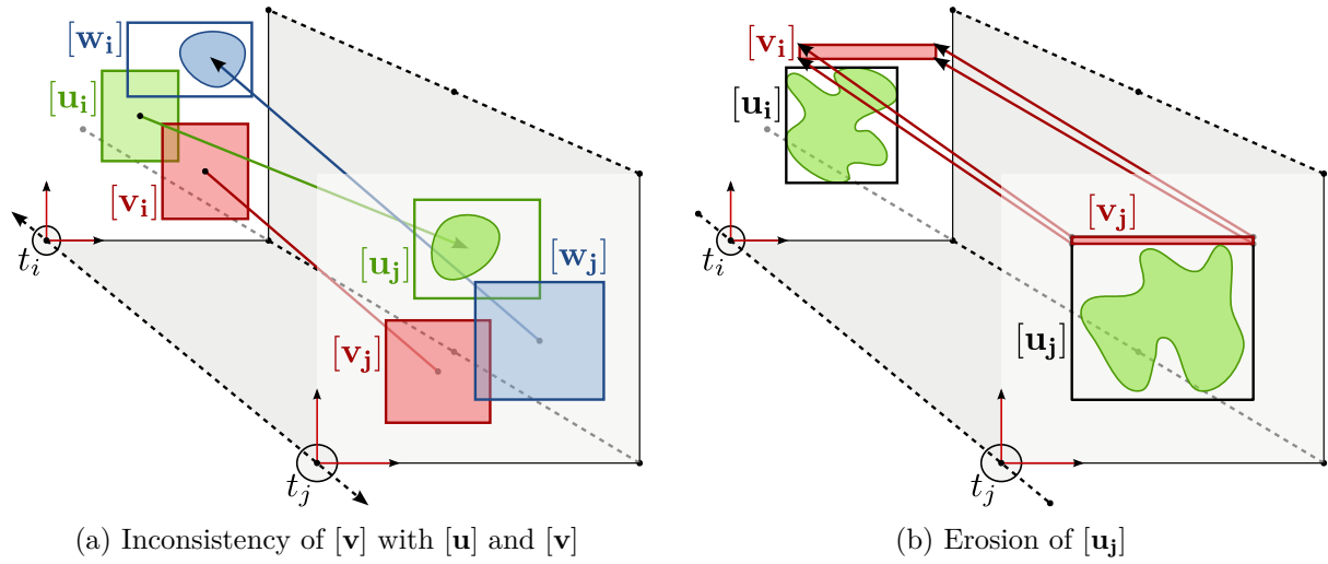
Figure 3.13: Consistency and inconsistency
