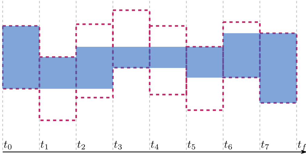
Figure 4.6: Contraction of the tube [u] with the \mathcal{C}_{\text{monotonic}}
