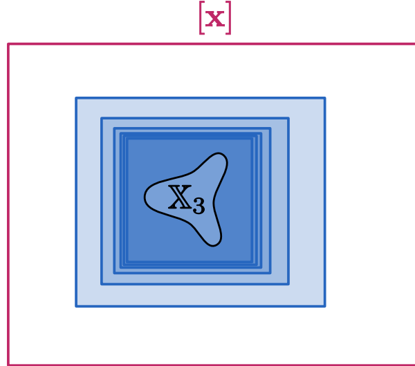
Figure 4.15: fixed point contractor
