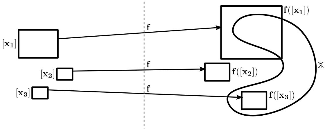
Figure 4.16: Sivia results - step 1: evaluation with \mathbf{f}
