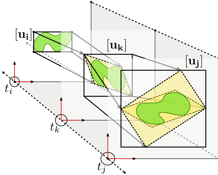
Figure 3.9: Evolution of the enclosure during the guaranteed integration
