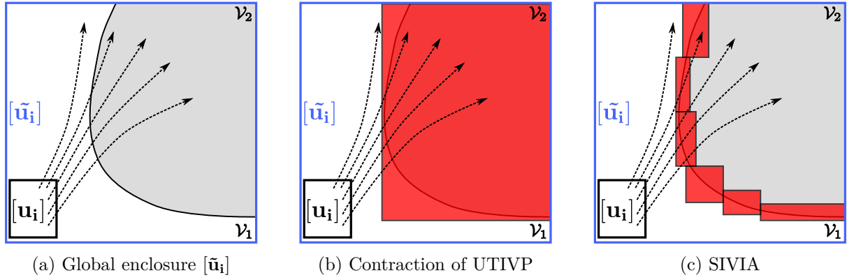
Figure 5.8: Refinement of the UTIVP with contraction and SIVIA
