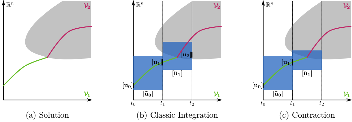
Figure 5.6: integration of a piecewise ODE - classic integration
