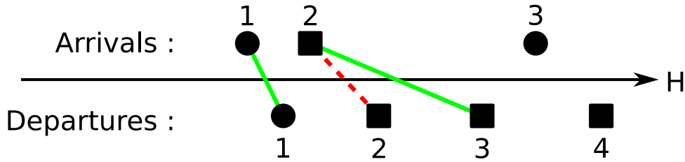
Figure A.7: Greedy Algorithm : example
