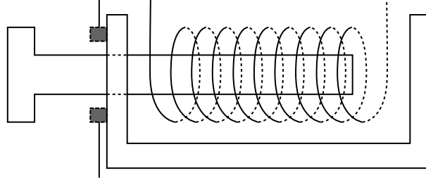
Figure 1.1: Design of the electromagnetic contactor - open position
