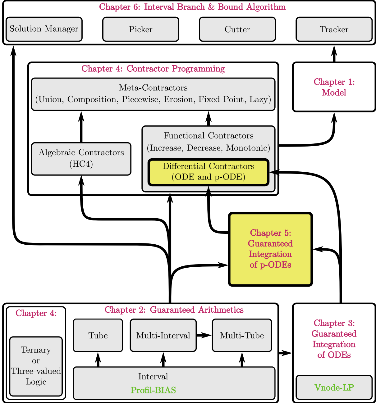
Figure 0: Architecture of the optimisation tool developed: GDODynS
