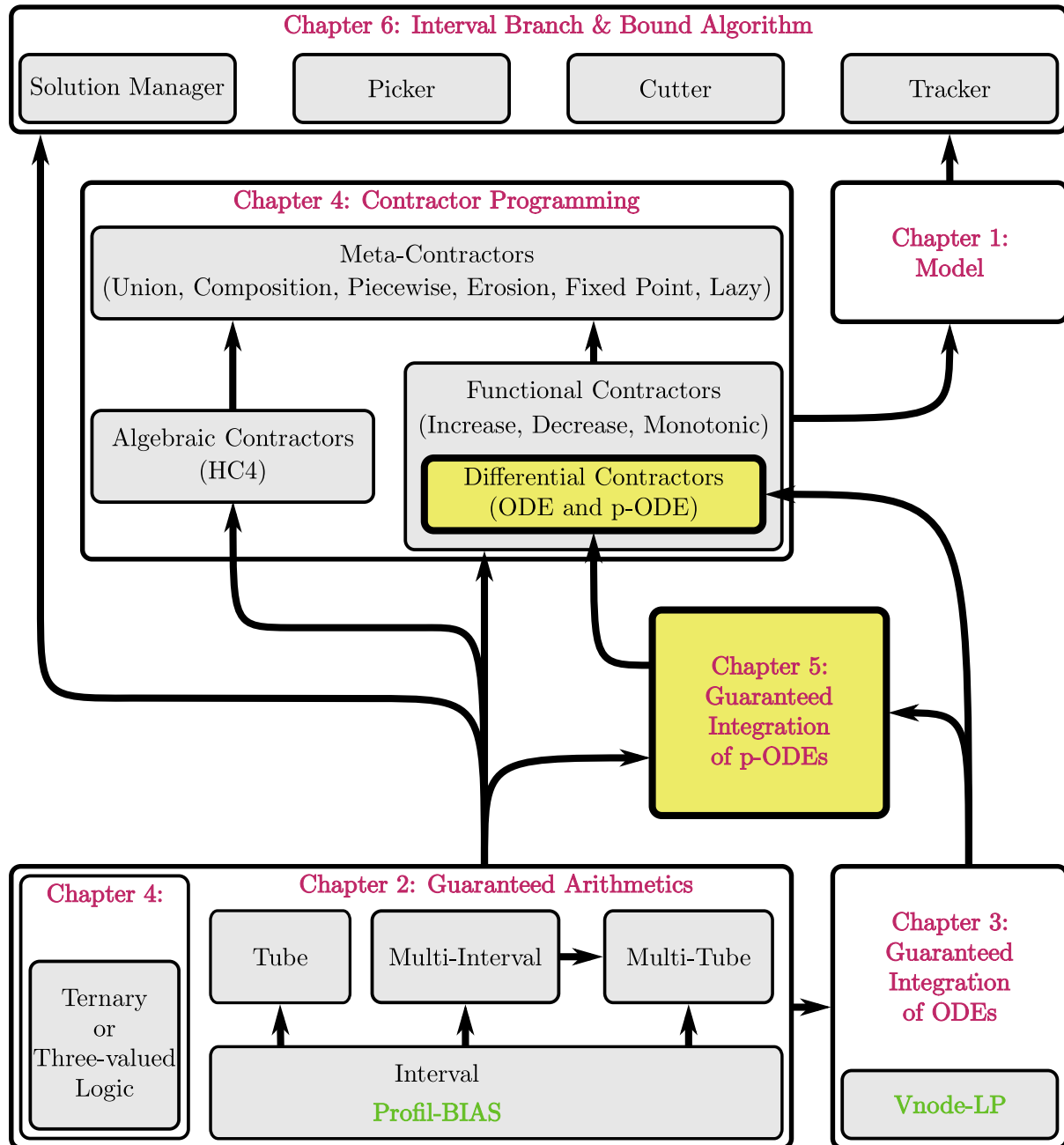
Figure 8: Architecture of the optimisation tool developed: GDODynS
