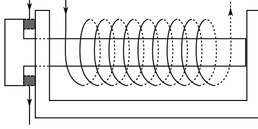
Figure 1.2: Design of the electromagnetic contactor - closed position
