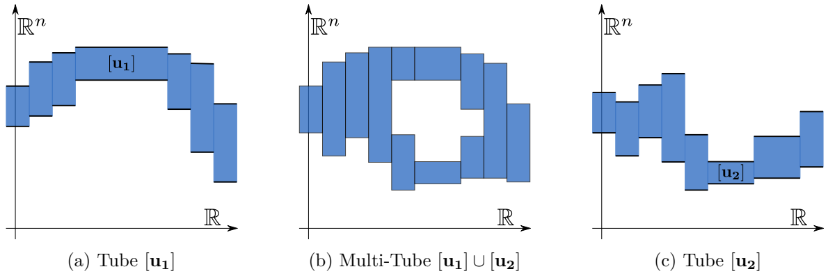
Figure 2.12: Operation on tubes [u_1] and [u_2]
