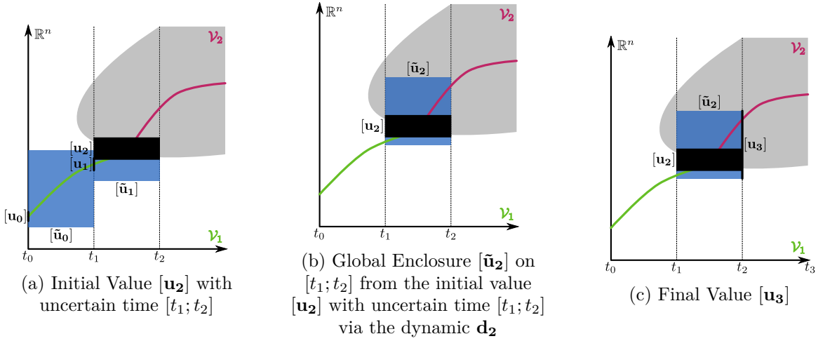
Figure 5.7: computing the new initial value
