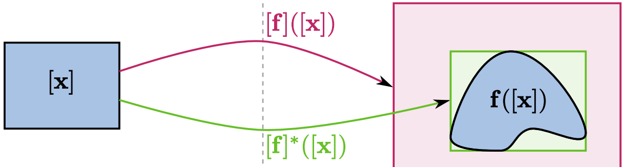
Figure 2.2: Image of the box [\mathbf{x}] by the function \mathbf{f} , by the inclusion function [\mathbf{f}] and by the minimal inclusion function [\mathbf{f}]^*
