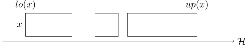
Figure A.5: Example of a multi-interval, with its lower and upper bounds.
