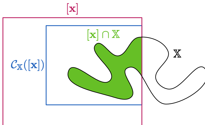
Figure 4.1: Contraction and completeness of the operator C_{\mathbb{X}}
