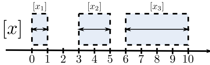
Figure 2.4: Representation of the multi-interval [x] = \{[0; 1], [3; 5], [6; 10]\} Eq. (2.40)
