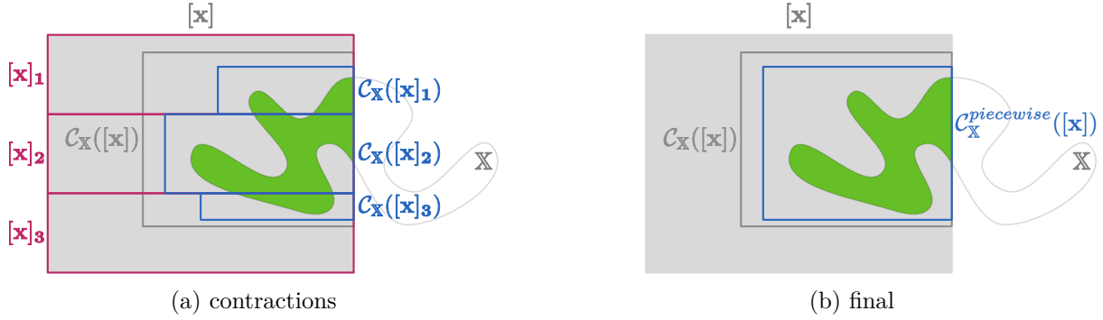
Figure 4.14: Piecewise meta-contractor over \mathcal{C}_{\mathbb{X}}
