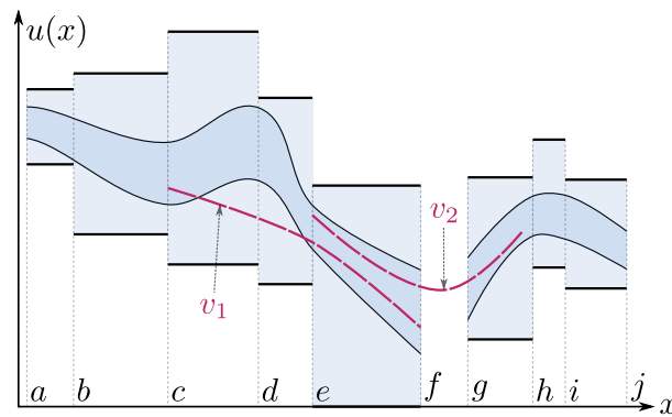
Figure 2.13: Tube [u] enclosing u : Numerical representation
