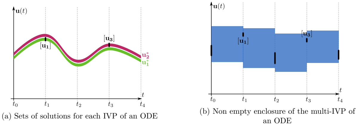
Figure 6.1: Enclosure of an unfeasible solution
