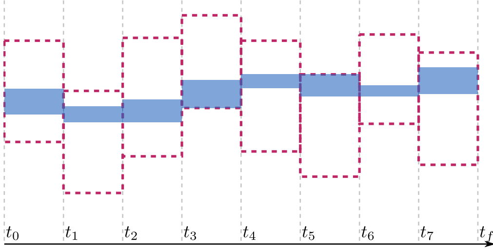
Figure 4.10: Intersection of the Forward and Backward integrations
