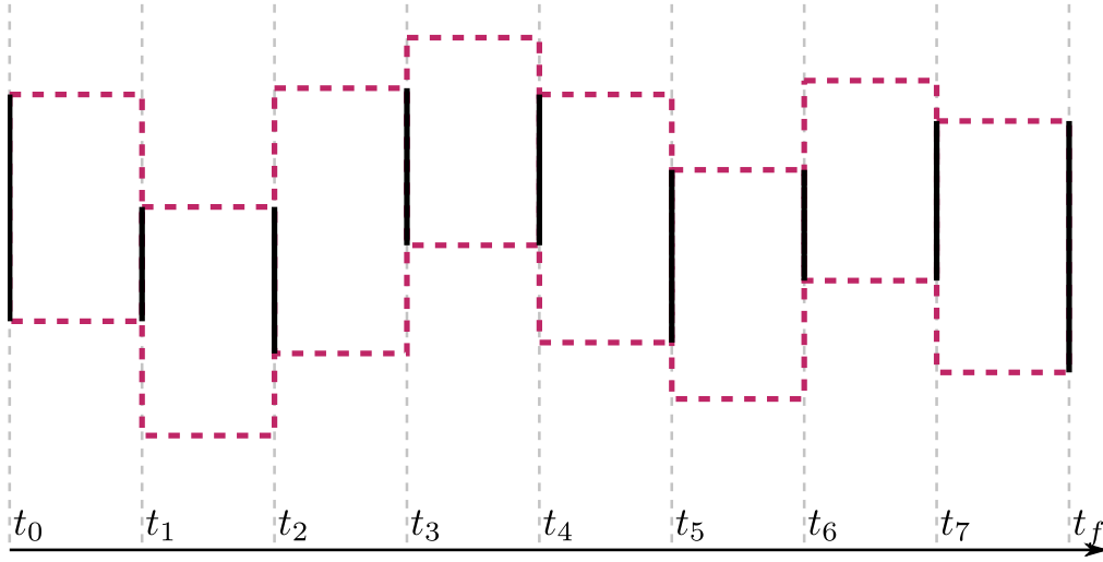
Figure 4.7: The tube [u] encloses all the functions
