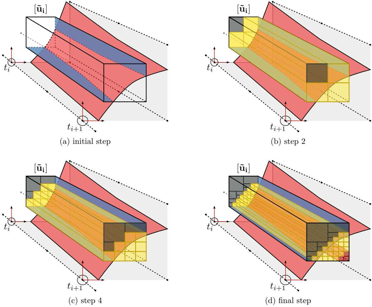
Figure 4.19: Application of the SIVIA on a tube
