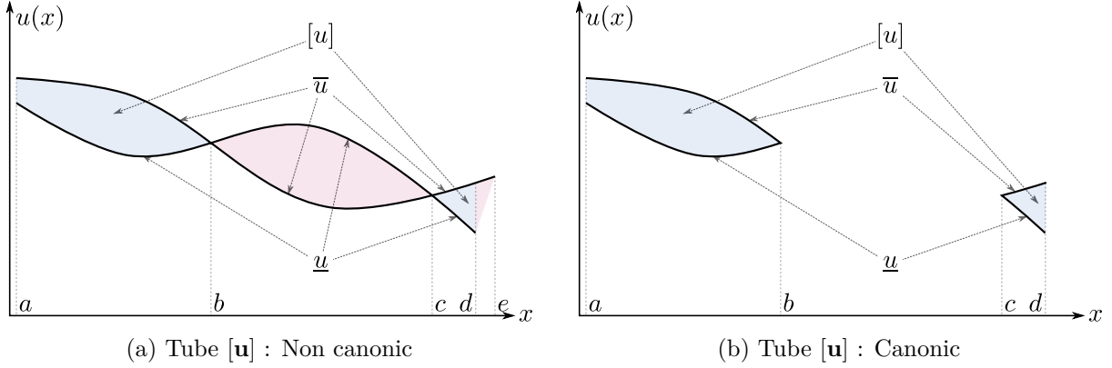
Figure 2.10: Two equivalent tubes [u]
