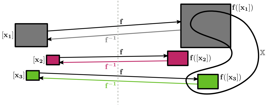
Figure 4.18: Sivia results - step 3: backward propagation of information with f^{-1}
