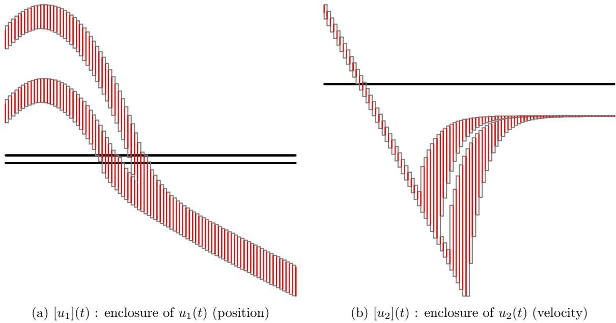
Figure 7.3: Results of the guaranteed integration with multiple initial values and minimal global enclosure approximation
