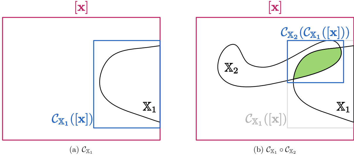
Figure 4.13: Composition of the contractors \mathcal{C}_{\mathbb{X}_1} and \mathcal{C}_{\mathbb{X}_2}
