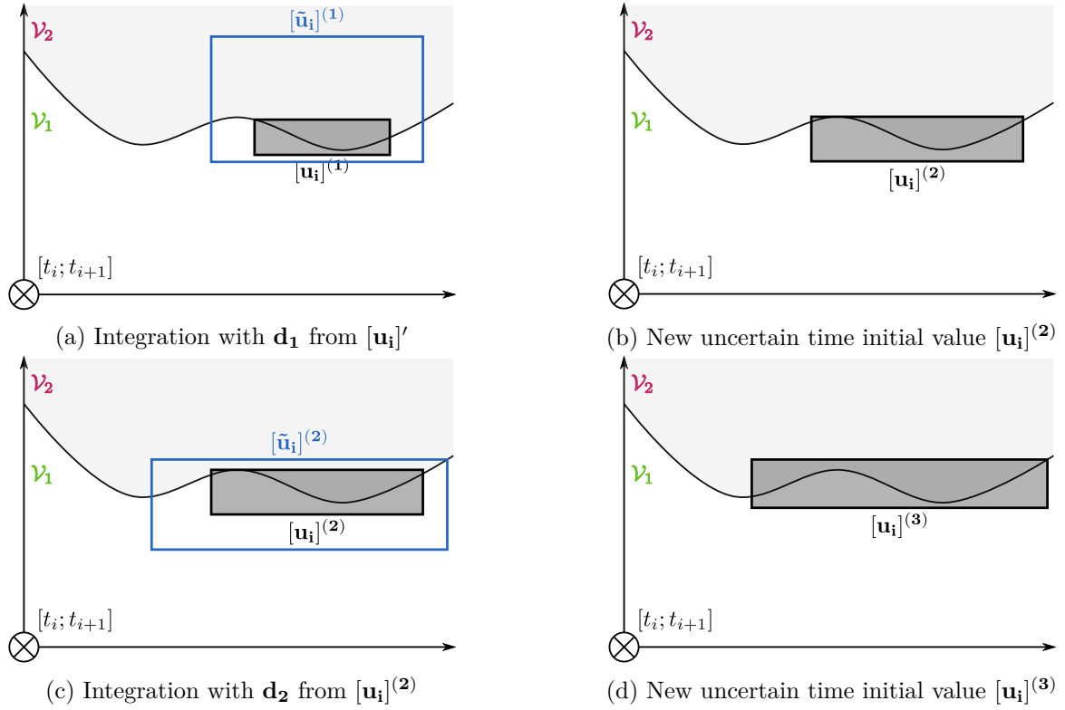
Figure 5.9: Growth of the uncertain time initial value
