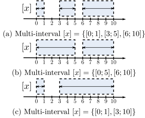
Figure 2.7: Limitation of the size of a multi-interval (Fig. 2.4)
