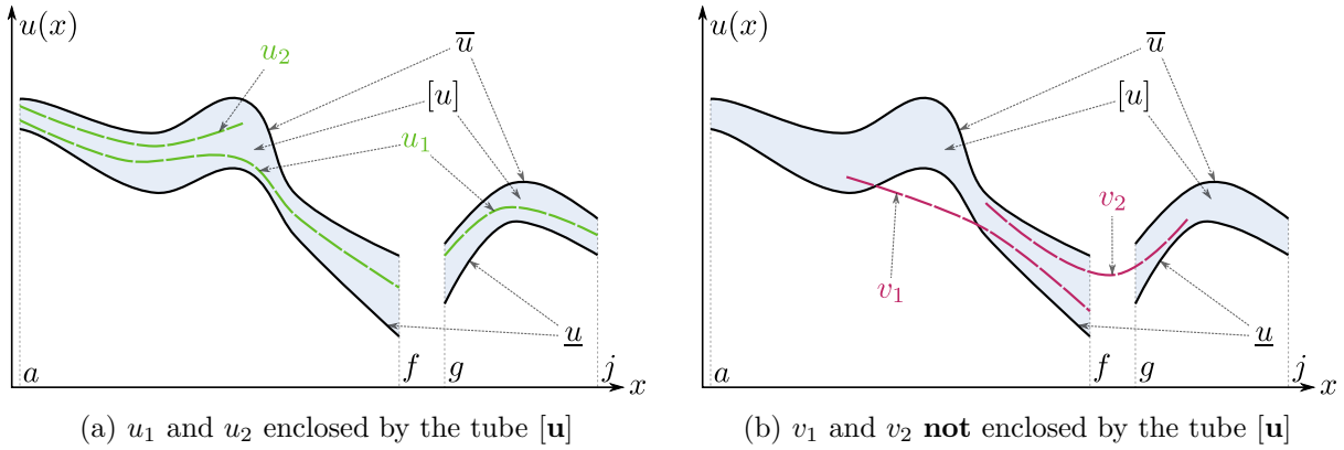
Figure 2.9: Functions inside and outside a tube
