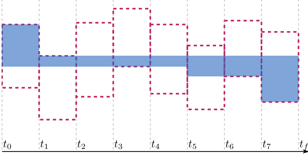
Figure 4.5: Contraction of the tube [u] with the \mathcal{C}_{decrease}
