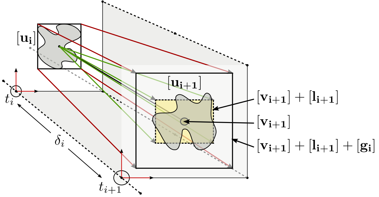
Figure 3.8: The three parts of the mean value form
