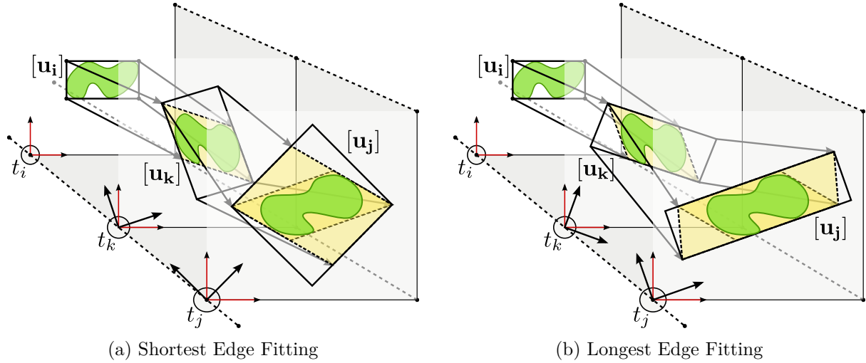
Figure 3.10: Comparison of the shortest and longest edges fitting
