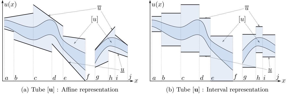
Figure 2.11: Numerical representations of a tube
