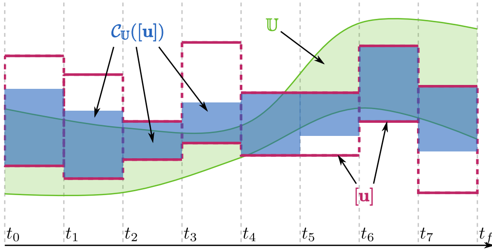
Figure 4.2: Contraction and completeness of the operator \mathcal{C}_{\mathbb{U}}
