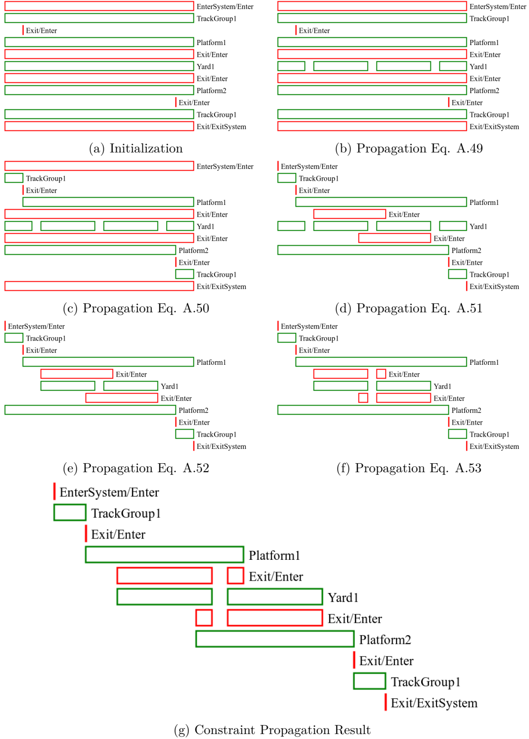
Figure A.6: Multi-Interval Filtering on the example instance, from Arr1 to Dep1 (see Table A.1) with the consumptions indicated in Table A.2.
