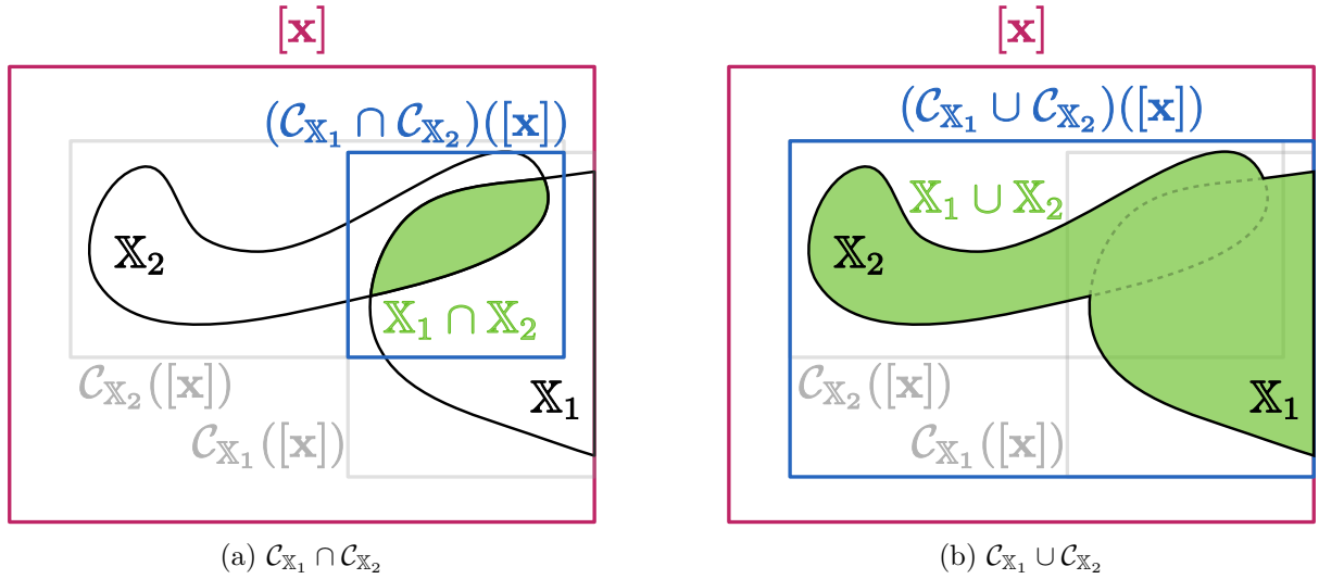
Figure 4.12: Intersection and union of the contractors \mathcal{C}_{\mathbb{X}_1} and \mathcal{C}_{\mathbb{X}_2}
