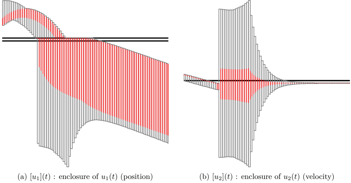
Figure 7.1: Results of the guaranteed integration
