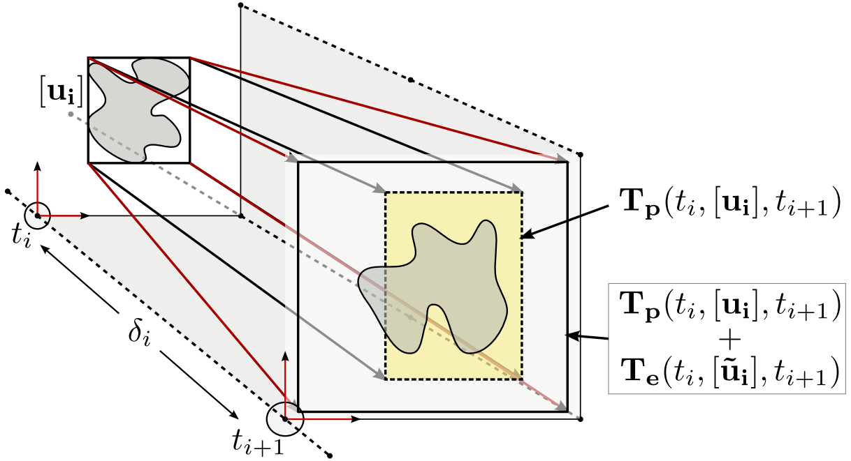
Figure 3.7: Enclosure [u_{i+1}] computed with Taylor model
