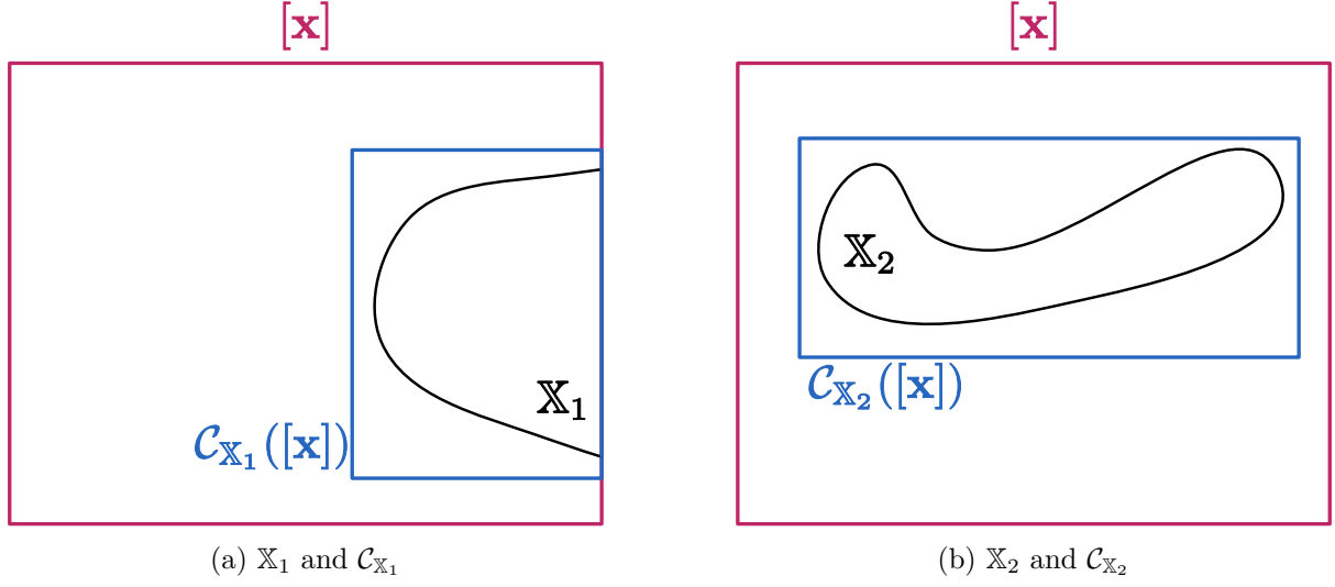
Figure 4.11: Domains \mathbb{X}_1, \mathbb{X}_2 with their associated contractors
