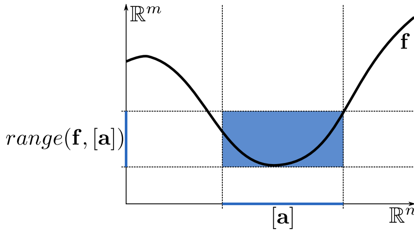
Figure 2.1: range of \mathbf{f} over [\mathbf{a}]
