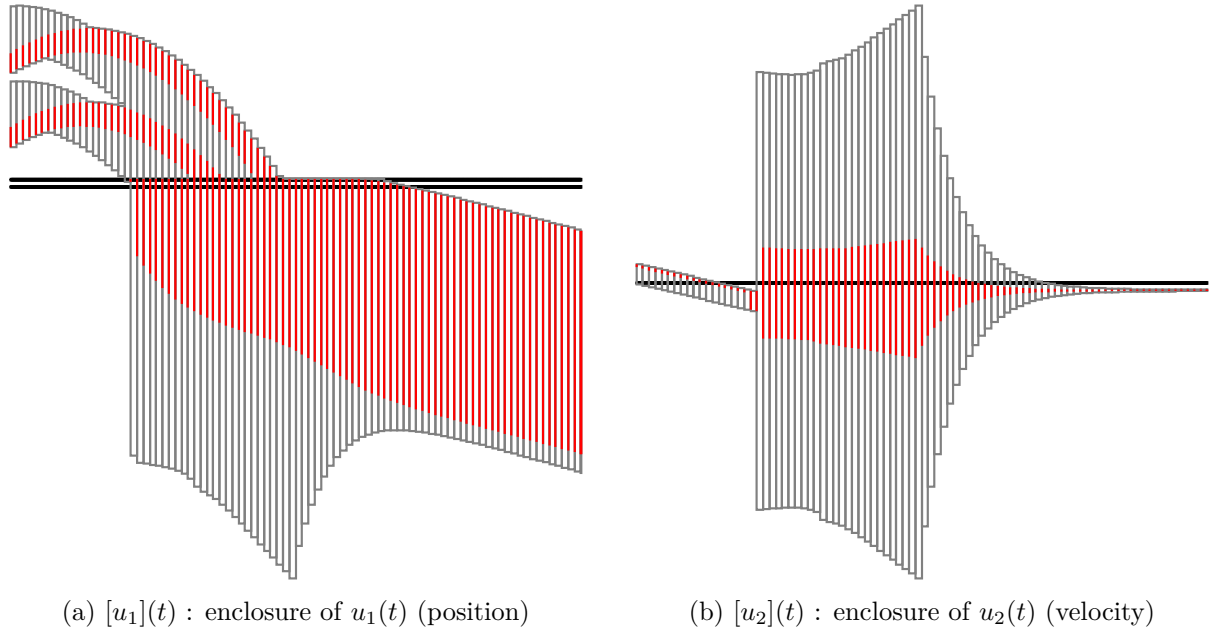
Figure 7.2: Results of the guaranteed integration with multiple initial values
