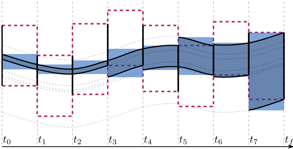
Figure 4.9: Backward integration
