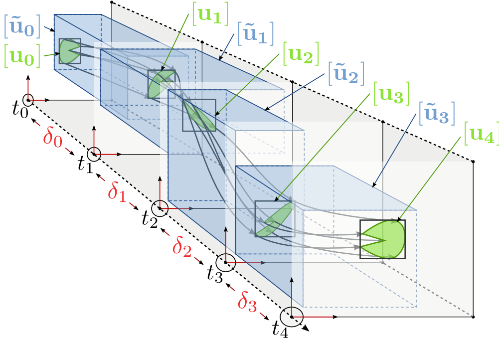
Figure 3.2: Enclosure of an ODE solution \mathbf{u}^* returned by Algorithm 1
