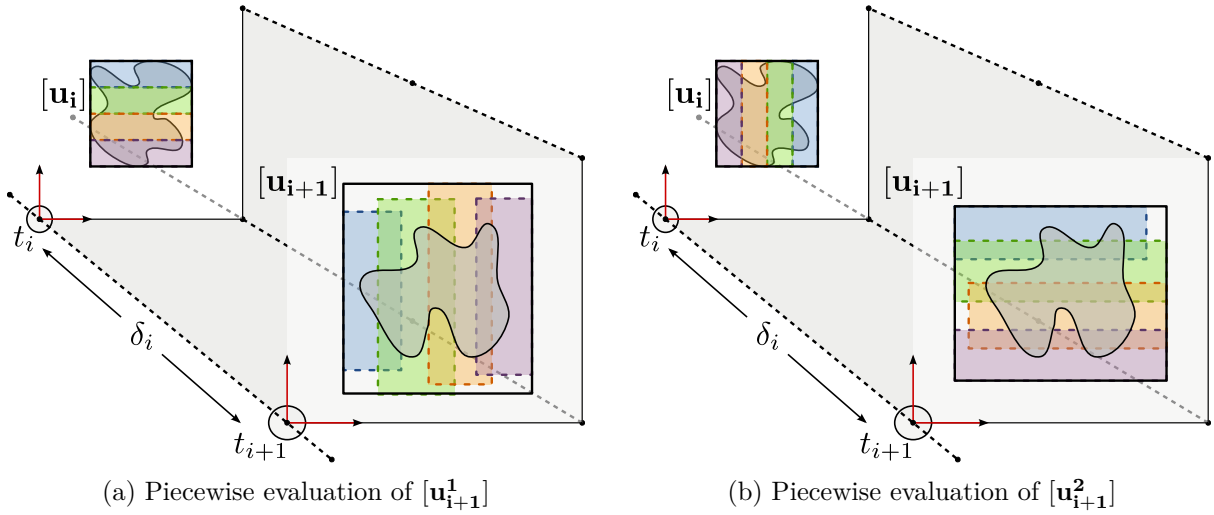
Figure 3.12: Piecewise evaluation
