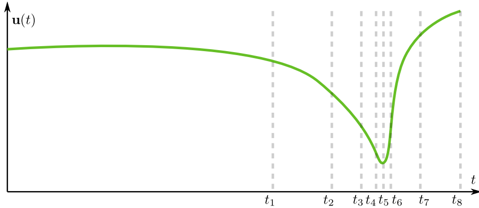
Figure 3.3: Adaptive stepsize
