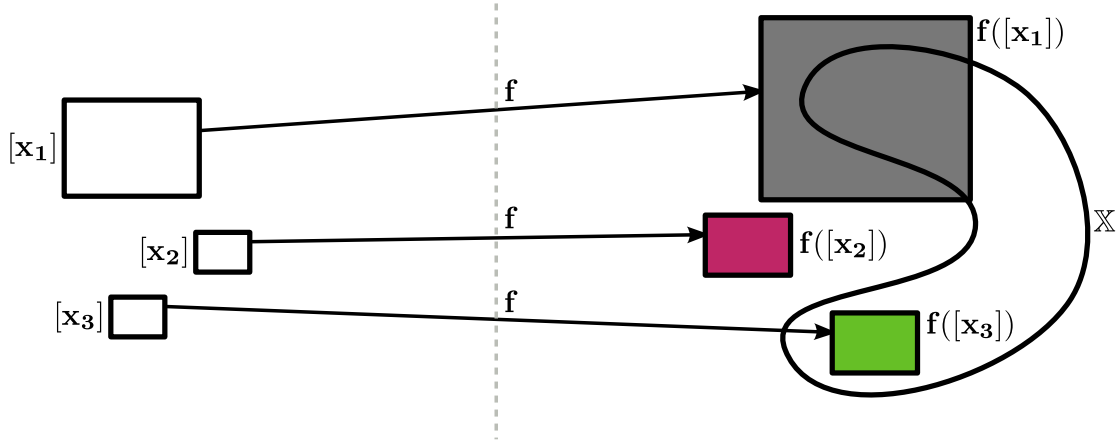
Figure 4.17: Sivia results - step 2: information on f([x])
