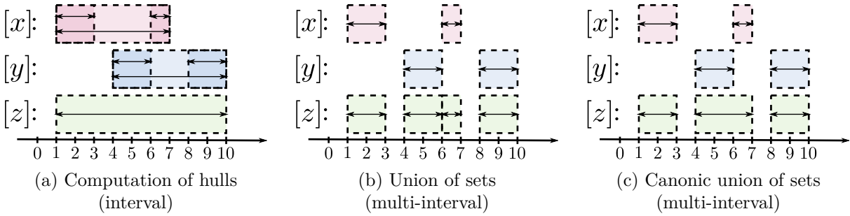
Figure 2.6: Three versions of the computation [z] \leftarrow [x] \cup [y]
