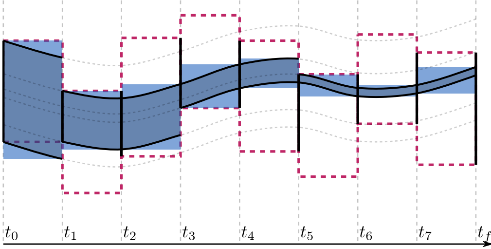
Figure 4.8: Forward integration
