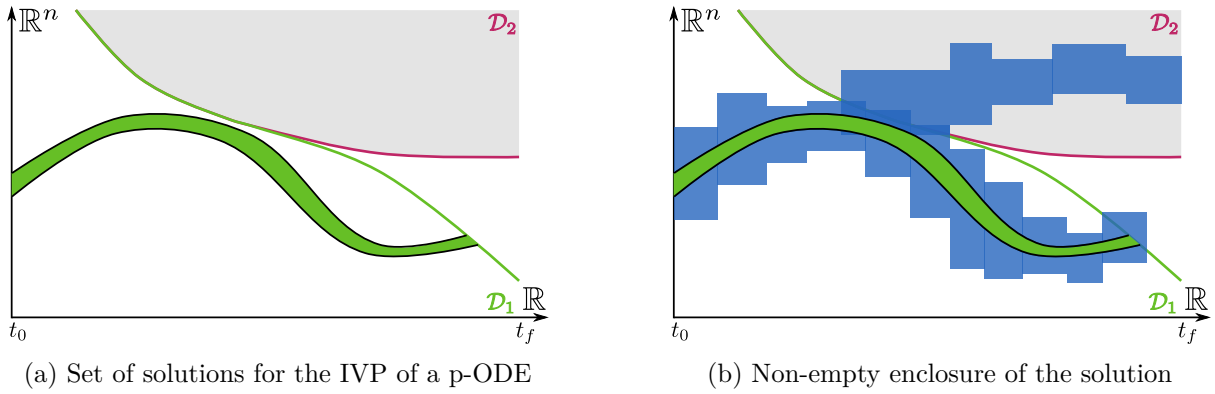
Figure 6.2: Enclosure of an unfeasible solution at t_f
