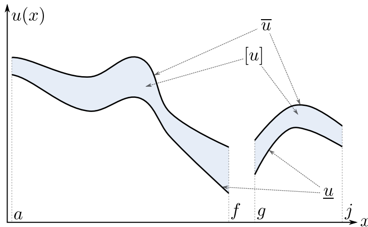
Figure 2.8: Tube [u] enclosing u
