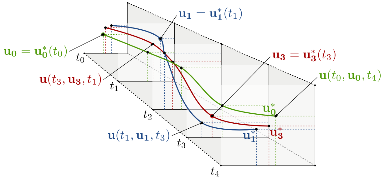
Figure 3.1: Solutions of various IVPs
