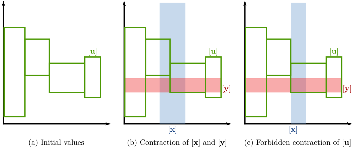
Figure 4.3: Contraction of [\mathbf{x}] and [\mathbf{y}]
