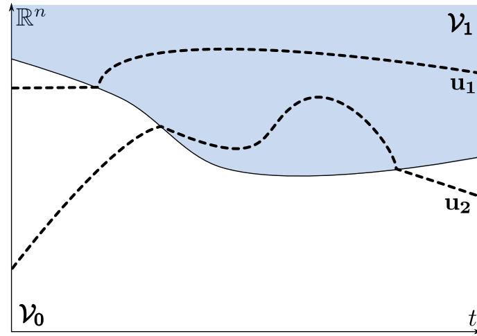
Figure 5.2: Cooperative dynamics
