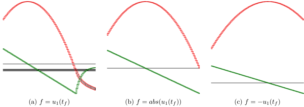
Figure 7.4: Enclosures [u_1](t) and [u_2](t) for each solution returned by the optimization process according to the objective function
