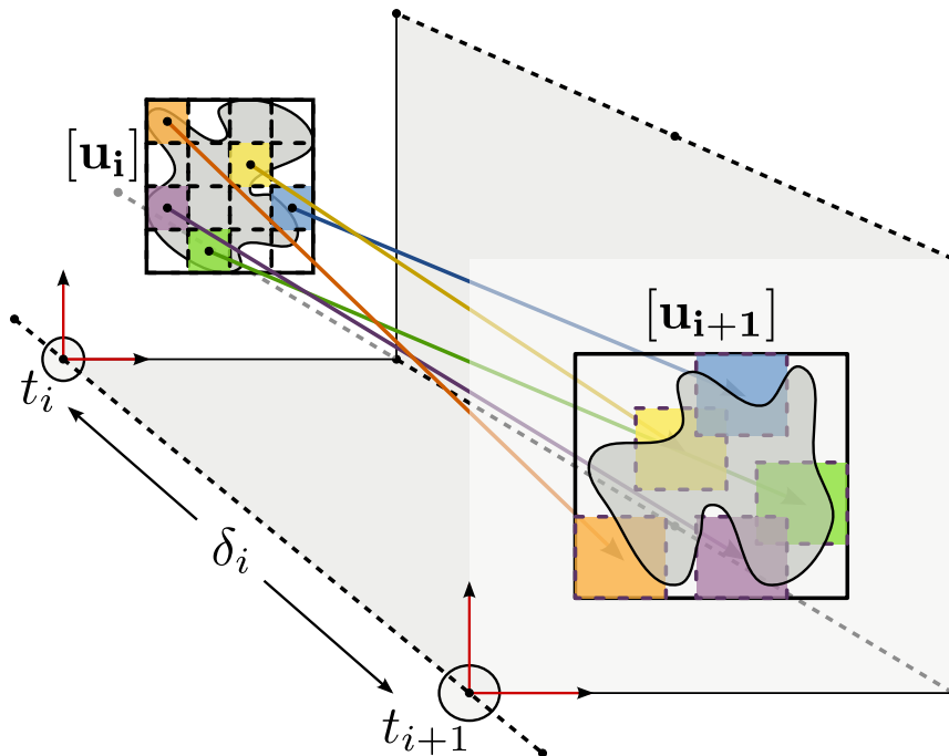
Figure 3.11: Complete piecewise evaluation on [\mathbf{u}_i]
