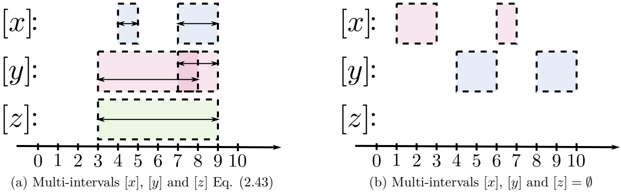
Figure 2.5: Few examples of multi-intervals
