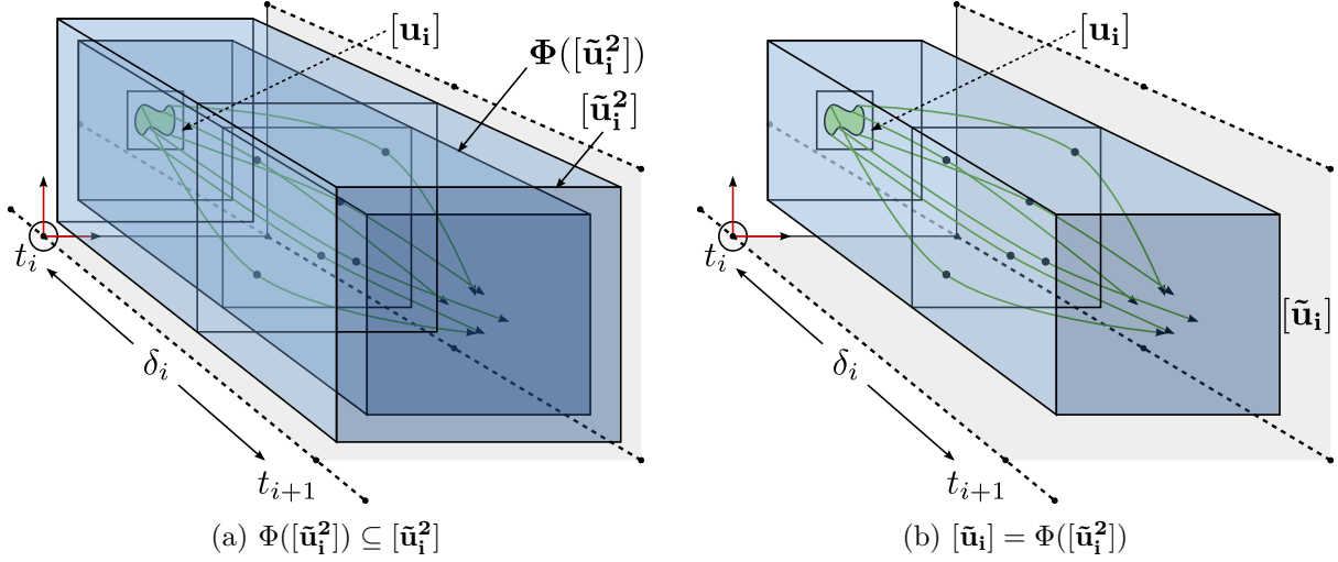
Figure 3.6: Success of the Picard iteration
