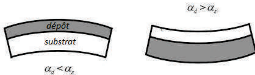
Figure I.16: Schéma des contraintes dites "thermiques" (gris = compression et blanc = tension)
