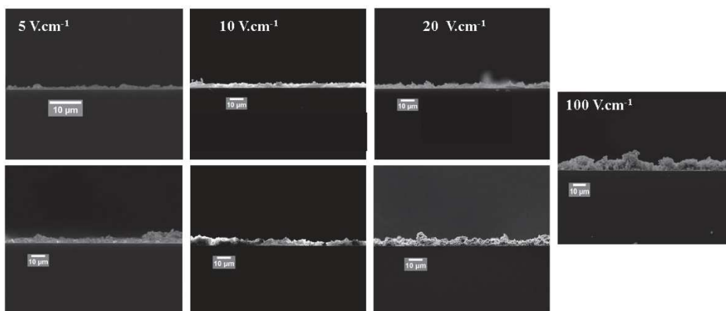
Figure 3.7: SEM cross-section micrographs of deposits obtained at 5-100 \text{V.cm}^{-1}
