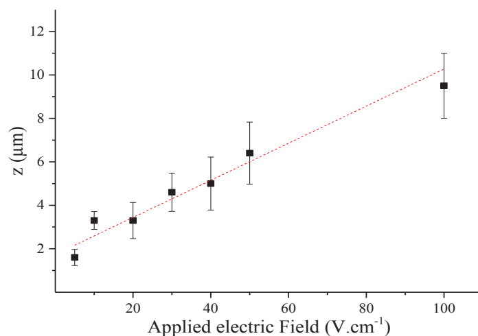
Figure 3.8: Average thickness ( z ), obtained from SEM cross section, as a function of E ( \text{V}\cdot\text{cm}^{-1} ).
