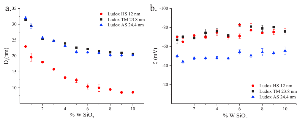
Figure 2.4: Hydrodynamic diameter ( D_h ) and zeta potential ( \zeta_p ) of SiO 2 suspension.
