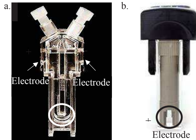
Figure 2.8: A classical micro-electrophoresis measurement cell: folded capillary cell and dip cell
