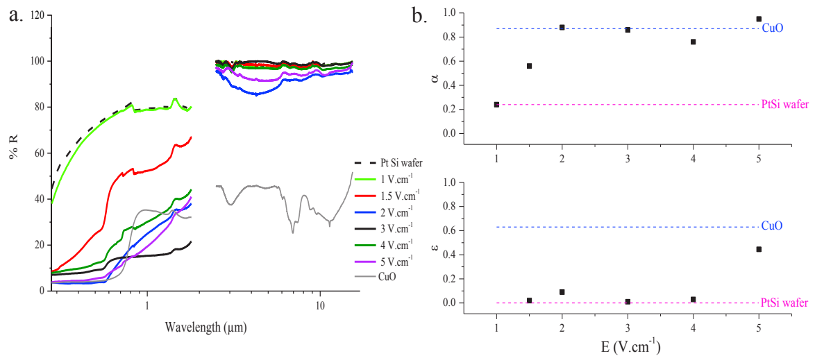
Figure 4.17: Total reflectance (%R) of the obtained deposits at 1, 1.5, 2, 3, 4, 5 V.cm -1 .
