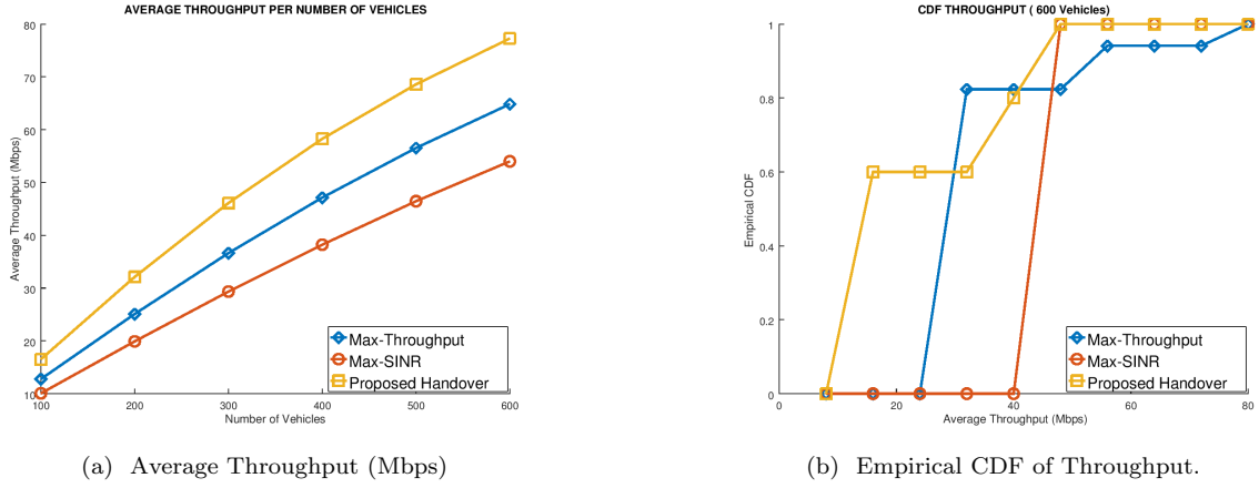
Figure 6.4: (a) Average Throughput in Mbps per Number of vehicles and (b) Empirical CDF of Throughput ( 600 Vehicles).
