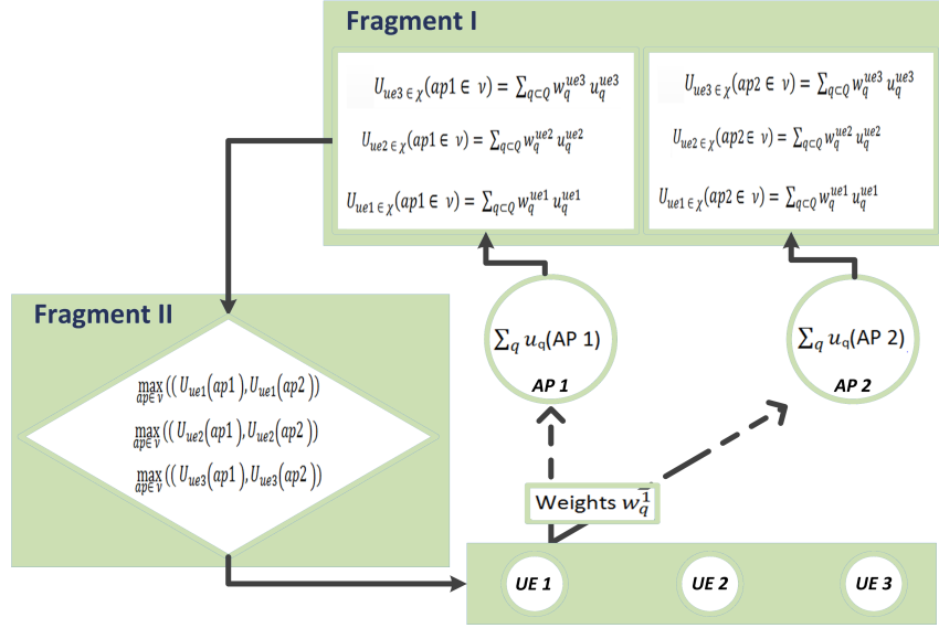
Figure 4.4: A matching example of three UEs and two APs.
