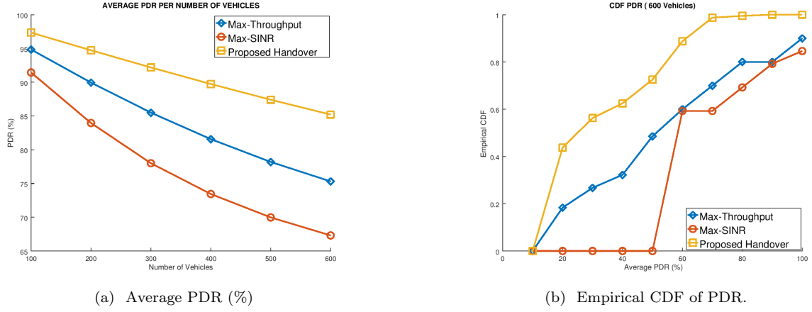
Figure 6.6: (a) Average PDR per Number of vehicles and (b) Empirical CDF of PDR( 600 Vehicles).
