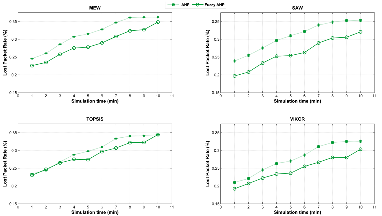
Figure 5.6: AHP and FAHP Performances of Packet Loss Rate over Time in Streaming Traffic.
