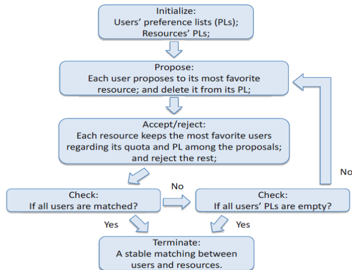
Figure 4.2: Deferred Acceptance (DA) Algorithm Gu et al. (2015).
