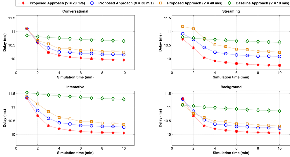
Figure 5.17: Behaviour of Delay over Time using Utility-based scheme in different speed scenarios for all traffics.
