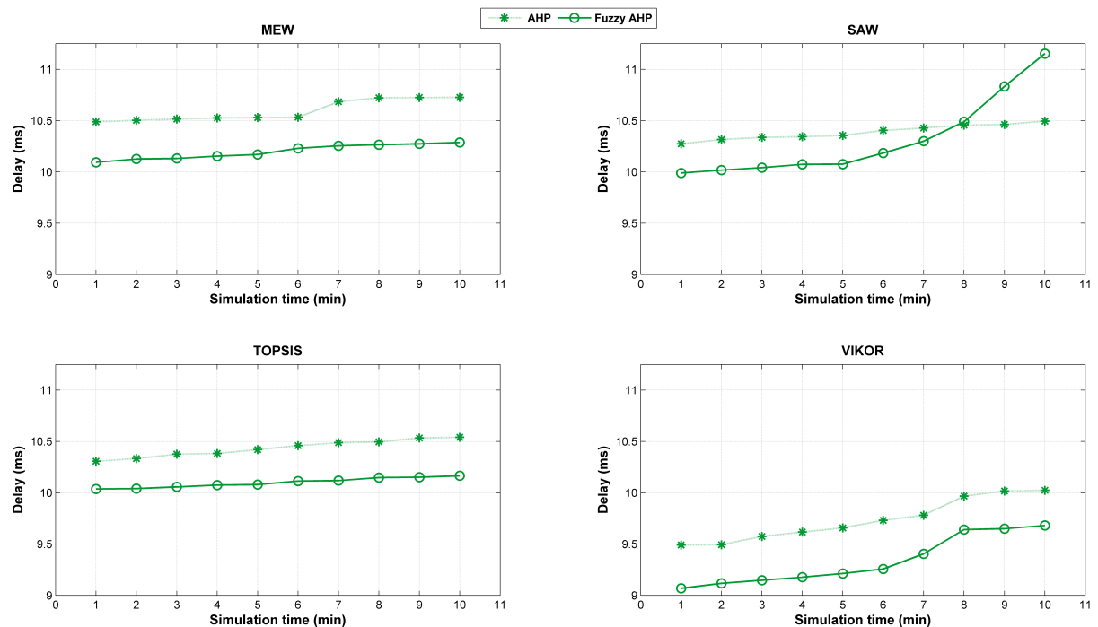
Figure 5.2: AHP and FAHP Performances of Delay over Time in Streamig Traffic.
