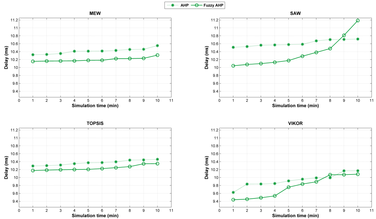
Figure 5.4: AHP and FAHP Performances of Delay over Time in Background Traffic.
