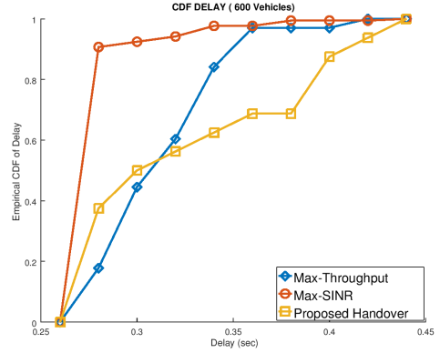
(b) Empirical CDF of Delay.
