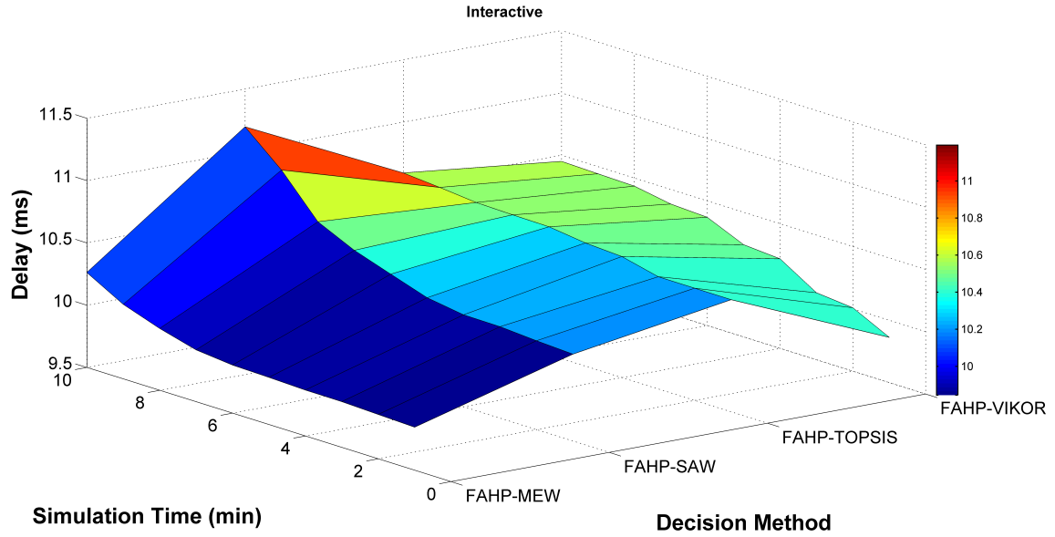
Figure 5.13: Delay Performance over Time in Interactive Traffic using FAHP.
