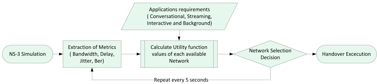
Figure 4.3: Utility-based Algorithm Block.
