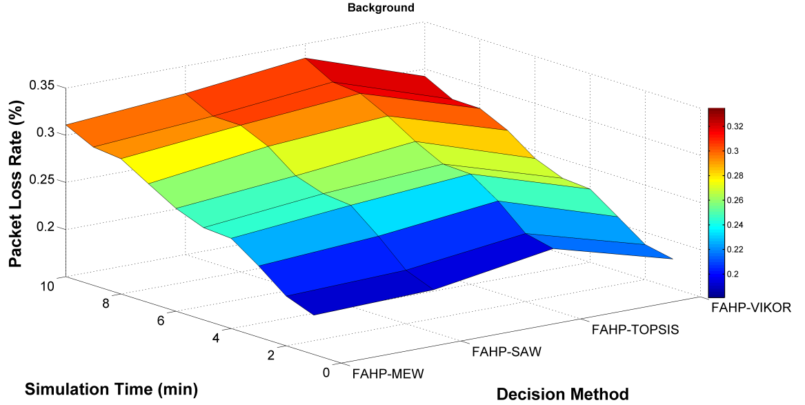
Figure 5.16: Packet Loss Performance over Time in Background Traffic using FAHP.
