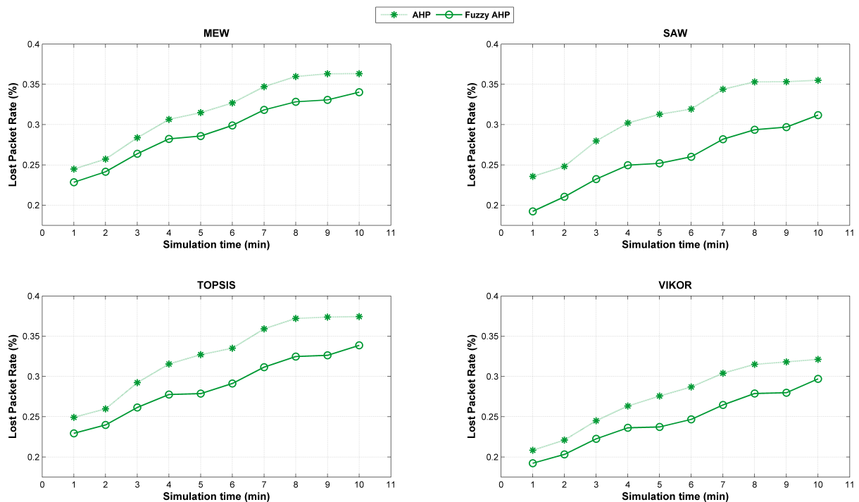
Figure 5.7: AHP and FAHP Performances of Packet Loss over Time in Interactive Traffic.
