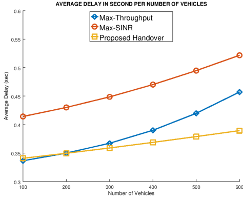
(a) Average Delay (sec)
