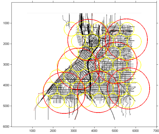
Figure 6.3: LTE Base stations mapping in the simulated area.
