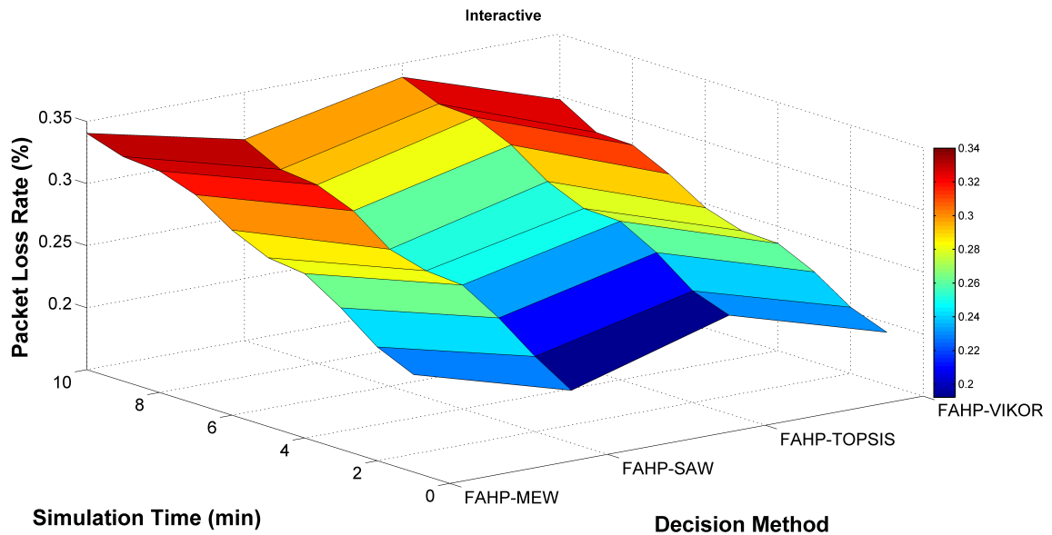
Figure 5.14: Packet Loss Performance over Time in Interactive Traffic using FAHP.
