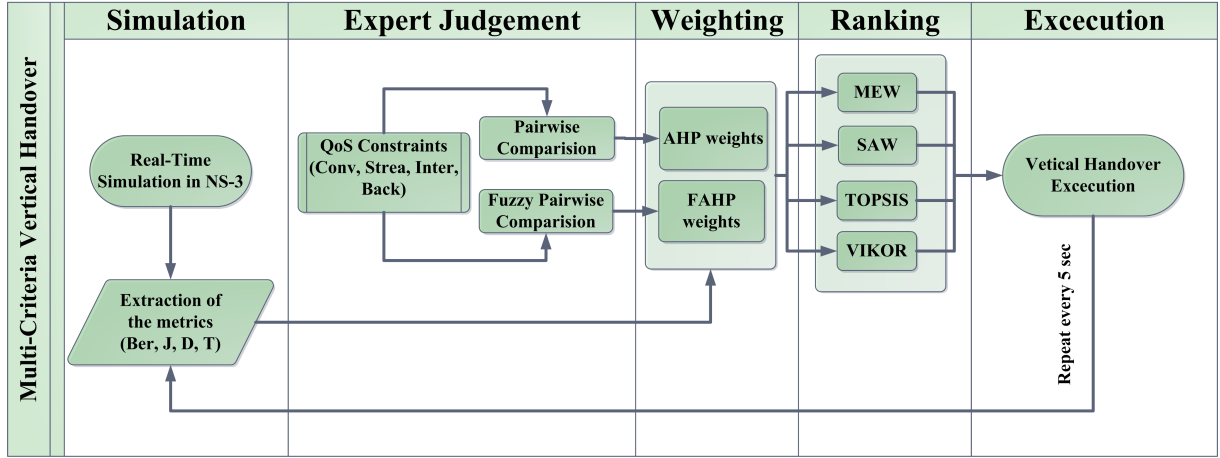
Figure 3.2: MADM-based Algorithm Block
