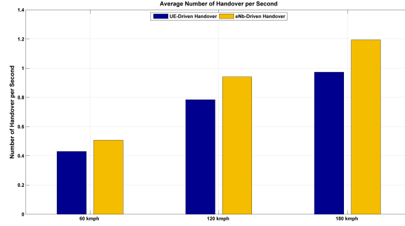
Figure 5.22: Average Number of Handover per Second using User-Driven Handover Scheme in LTE Macro/Femto Cells in Streaming traffic.
