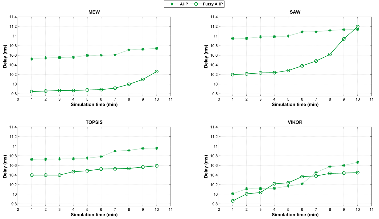
Figure 5.3: AHP and FAHP Performances of Delay over Time in Interactive Traffic.
