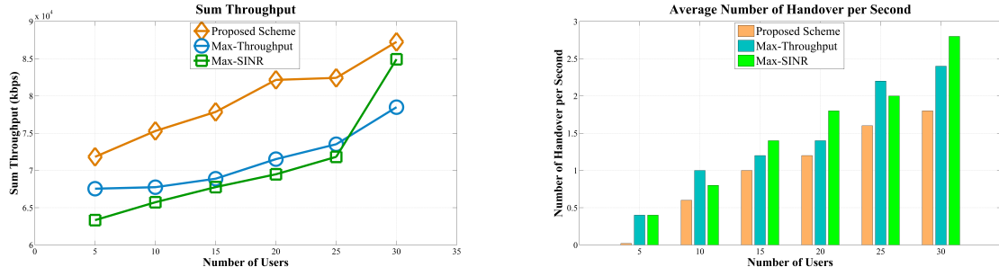
(a) Empirical Sum Throughput as a function of number of users. (b) Average Number of Handover per Second as a function of number of users.
