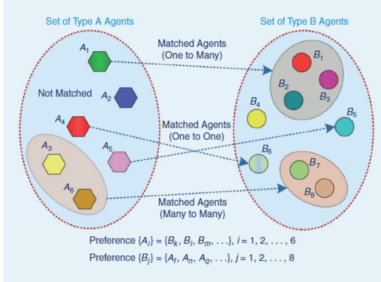
Figure 4.1: The general configuration of the matching structure Bayat et al. (2016).
