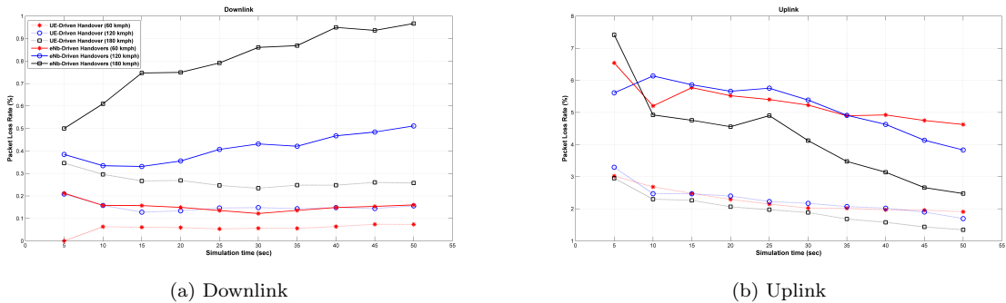
Figure 5.21: Behaviour of Packet Loss Rate over Time using User-Driven Handover Scheme in LTE Macro/Femto Cells in Streaming traffic.
