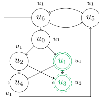
(b) 1 st iteration: propagation of u_1
