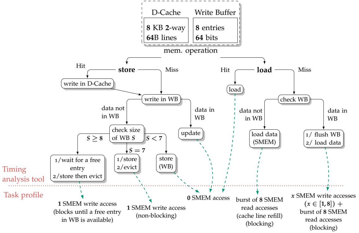
Figure 6.5: Occurrence of accesses from data cache and write butter to shared memory
