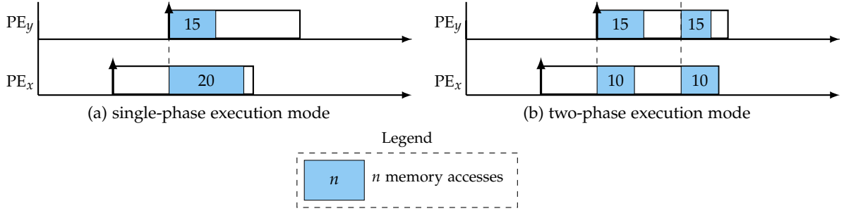
Figure 7.1: Pessimism in single-phase and two-phase execution models
