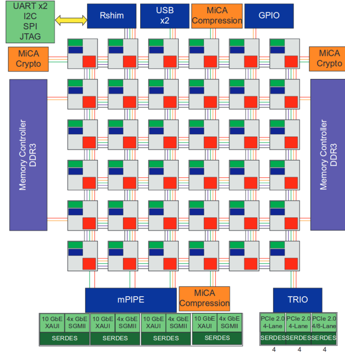
Figure 2.11: Overview of the Tileria TILE-Gx36 processor (taken from [Til12])
