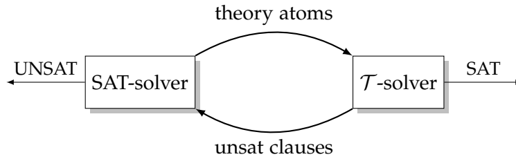
Figure 4.3: General DPLL( \mathcal{T} ) framework
