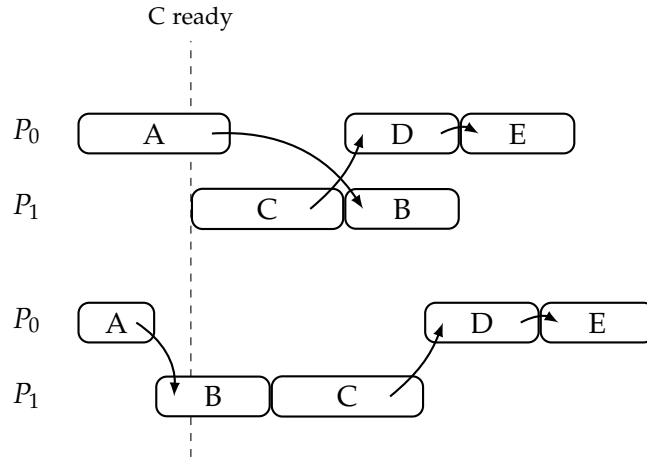
Figure 2.9: Scheduling anomaly
