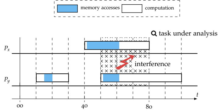
Figure 5.3: Interference from tasks on core P_y on the task on core P_x , where P_y, P_x \in \Pi and P_y \neq P_x . Only overlapping tasks mutually interfere.
