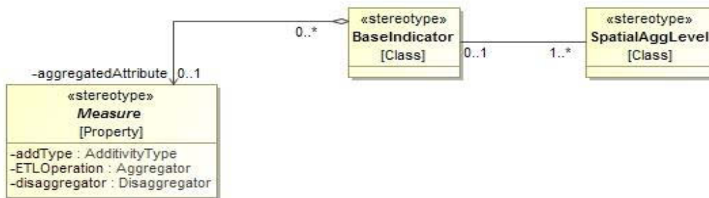
Figure 4-9: Indicator-level dependency
