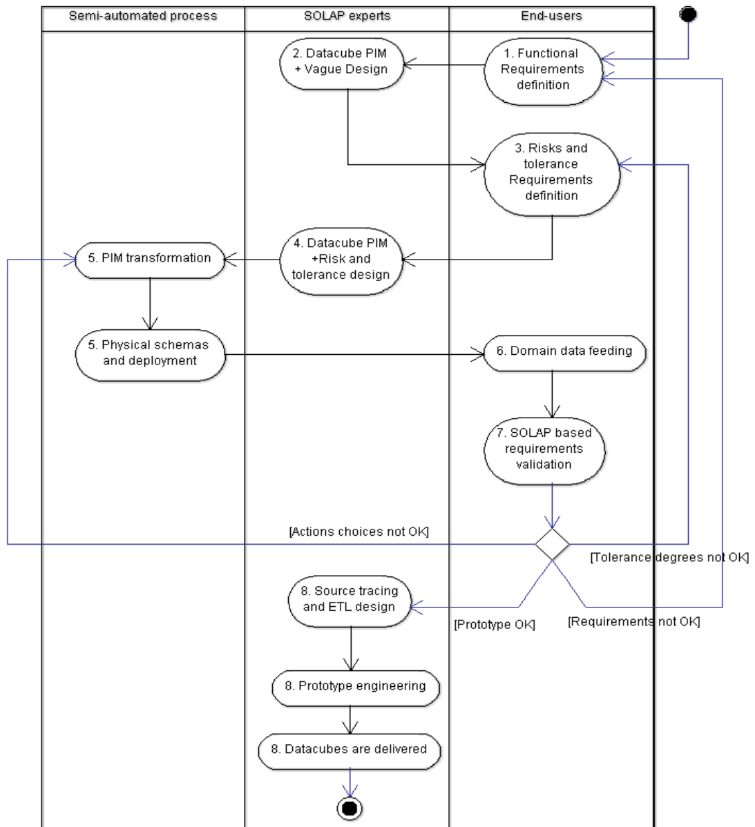
Figure 4-4: RADSOLAP method
