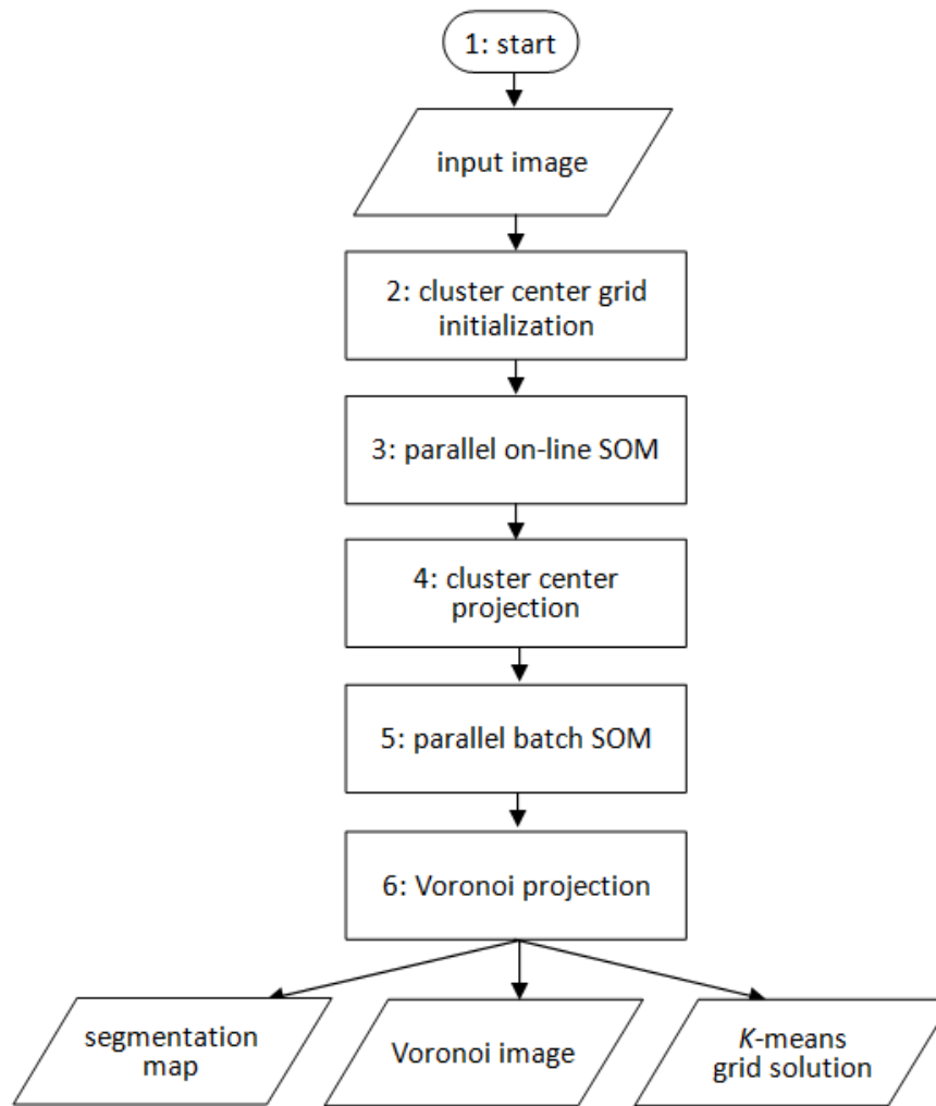
FIGURE 4.7: Flowchart of the SPASM algorithm.
