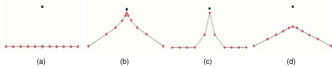
FIGURE 2.1: A single SOM iteration with one-dimensional neural network. The red circles represent neurons while the black dots represent input data points. (a) Initial configuration; (b) \alpha = 0.9, \sigma = 4 ; (c) \alpha = 0.9, \sigma = 1 ; (d) \alpha = 0.5, \sigma = 4 .
