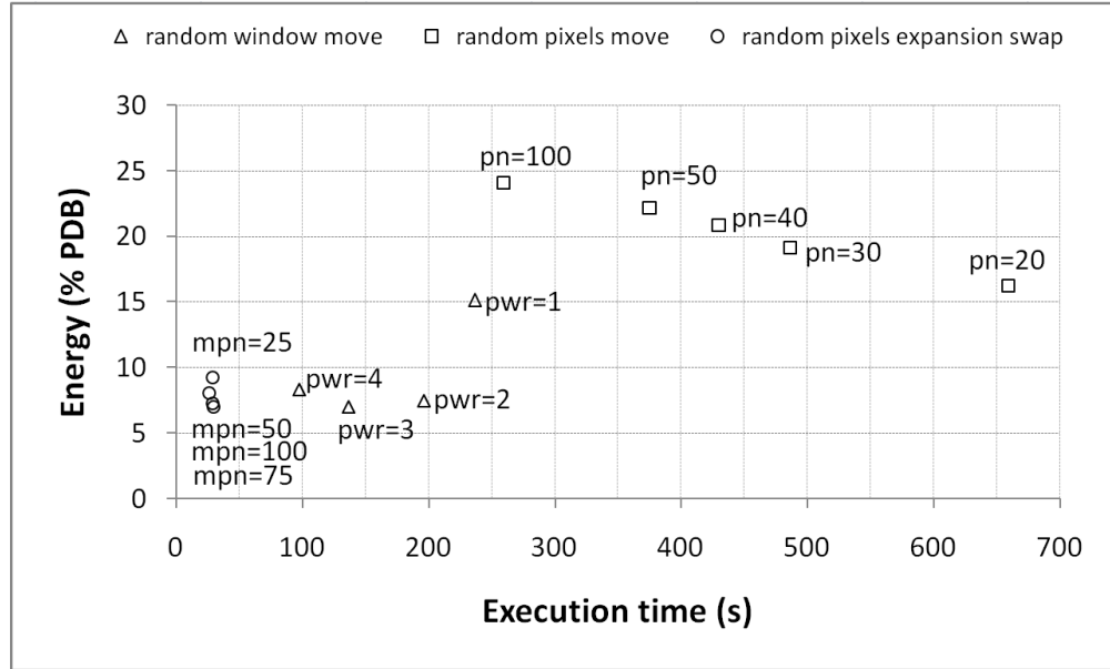
FIGURE 7.1: DLS with single operator on the Tsukuba benchmark. The x -axis shows execution time and the y -axis shows the %PDB value computed according to the lowest energy found by the TRW approach [WJW05, SZS + 08]. All the results are mean values over 10 runs. Acronyms: “pwr” stands for pickedWindowRadiu ; “pn” stands for pickedNumber ; “mpn” stands for maxPickedNumber .
