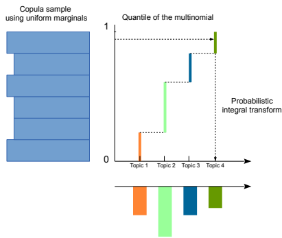
Figure 4.3: The transformation of a random variate to multinomial (or arbitrary) marginals. The arrows illustrate the generalized inverse; the histograms in y (resp. x ) axis depict the distributions of the initial (resp. transformed) samples.
