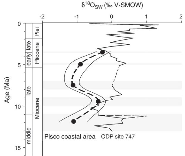
Fig. 4. Comparison between two seawater \delta^{18}O_w curves obtained from the \delta^{18}O_p values (bold black) of dolphins, seals and marine turtles (this study) and by using paired Mg/Ca and \delta^{18}O_c values (black) of benthic foraminifera (Billups and Schrag, 2002). The \delta^{18}O_{sw} value of -1.1\% was estimated for the oldest site (Cerro la Bruja) using \delta^{18}O_p values of marine turtles. Shaded areas represent the uncertainties associated with the geological ages of the Pisco localities.
