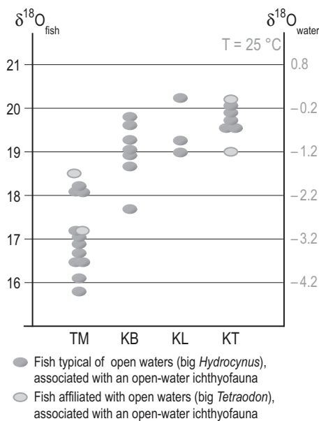
Figure 3. \delta^{18}\text{O}_{\text{fish}} of open water fish teeth from Toros-Menalla (TM), Kossom Bougoudi (KB), Kolle (KL), and Koro Toro (KT), all located in Djurab Desert, northern Chad. Values of \delta^{18}\text{O}_{\text{water}} of corresponding water are given for 25 °C according to fractionation equation \delta^{18}\text{O}_{\text{water}} = \delta^{18}\text{O}_{\text{fish}} - 25.9 + 7/4.38 (from Kolodny et al., 1983).
