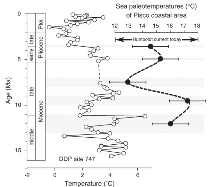
Fig. 5. Comparison between two seawater temperature curves, the first one obtained from the \delta^{18}O_p values (bold black) of dolphins, seals, turtles and sharks (this study), and the second one by using paired Mg/Ca and \delta^{18}O_c values (black) of benthic foraminifera (Billups and Schrag, 2002). Shaded areas represent the uncertainties associated with the geological ages of the Pisco localities.
