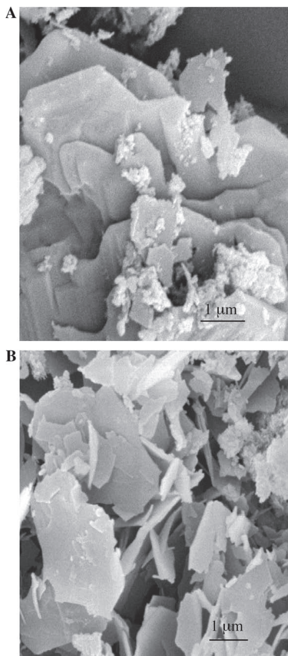
Fig. 2. Photomicrograph by Scanning Electron Microscopy of inorganically precipitated crystals of carbonate-bearing hydroxyapatite. (A) HAP crystals precipitated at 10 ^{\circ}\text{C} (magnification of 9000 \times ). (B) HAP crystals precipitated at 37 ^{\circ}\text{C} (magnification of 5000 \times ).
