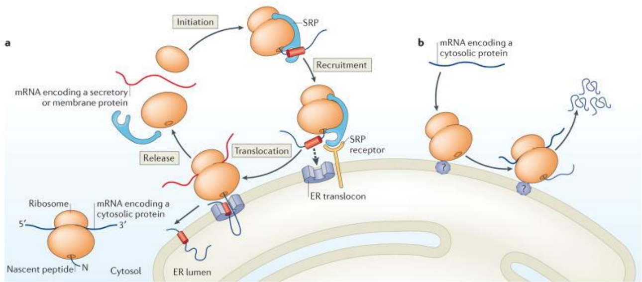
Figure 30. Model for translational compartmentalization.
