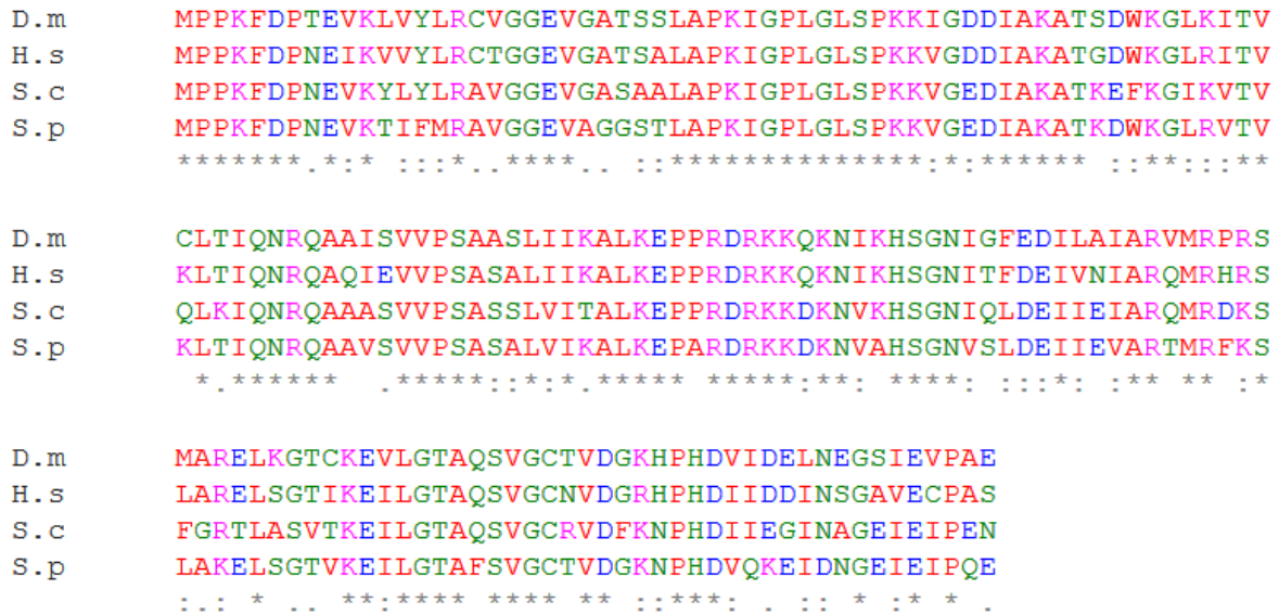
Figure 41. Alignment of uL11 protein sequence among eukaryotes. The alignment was realized with Clustal Omega v1.2.4. D.m, Drosophila melanogaster ; H.s, Homo sapiens ; S.c Saccharomyces cerevisiae ; S.p, Schizosaccharomyces pombe .
