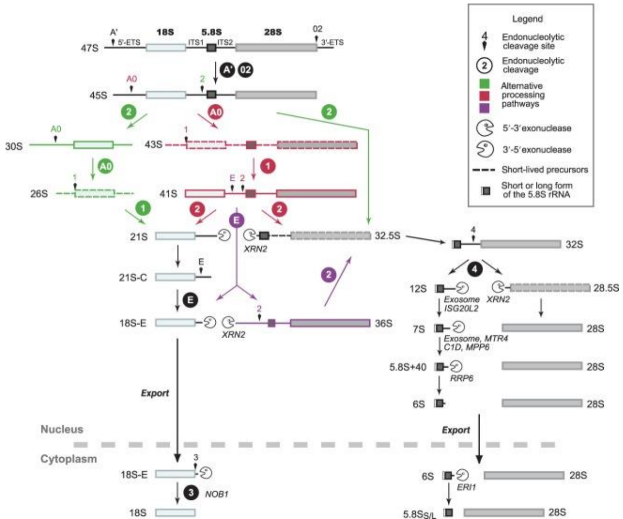
Figure 9. Pre-ribosomal RNA processing in mammalian cells.
