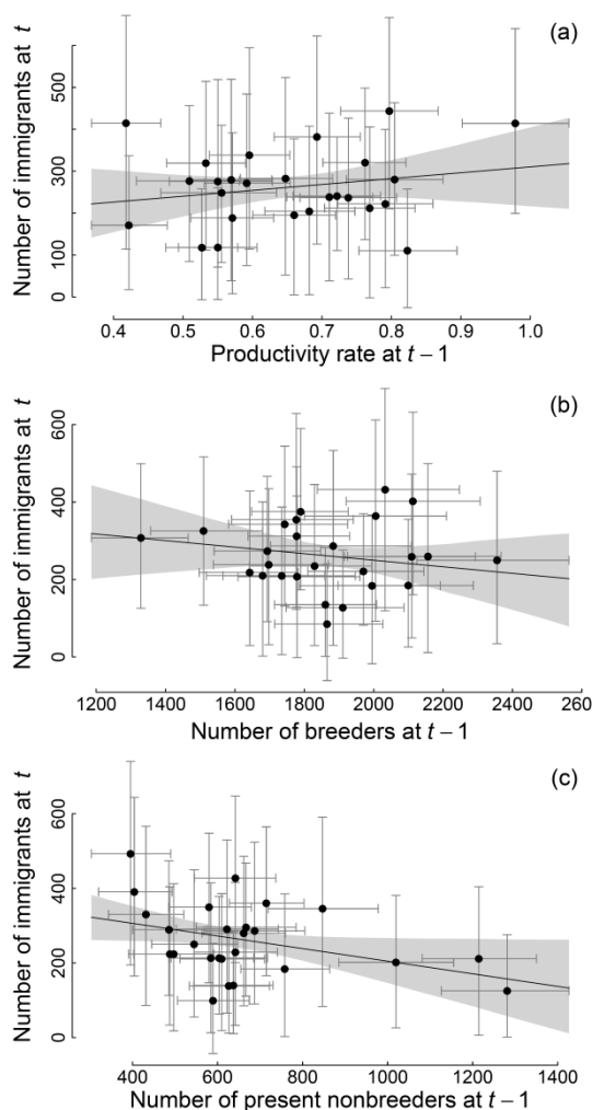
Figure C.5.7. Partial residual plots of the relationships between the number of immigrants in year t and (a) productivity at t-1 , (b) number of breeders at t-1 , (c) number of nonbreeders present at t-1 . The partial correlation was (a) 0.148 [-0.125,0.413], (b) -0.140 [-0.407, 0.135], and (c) -0.278 [-0.525,0.014]. See further details in Materials and Methods , and partial correlation values in Results . Specifications are the same as for Fig. C.5.5.
