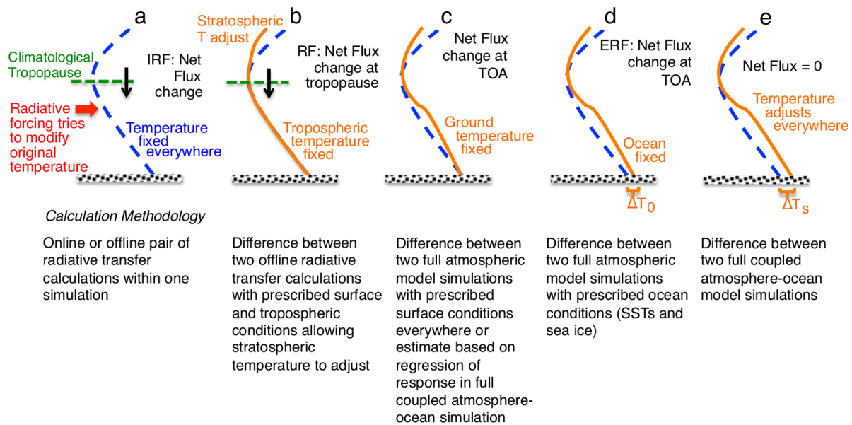
Figure 5.15: Schematic illustrating the difference between instantaneous (IRF), effective (ERF), and other types of radiative forcing (RF). Graphic extracted from Myhre et al. [2013] with the following caption: "Cartoon comparing (a) instantaneous RF, (b) RF, which allows stratospheric temperature to adjust, (c) flux change when the surface temperature is fixed over the whole Earth (a method of calculating ERF), (d) the ERF calculated allowing atmospheric and land temperature to adjust while ocean conditions are fixed and (e) the equilibrium response to the climate forcing agent. The methodology for calculation of each type of forcing is also outlined. \Delta T_0 represents the land temperature response, while \Delta T_S is the full surface temperature response."
