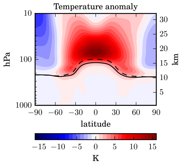
Figure 5.3: Latitude-height cross-section of the zonal and annual mean temperature anomaly (in K) in the STANDARD experiment relative to the CONTROL experiment.
