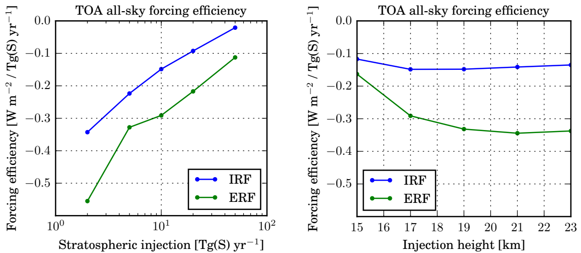
Figure 5.17: Global mean IRF and ERF efficiency in the experiments with different injection magnitudes (left) and different injection heights (right). The forcings were averaged over the years 4, 5, and 6 of the simulations in order to reduce the effect of inter-annual variability.
