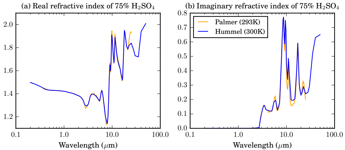
Figure 2.2: Real (a) and imaginary (b) refractive index of 75 % sulphuric acid solution in water. The values from Hummel et al. [1988] (blue lines) were used for the computation of aerosol optical properties in the LMDZ-S3A model. Values from Palmer and Williams [1975] (orange lines) were used in other models [e.g. English et al., 2012].
