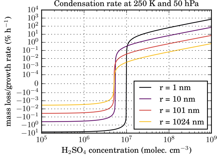
Figure 3.4: Mass growth rate (condensation rate relative to the particle mass, in % per hour) as a function of sulphuric acid vapour concentration for different particle radii at typical stratospheric conditions of 250 K and 50 hPa. A negative growth rate corresponds to evaporation. Note that the logarithmic y scale is linear between -10^{-4} and +10^{-4} % h -1 .
