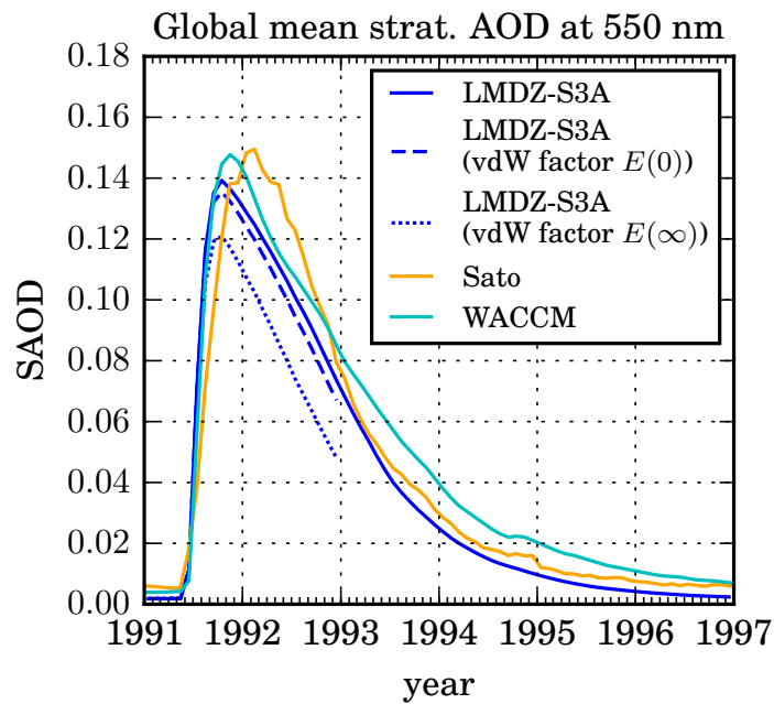
Figure 4.12: Evolution of the global mean stratospheric aerosol optical depth (SAOD) at 550 nm modelled with LMDZ-S3A compared to the climatology from Sato [2012] and to SAOD simulated with WACCM by Mills et al. [2016]. The dashed (resp. dotted) line shows the model result for coagulation enhanced by the continuum regime van der Waals enhancement factor E(0) (resp. the kinetic regime enhancement factor E(\infty) ).
