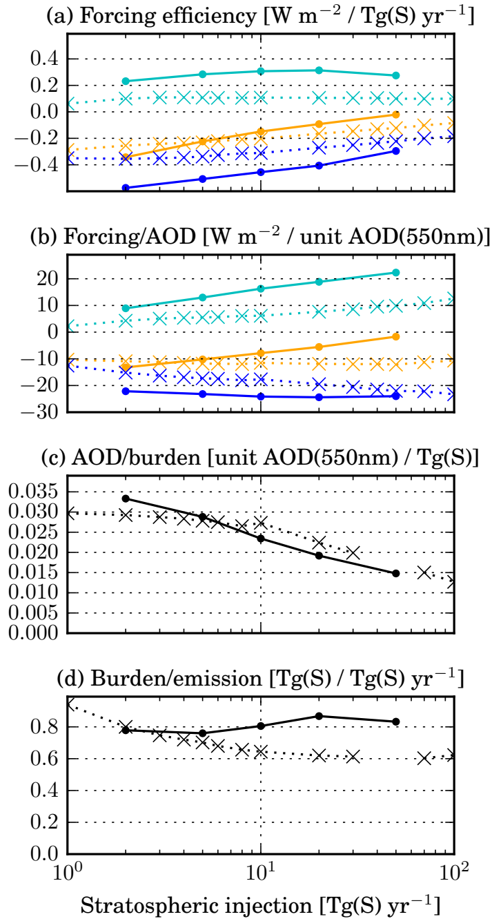
Figure 5.7: (a) Forcing efficiency (i.e., ratio of global mean instantaneous radiative forcing by the global sulphur injection rate) for the x_{\text{TGS}} simulations with different injection rates. The SW component is shown in dark blue, the LW component in light blue and the net flux in orange. Panels (b) to (d) show the decomposition of the forcing efficiency as described in the text (see Eq. 5.1). The solid lines show the results from the described LMDZ-S3A simulations, while the crosses show results from a previous study by Niemeier and Timmreck [2015].
