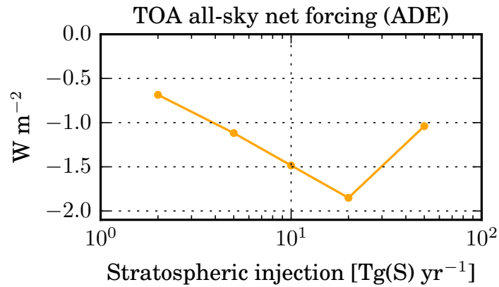
Figure 5.5: Global mean instantaneous net radiative forcing (aerosol direct effect = ADE) at the top of the atmosphere (TOA) in \text{W m}^{-2} for the x\_TGS experiments with different injection rates.
