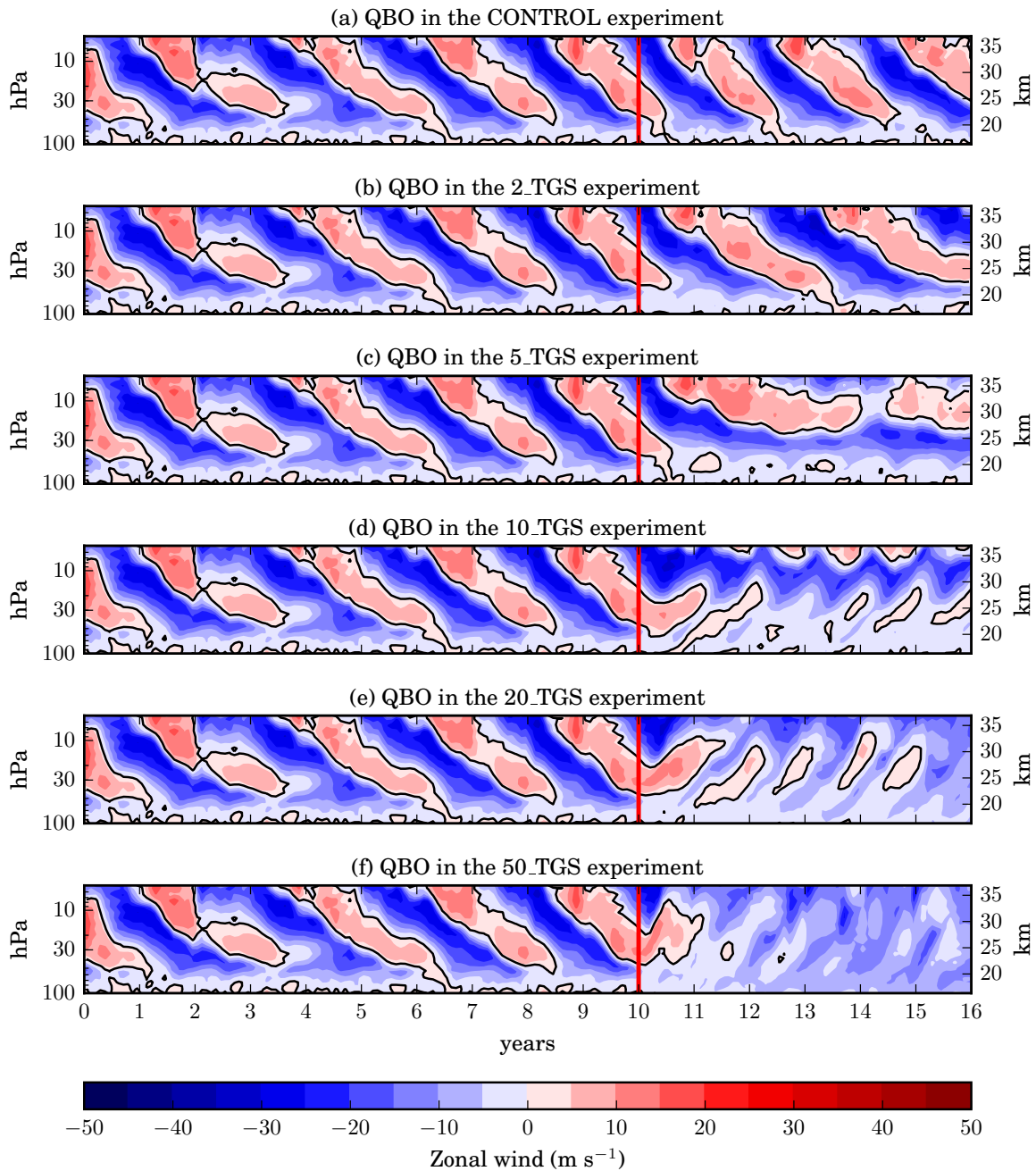
Figure 5.14: Temporal evolution of the vertical profiles of zonal wind (in \text{m s}^{-1} ), averaged zonally and between 2^\circ\text{N} and 2^\circ\text{S} . The QBO can be seen in the alternating downward propagation of easterly (blue) and westerly (red) wind direction. All the simulations share the same background aerosol spin up period of 10 years. The onset of the continuous sulphur injections is marked by a red line.
