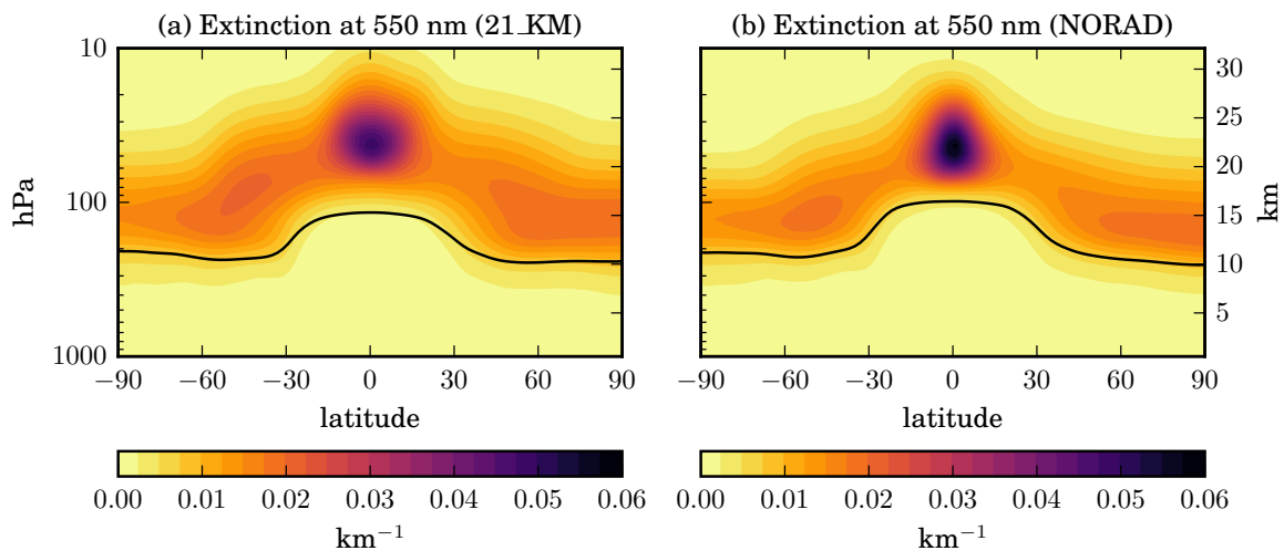
Figure 5.13: Latitude-height cross-section of the zonal and annual mean distribution of the aerosol extinction coefficient ( \text{km}^{-1} ) at 550 nm for equatorial stratospheric aerosol injections at 21 km from (a) a simulation with radiatively interactive aerosol (21_KM) and (b) a simulation with non-radiatively interactive aerosol (NORAD).
