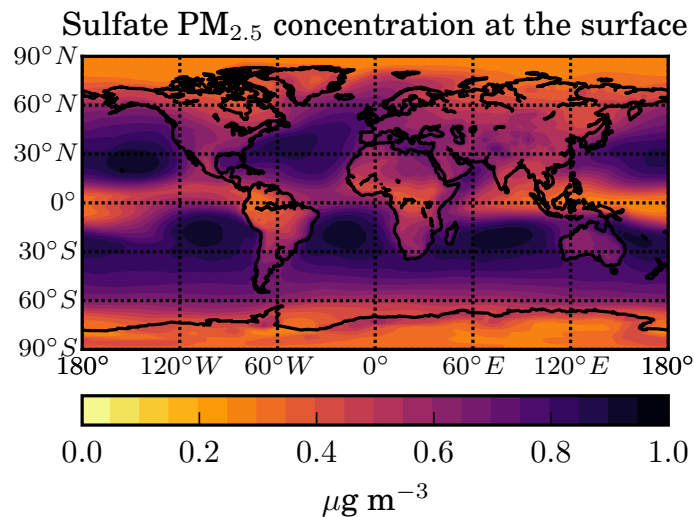
Figure 5.20: Annual mean concentration of sulphate aerosol particles ( as ammonium sulphate) of stratospheric origin with dry diameter below 2.5 \mu\text{m} at the Earth's surface (in \mu\text{g m}^{-3} ) in the STANDARD scenario.
