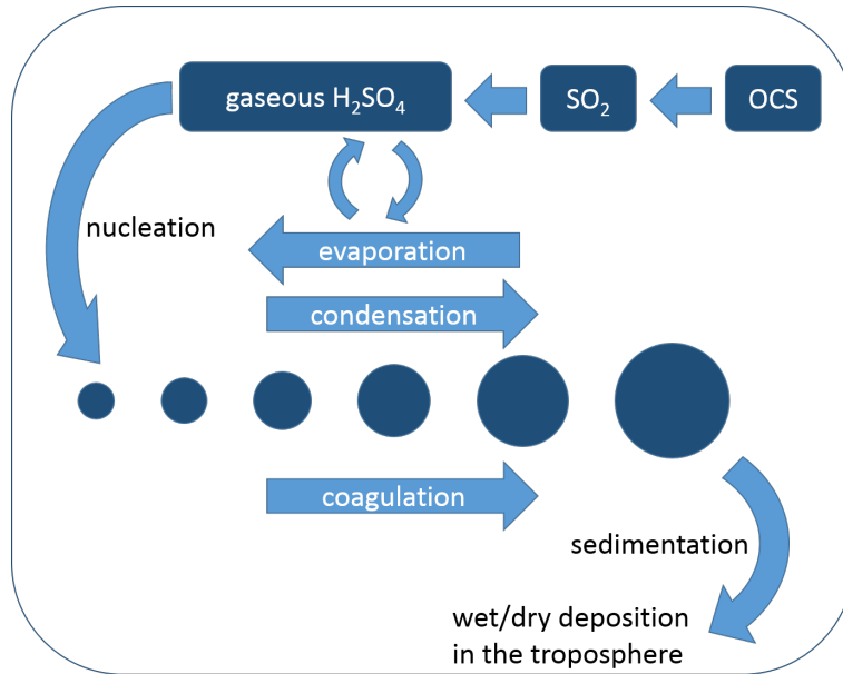
Figure 3.3: Schematic representation of the sulphur species and the processes affecting them that are represented in the LMDZ-S3A model.
