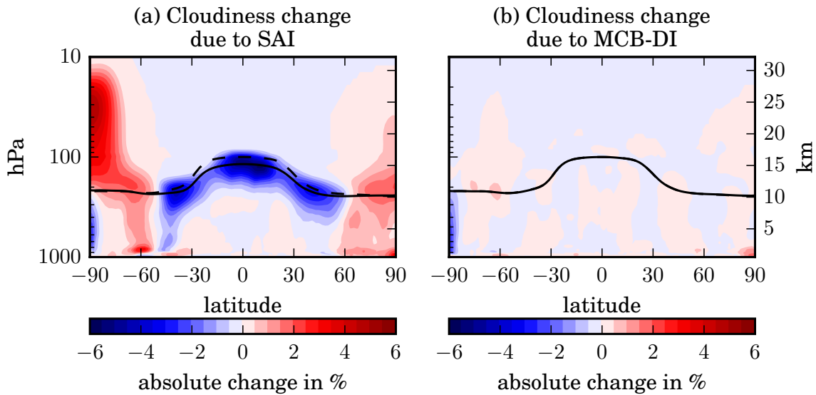
Figure 6.3: Same as Figure 6.1 but for the absolute change in cloudiness (%).
