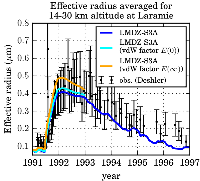
Figure 4.11: Stratospheric effective particle radius (in \mu\text{m} ) at Laramie, Wyoming ( 41^\circ\text{ N} , 105^\circ\text{ W} ) as simulated by the LMDZ-S3A model and observed with optical particle counters [Deshler et al., 2003]. The light blue (resp. orange) line shows the model result for coagulation enhanced by the continuum regime van der Waals enhancement factor E(0) (resp. the kinetic regime enhancement factor E(\infty) ).
