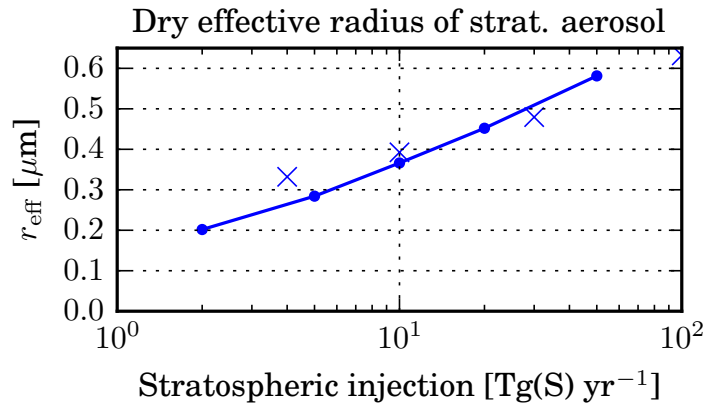
Figure 5.8: Global mean dry effective radius (in \mu\text{m} ) of the stratospheric sulphate aerosol as a function of sulphur injection rate ( \text{Tg S yr}^{-1} ). The solid lines show the results from the x_{\text{TGS}} experiments using LMDZ-S3A, while the crosses show results from a previous study by Niemeier and Timmreck [2015].
