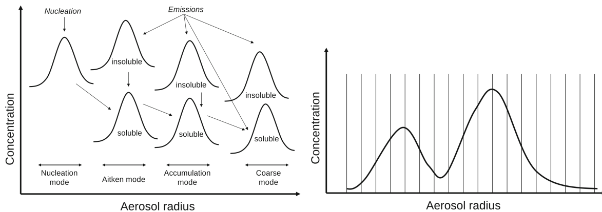
Figure 1.3: Schematic representation of the modal (left) and the sectional (right) aerosol modelling approach described in the text. Both graphics are extracted from Boucher [2015].
