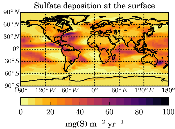
Figure 5.19: Annual mean deposition rate of sulphate aerosol of stratospheric origin at the Earth's surface (in \text{mg S m}^{-2} \text{ yr}^{-1} ) in the STANDARD scenario.
