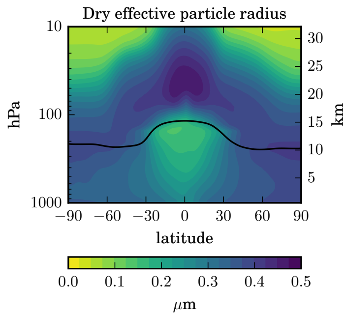
Figure 5.4: Latitude-height cross-section of the zonal and annual mean effective radius (in \mu\text{m} ) of dry sulphate particles in the STANDARD experiment. The effective radius is computed from the zonal and annual means of the aerosol volume and surface area.
