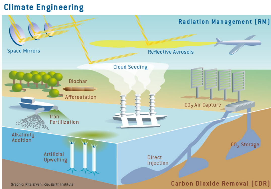
Figure 1.1: Overview of some of the proposed climate engineering techniques described in the text. Graphic taken from www.spp-climate-engineering.de .
