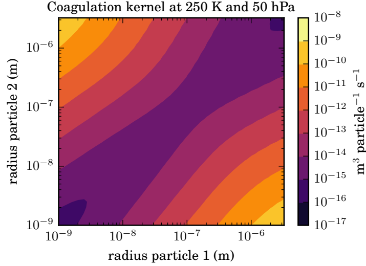
Figure 3.5: Brownian coagulation kernel for particles in the size range covered by the LMDZ-S3A model at typical stratospheric conditions of 250 K and 50 hPa.
