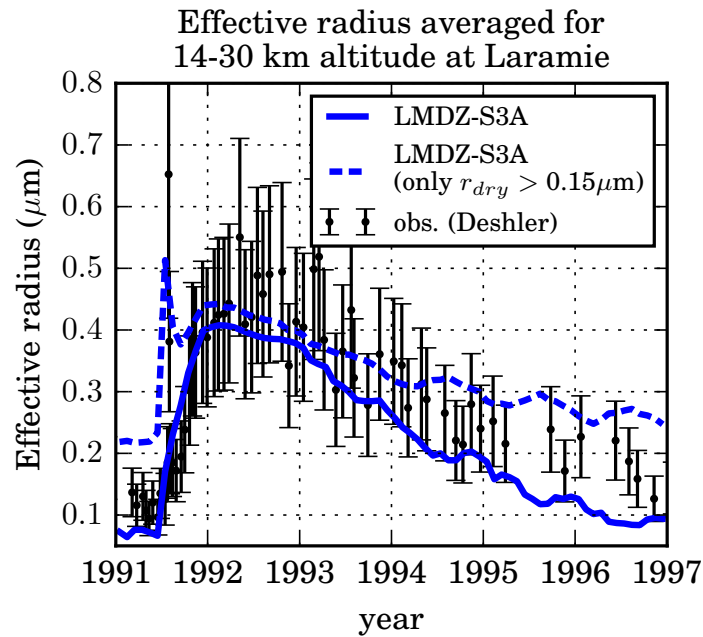
Figure 4.8: Stratospheric effective particle radius (in \mu\text{m} ) at Laramie, Wyoming ( 41^\circ\text{ N} , 105^\circ\text{ W} ) as simulated by the LMDZ-S3A model and observed with optical particle counters [Deshler et al., 2003]. Error bars of the measurements were determined from the 40 % uncertainty in aerosol surface area A and volume V assuming a correlation coefficient of 0.5 between A at different altitudes, V at different altitude and A and V at the same altitude.
