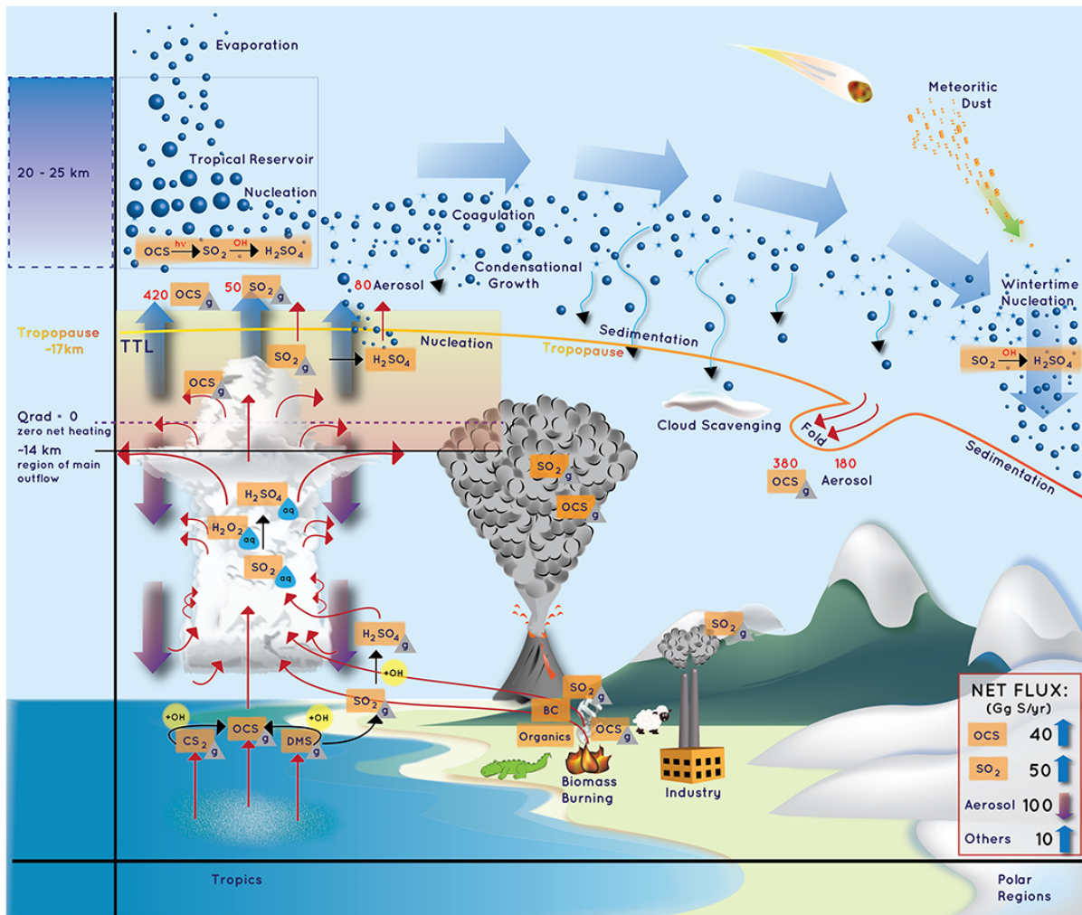
Figure 1.2: Schematic extracted from Kremser et al. [2016] with the following caption: "Schematic of the relevant processes that govern the stratospheric aerosol life cycle and distribution. The large blue arrows indicate the large-scale circulation, while the red arrows indicate transport processes. The black arrows indicate chemical conversions between compounds. The different chemical species are marked as either gas phase (grey triangle) or aqueous phase (blue drop). The blue thin arrows represent sedimentation of aerosol from the stratosphere to the troposphere. Note that due to its long tropospheric lifetime, carbonyl sulfide (OCS) does not necessarily require deep convection to be transported into the TTL (as shown in the figure). The red numbers represent the flux of OCS and sulfur dioxide (SO 2 ) as well as the flux of aerosol in Gg S/yr based on model simulations from Sheng et al. [2015]. The approximate net flux of sulfur containing compounds across the tropopause is shown in the grey box [Sheng et al., 2015], where the 10 Gg S/yr contribution from others can be mostly attributed to dimethyl sulfide (DMS) and hydrogen sulfide (H 2 S). Other chemical compounds shown in this figure are carbon disulfide (CS 2 ), sulfuric acid (H 2 SO 4 ), and black carbon (BC). [...]"
