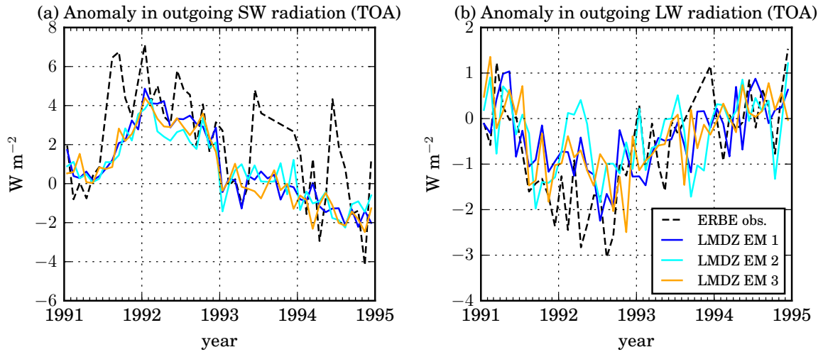
Figure 4.1: Comparison of the observed and the simulated top-of-the-atmosphere (TOA) anomaly in the outgoing (a) SW and (b) LW radiation following the eruption of Mount Pinatubo in June 1991. The black dashed line shows the ERBE satellite measurements, while the coloured solid lines show model results from three different ensemble members (EM) with slightly different initial conditions.
