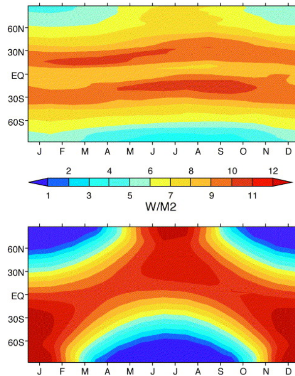
Figure 2.3: Figure extracted from Govindasamy et al. [2003] with the following caption: "Change in net long-wave radiative flux at the tropopause when CO 2 is quadrupled (top panel) with respect to the Control case and the reduction in incoming solar radiation (bottom panel) needed to compensate this forcing. Both values ( \text{W m}^{-2} ) are zonally averaged as a function of time of year. Change in solar radiation has a latitudinal and seasonal pattern markedly different from the radiative forcing of CO 2 ."
