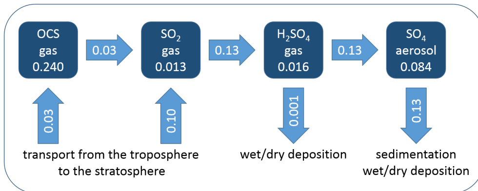
Figure 4.4: Modelled annual mean stratospheric burden (in Tg S) and fluxes (in Tg S yr -1 ) of the represented sulphur species. The values are given for steady state background conditions without any stratospheric volcanic emissions. Sedimentation and advection can take the species out of the stratosphere into the troposphere, where they can be removed by wet and dry deposition.
