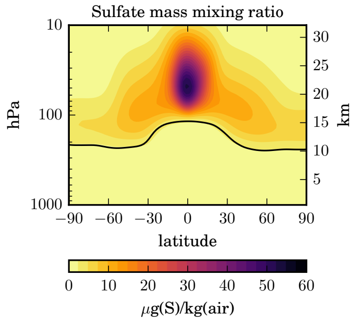
Figure 5.2: Latitude-height cross-section of the zonal and annual mean sulphate aerosol mass mixing ratio (in \mu\text{g S kg air}^{-1} ) for the STANDARD experiment.
