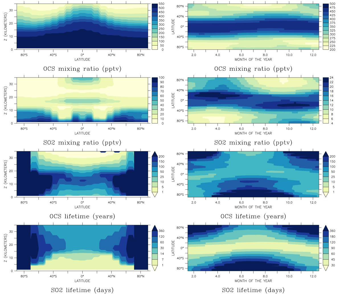
Figure 3.2: Climatological volume mixing ratios (upper half, in pptv) and lifetimes (lower half, in years or days) of OCS and SO 2 produced by the UPMC / Cambridge model and used as initial and boundary conditions for the LMDZ-S3A model. The left column shows the zonal and annual mean latitude-height distribution, while the right column shows an annual cycle of the zonal mean value at 20 km altitude.
