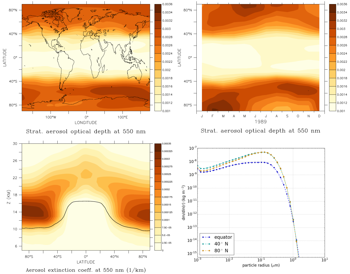
Figure 4.2: Upper left panel: Annual mean latitude-longitude distribution of the stratospheric AOD at 550 nm. Upper right panel: Zonal mean latitude-time distribution of the stratospheric AOD at 550 nm. Lower left panel: Zonal mean latitude-height distribution of stratospheric aerosol extinction coefficient ( \text{km}^{-1} ) at 550 nm. Lower right panel: Vertically integrated mass size distribution at different latitudes (in \text{kg m}^{-2} ). All variables are from the 10 th year of the simulation with no volcanic input in the stratosphere and are assumed to represent a steady state.
