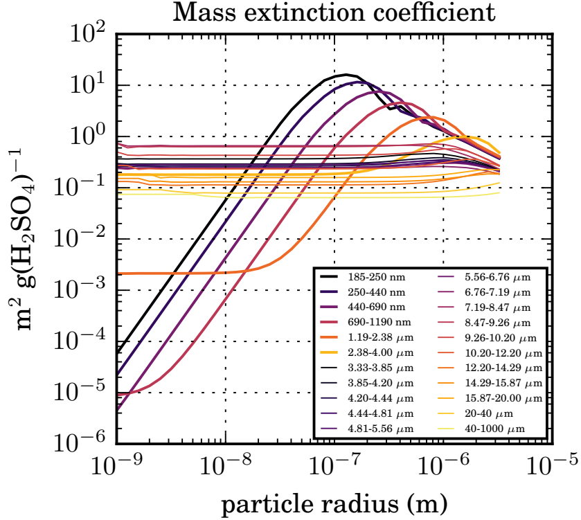
Figure 3.6: Modelled mass extinction coefficient of sulphate aerosol in \text{m}^2 \text{g}(\text{H}_2\text{SO}_4)^{-1} as a function of dry particle radius in the 6 SW (bold lines) and 16 LW (thin lines) spectral bands of the LMDZ-S3A model.
