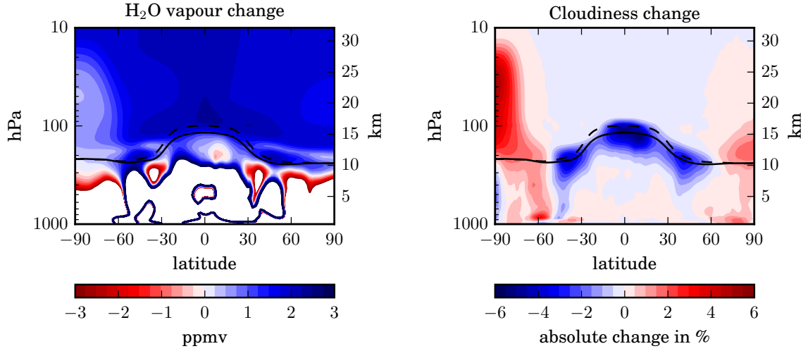
Figure 5.16: Change in water vapour mixing ratio (left, in ppmv) and in cloudiness (right, in %) in the STANDARD experiment, relative to the CONTROL experiment.
