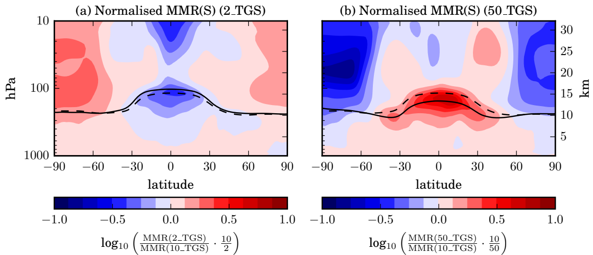
Figure 5.6: Latitude-height cross-sections of the zonal and annual mean sulphate aerosol mass mixing ratio (a) for the 2_TGS and (b) for the 50_TGS experiment, normalised by the value in the STANDARD (= 10_TGS) experiment and the ratio of the injection rates. The base-10 logarithm of the ratio is plotted as indicated below the color scale, so that positive (negative) values indicate larger (smaller) values than implied by a linear scaling. The mean tropopause level in the experiment is indicated by a solid line and the tropopause in the STANDARD simulation by a dashed line.
