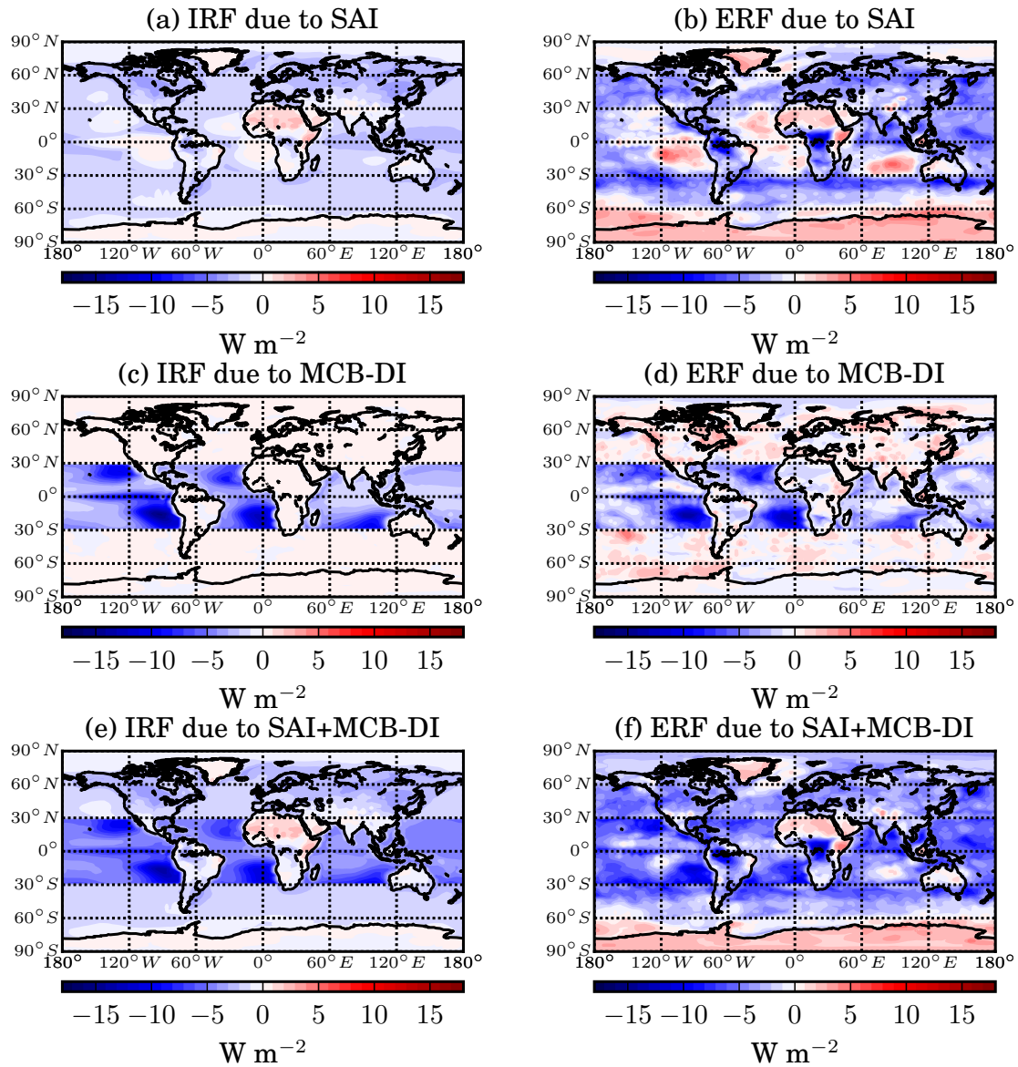
Figure 6.4: Instantaneous top-of-the-atmosphere net radiative forcing (IRF, in \text{W m}^{-2} , left column) computed from double radiation call for SAI (a), MCB-DI (c), and SAI+MCB-DI (e) and effective net radiative forcing (ERF, in \text{W m}^{-2} , right column) computed from differences in top-of-the-atmosphere radiative fluxes between parallel fixed-SST experiments for SAI (b), MCB-DI (d) and SAI+MCB-DI (f).
