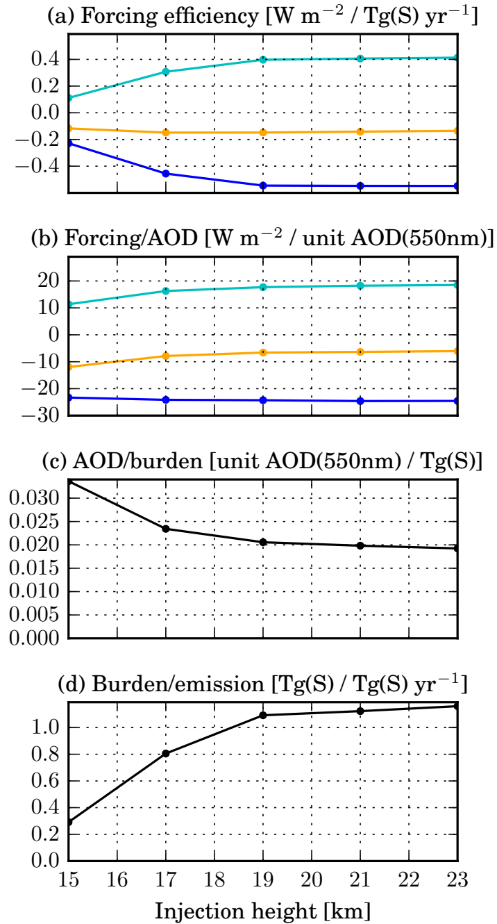
Figure 5.10: Forcing efficiency and its decomposition (as in Figure 5.7) for the z_{\text{KM}} simulations with different injection heights.
