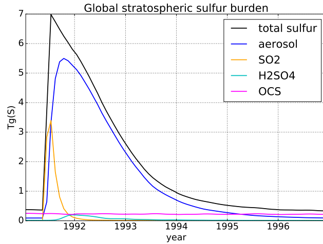
Figure 4.7: Evolution of the stratospheric sulphur burden and its distribution among the different species modelled with LMDZ-S3A for the period from January 1991 to December 1996, including the Pinatubo eruption (but no other eruptions).
