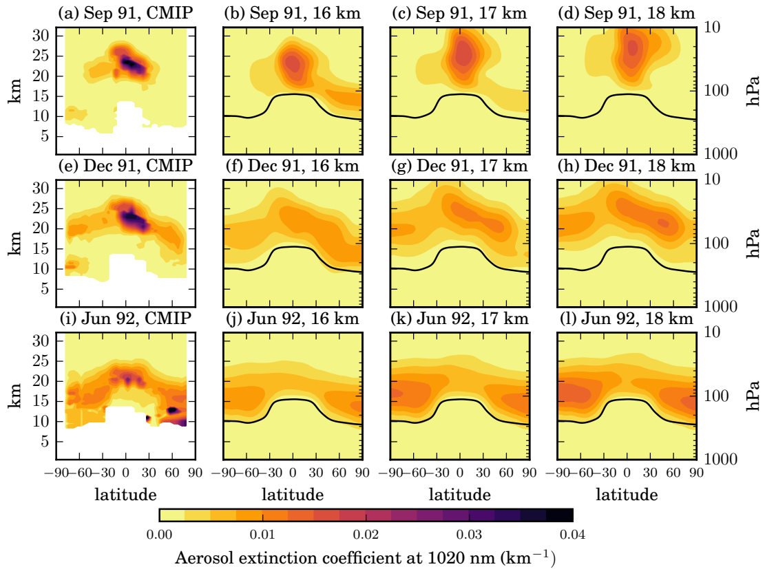
Figure 4.5: Temporal evolution of the zonal mean aerosol extinction coefficient ( \text{km}^{-1} ) at 1020 nm. Monthly mean latitude-height distributions in September 1991 (first row), December 1991 (second row) and June 1992 (third row). Observation-based CMIP6 aerosol data set (first column), simulations with emission of \text{SO}_2 at 16 km (second column), 17 km (third column) and 18 km (fourth column). The vertical axis shows the height in km and the black line indicates the modelled tropopause.
