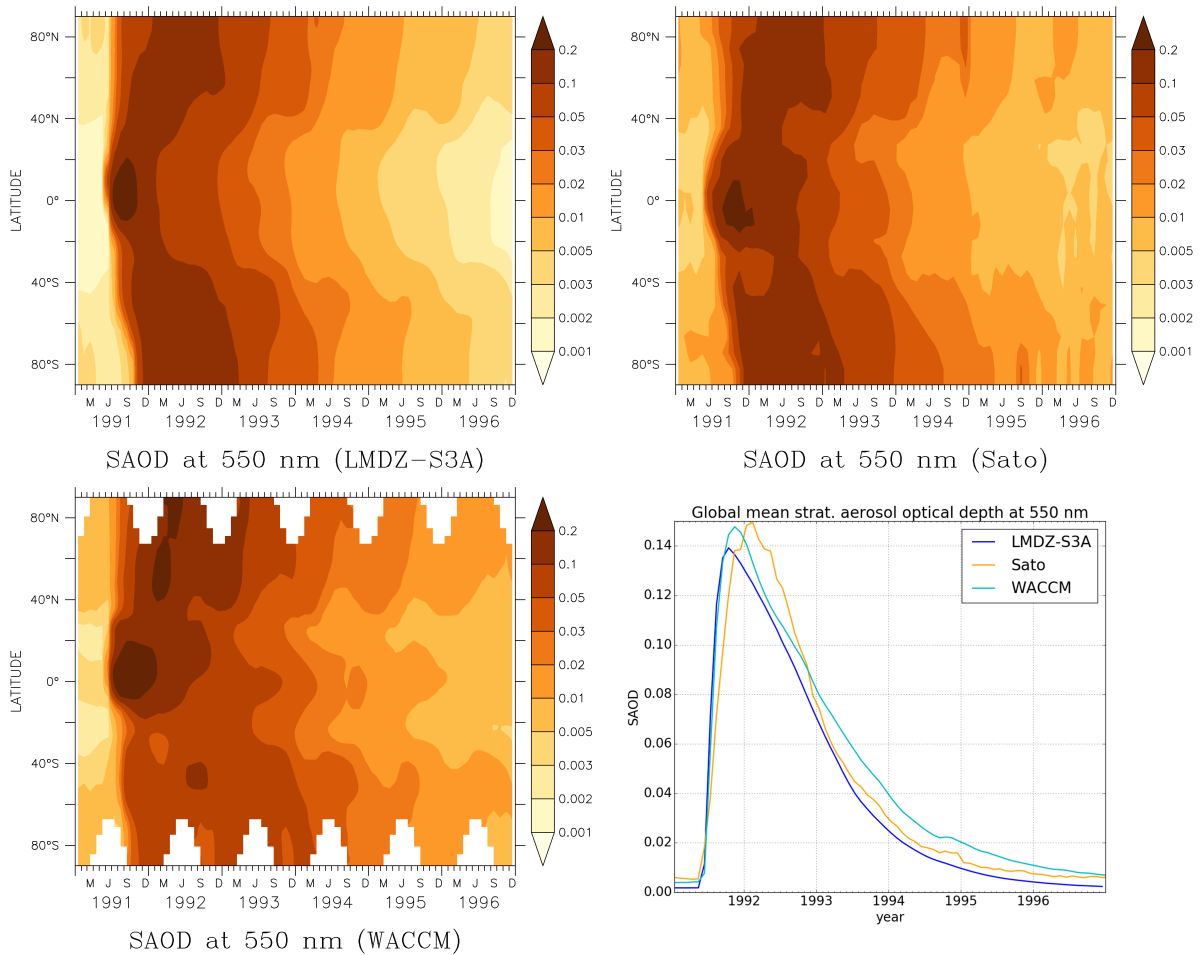
Figure 4.6: Evolution of the zonal mean stratospheric aerosol optical depth (SAOD) at 550 nm modelled with LMDZ-S3A (upper left panel) compared to the climatology from Sato [2012] (upper right panel) and to SAOD simulated with WACCM by Mills et al. [2016] (lower left panel), as well as the global mean SAOD (lower right panel). Note that unlike our simulation, WACCM includes small volcanic eruptions that occurred after that of Mount Pinatubo.
