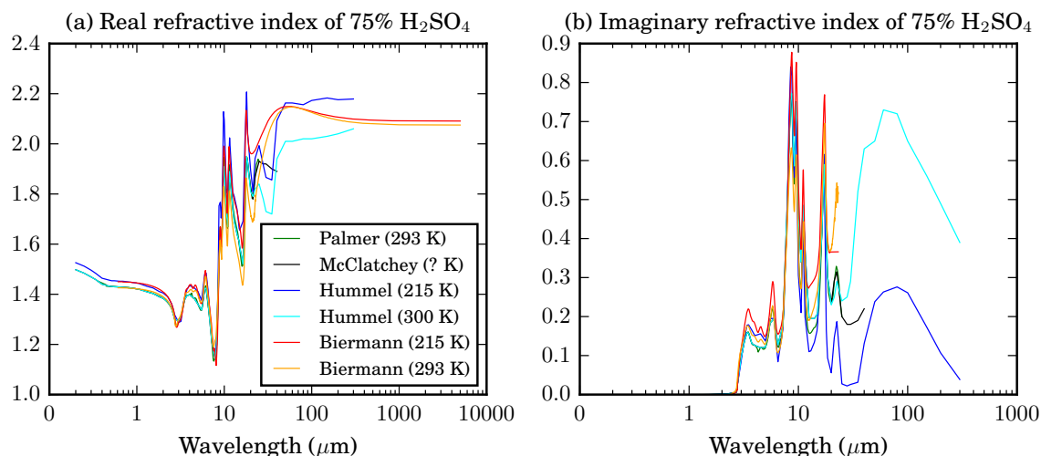
Figure 5.18: Comparison of (a) real and (b) imaginary refractive index of a 75 % H 2 SO 4 – 25 % H 2 O solution from different sources [Palmer and Williams, 1975, McClatchey et al., 1984, Hummel et al., 1988, Biermann et al., 2000].
