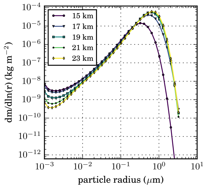
Figure 5.12: Column-integrated global and annual mean stratospheric aerosol mass size distribution ( dm/d \ln r , in \text{kg m}^{-2} ) for the z_{\text{KM}} experiments with varying injection height.
