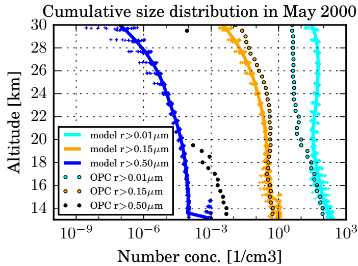
Figure 4.3: Vertical profile of the cumulative aerosol number concentration ( \text{cm}^{-3} ) for three channels ( r > 0.01 \mu\text{m} in light blue, r > 0.15 \mu\text{m} in orange, and r > 0.5 \mu\text{m} in dark blue) at Laramie, Wyoming ( 41^\circ \text{N} , 105^\circ \text{W} ) plotted in the style of Sekiya et al. [2016]. Solid lines show the modelled monthly mean, while the crosses indicate the range of daily mean concentrations within that month. Optical particle counter (OPC) measurements from Deshler et al. [2003] are shown as circles.
