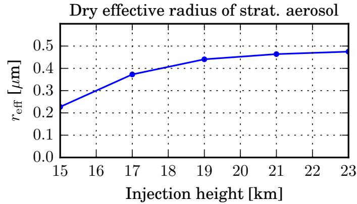
Figure 5.11: Global mean effective radius ( \mu\text{m} ) of the dry stratospheric sulphate aerosol as a function of injection height (in km) of the z_{\text{KM}} experiments.
