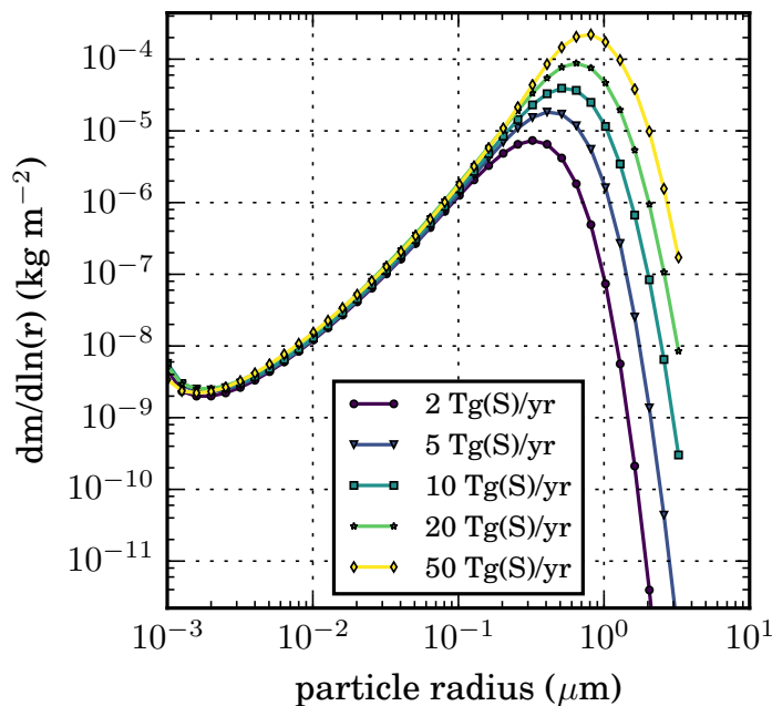
Figure 5.9: Column-integrated global and annual mean stratospheric aerosol mass size distribution ( dm/d \ln r , in \text{kg(H}_2\text{SO}_4) \text{ m}^{-2} ) for the x_{\text{TGS}} experiments with varying sulphur injection rate.
