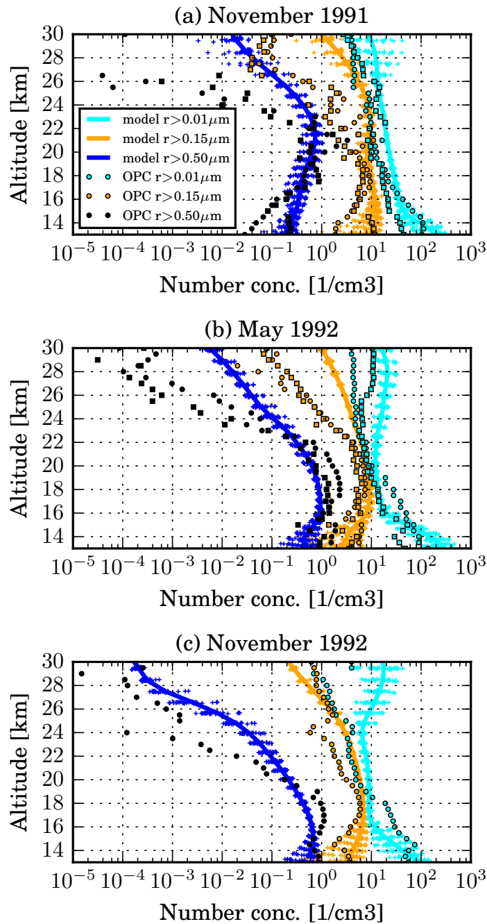
Figure 4.9: Vertical profile of the cumulative aerosol number concentration ( \text{cm}^{-3} ) for three channels ( r > 0.01 \mu\text{m} in light blue, r > 0.15 \mu\text{m} in orange, and r > 0.50 \mu\text{m} in dark blue) in November 1991, May 1992 and November 1992 at Laramie, Wyoming ( 41^\circ \text{N} , 105^\circ \text{W} ) in the style of Sekiya et al. [2016]. Solid lines show the modelled monthly mean, while the crosses indicate the range of daily mean concentrations within that month. Optical particle counter (OPC) measurements from Deshler et al. [2003] are shown as symbols.
