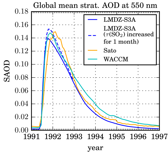
Figure 4.13: Same as Figure 4.12, but here the dashed line shows the model result for an \text{SO}_2 lifetime doubled on the day of the eruption, decreasing linearly to climatological values within one month.
