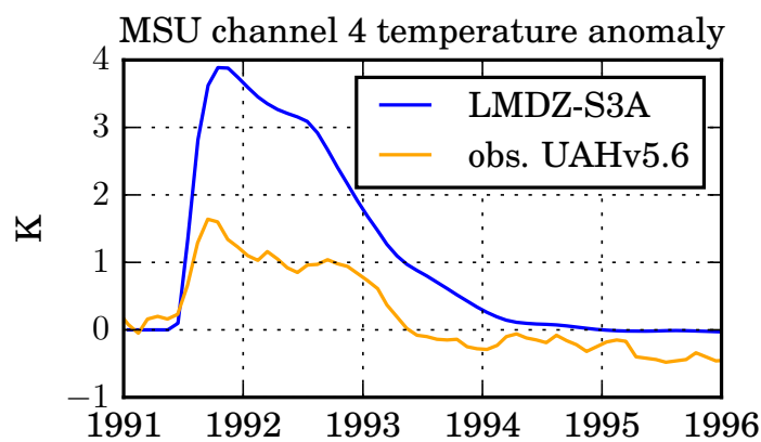
Figure 4.10: Global mean MSU channel 4 (upper tropospheric and lower stratospheric) temperature anomaly. The modelled anomaly due to the Pinatubo sulphate aerosol is computed as the difference between simulations with and without volcanic aerosol, while the observed anomaly reported by the UAH [Spencer and Christy, 1993] is with respect to the 1981–2010 base period.
