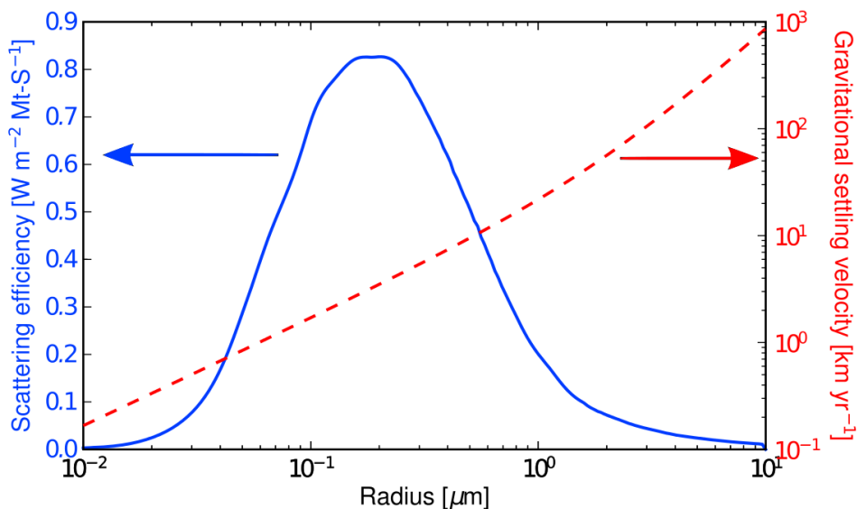
Figure 2.1: Figure extracted from Pierce et al. [2010] with the following caption: "Size dependence of factors that determine the radiative forcing of stratospheric sulphate aerosol. The blue curve and left axis show the solar-band cooling per mass (burden) of sulphate in the stratosphere as a function of aerosol size. The calculation was done assuming monodisperse aerosol and averaging over the solar spectrum. The red curve and right axis show the gravitational settling velocity at a height of 25 km."
