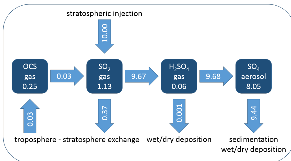
Figure 5.1: Annual mean stratospheric burdens (boxes, in Tg S) and fluxes (arrows, in Tg S yr -1 ) of the represented sulphur species from the 5 th year (quasi-steady state) of the STANDARD experiment. Minor discrepancies in the fluxes indicate that the steady state is not entirely reached after 5 years.
