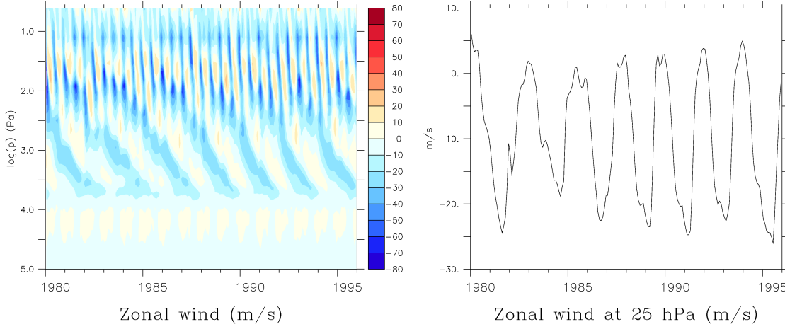
Figure 3.1: Left panel: Altitude-time profile of the zonal wind (in \text{m s}^{-1} ), averaged between 10^\circ \text{ S} and 10^\circ \text{ N} , from an LMDZ-S3A simulation with evolving background aerosol. The vertical axis shows the logarithm of the pressure in Pa. Right panel: Zonal wind at 25 hPa, averaged between 10^\circ \text{ S} and 10^\circ \text{ N} .
