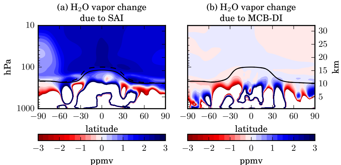
Figure 6.2: Same as Figure 6.1 but for the absolute change in stratospheric water vapour (ppmv). White areas correspond to tropospheric changes that are larger than spanned by the color scale.
